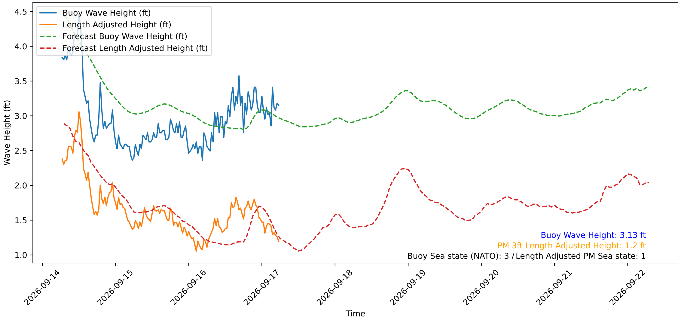
Wave Heights over Time for Oceanside Harbor at 2026-09-17 06:30:29
