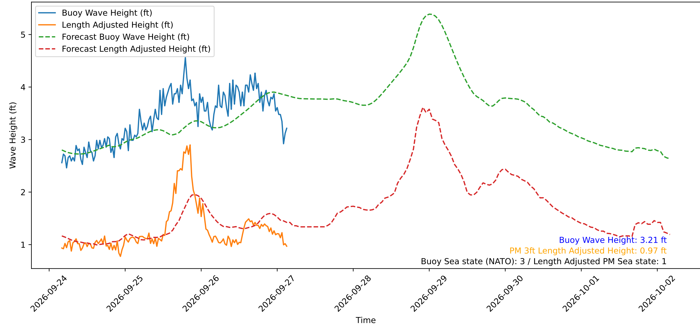
Wave Heights over Time for Green Beach at 2026-09-27 03:41:12
