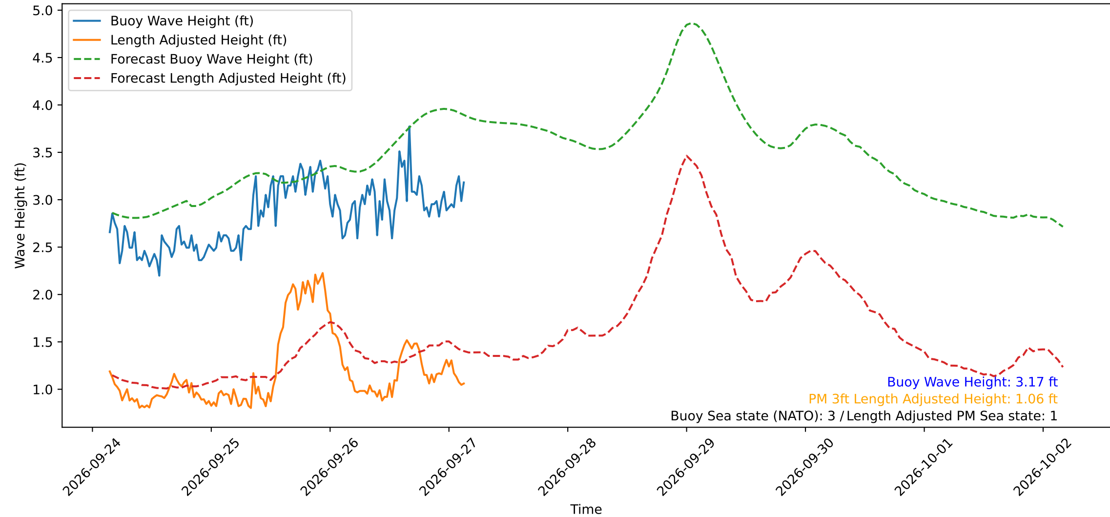
Wave Heights over Time for Oceanside Harbor at 2026-09-27 03:40:30
