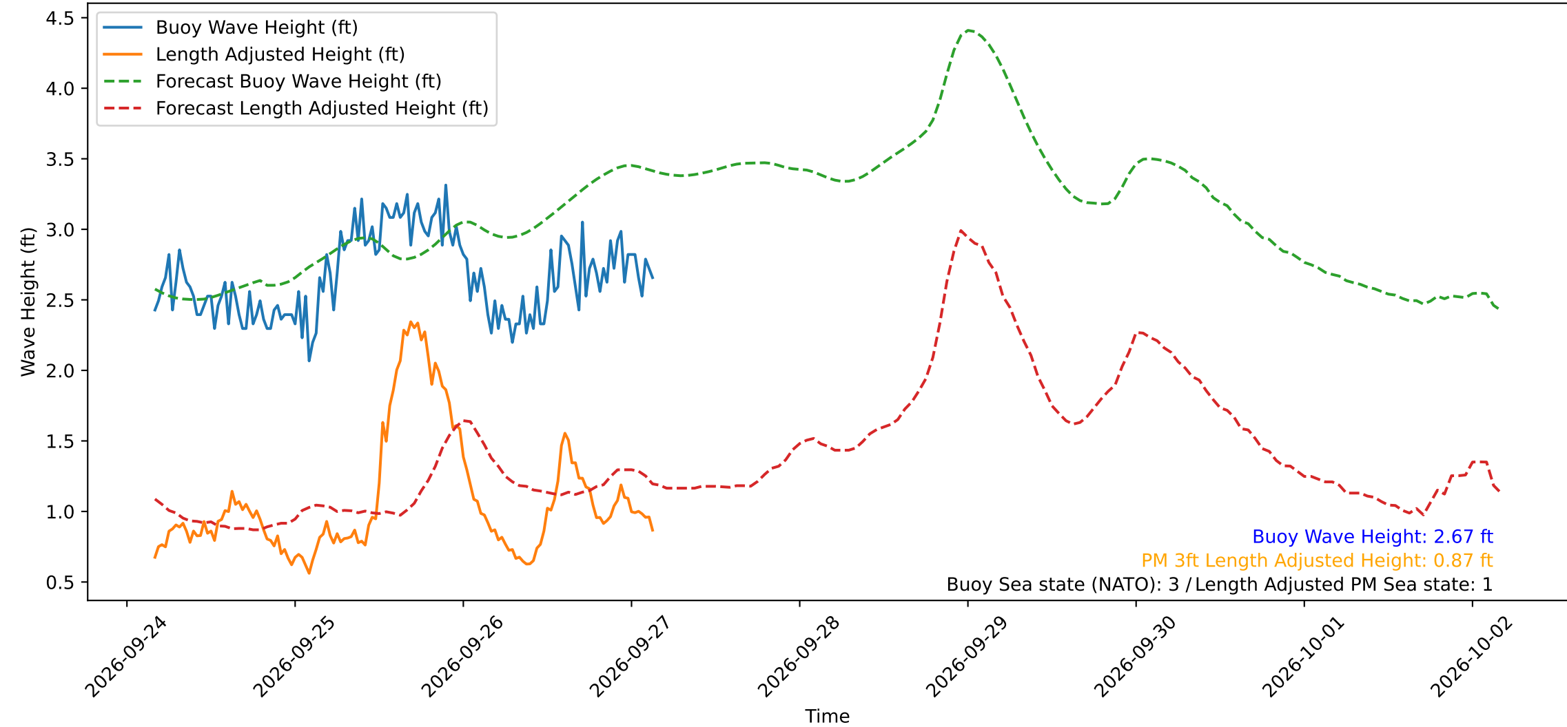
Wave Heights over Time for Red Beach at 2026-09-27 03:40:50
