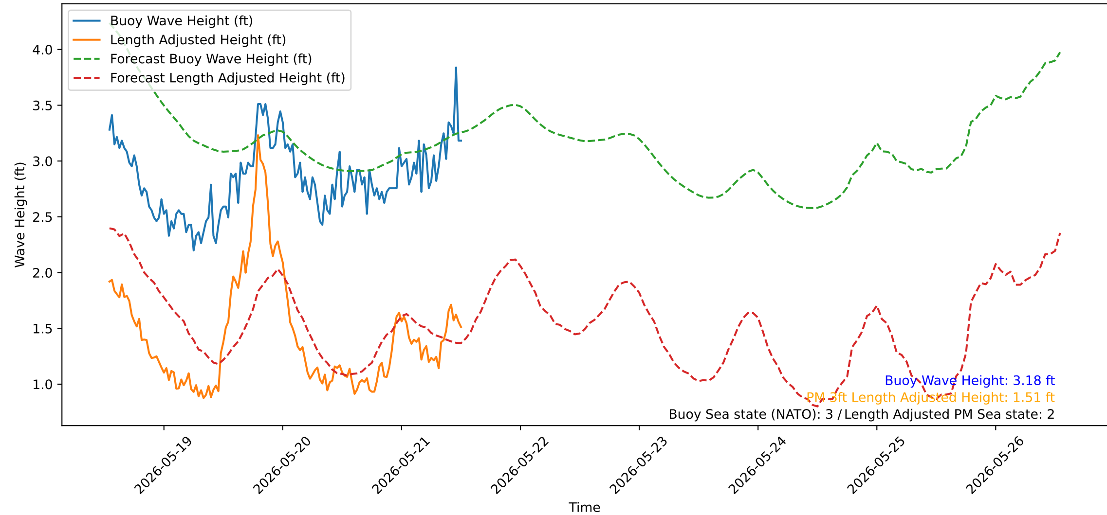
Wave Heights over Time for Oceanside Harbor at 2026-05-21 12:50:31
