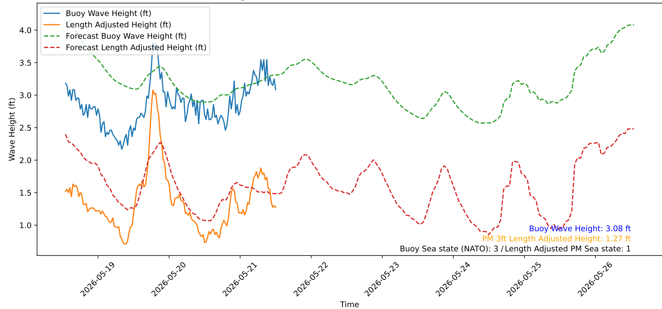
Wave Heights over Time for Green Beach at 2026-05-21 12:51:15
