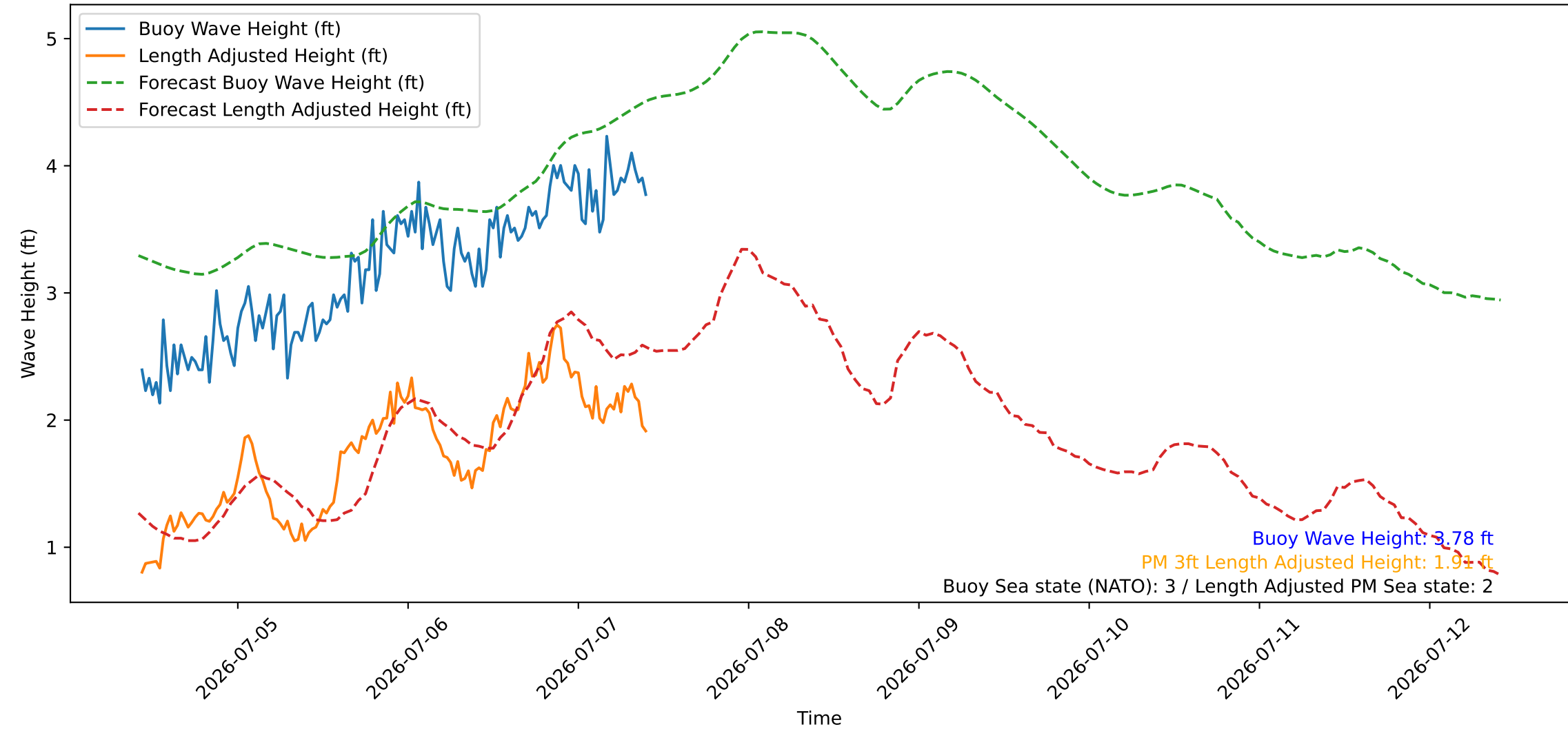
Wave Heights over Time for Oceanside Harbor at 2026-07-07 10:20:26
