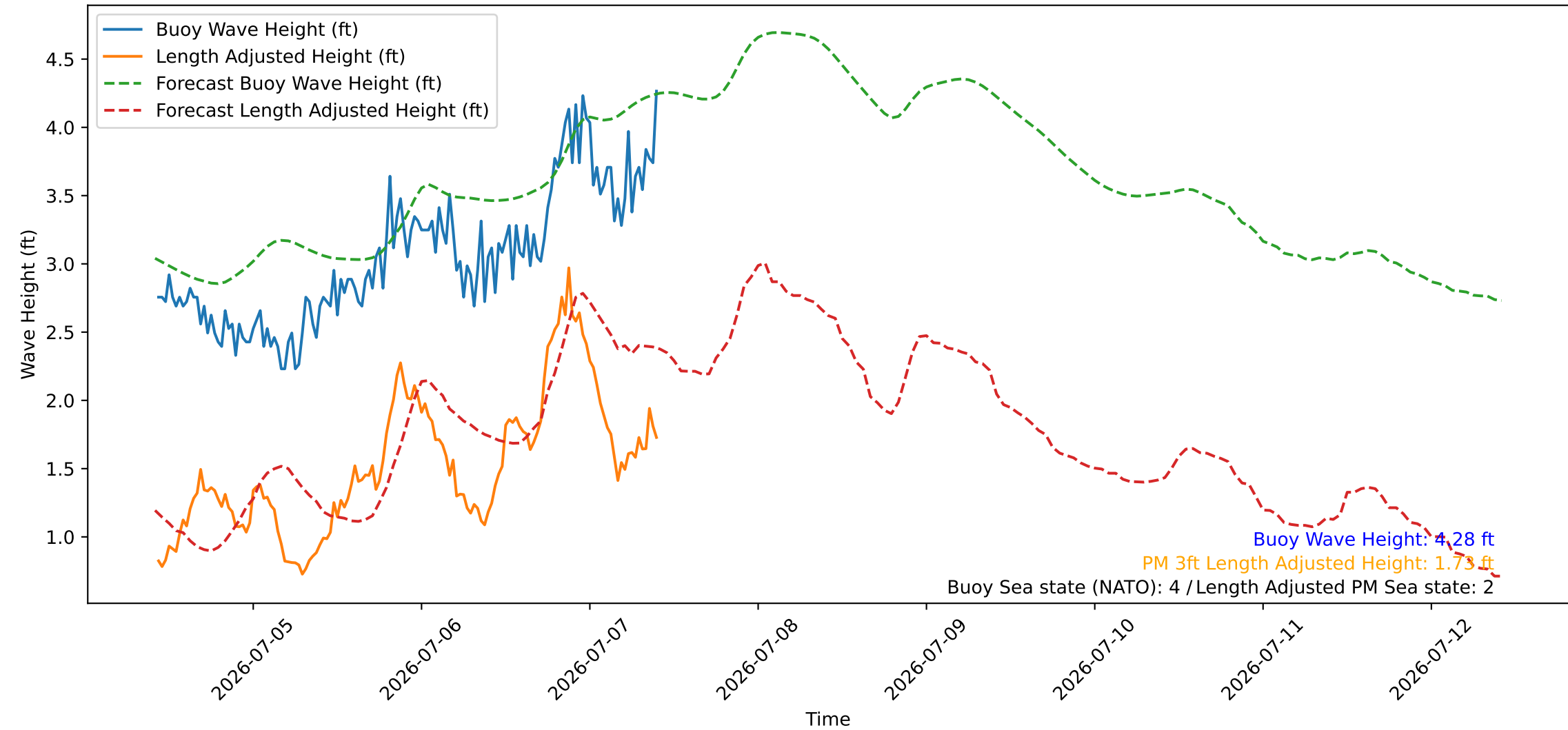
Wave Heights over Time for Red Beach at 2026-07-07 10:20:48
