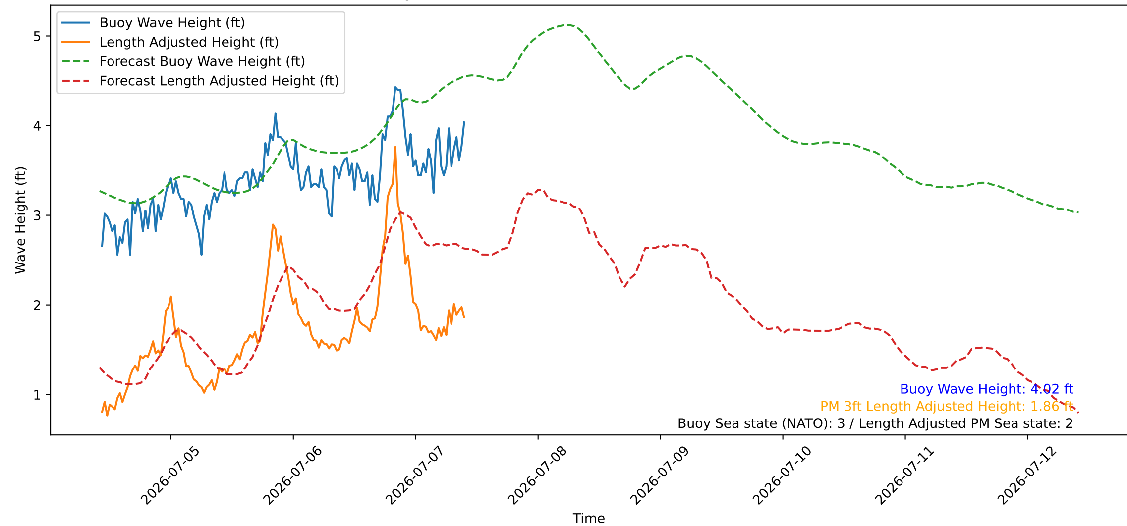
Wave Heights over Time for Green Beach at 2026-07-07 10:21:10
