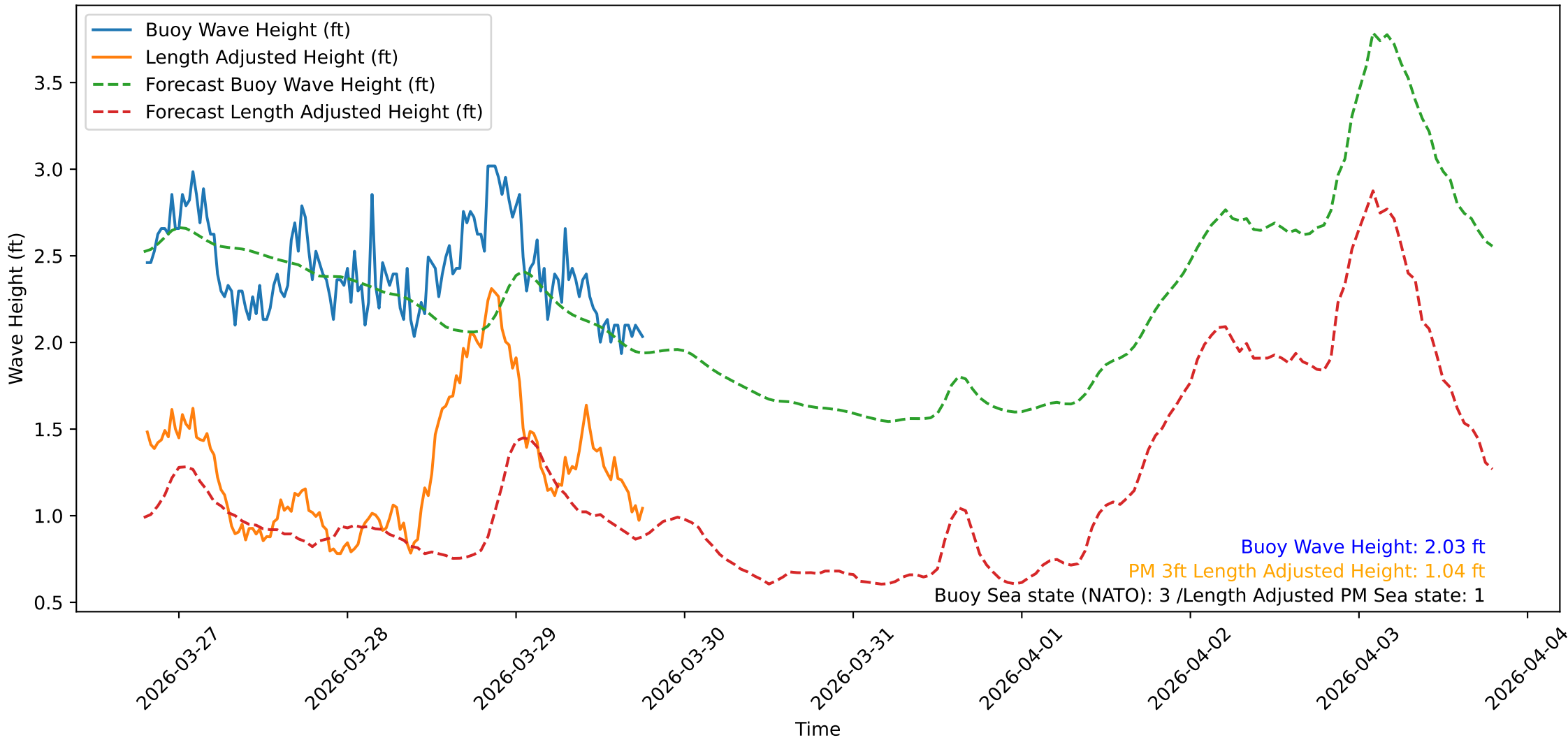
Wave Heights over Time for Red Beach at 2026-03-29 19:00:47
