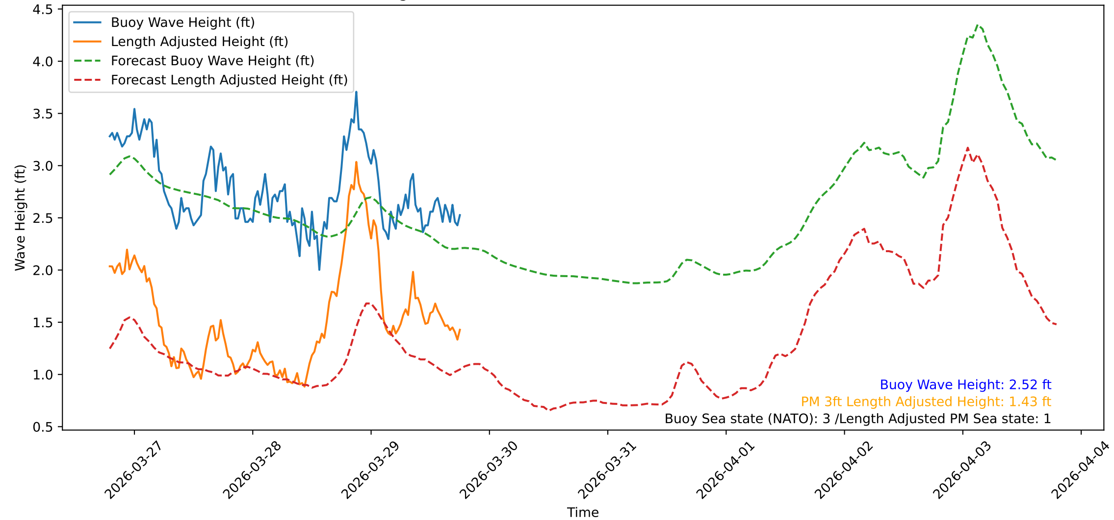
Wave Heights over Time for Green Beach at 2026-03-29 19:01:09
