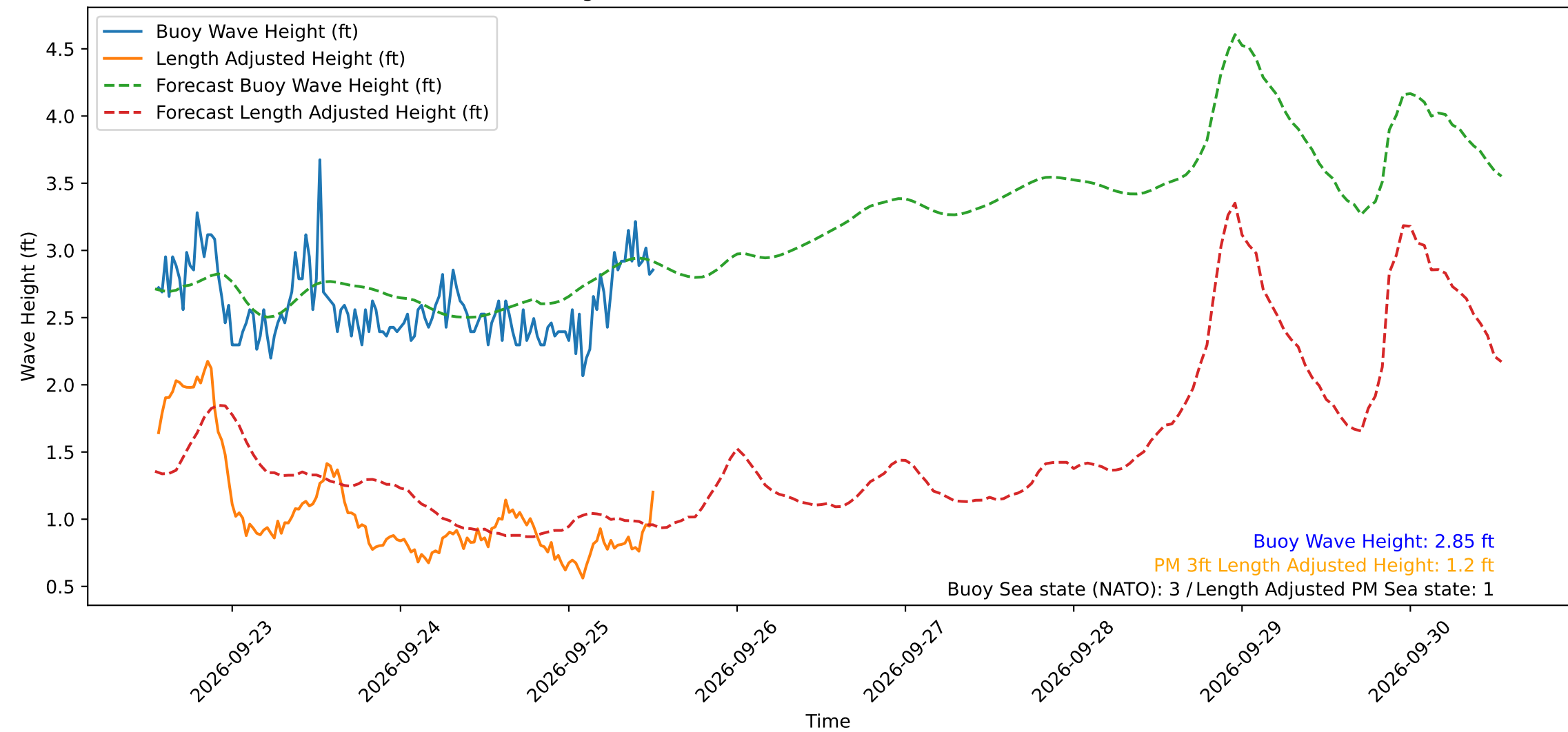
Wave Heights over Time for Red Beach at 2026-09-25 13:10:48
