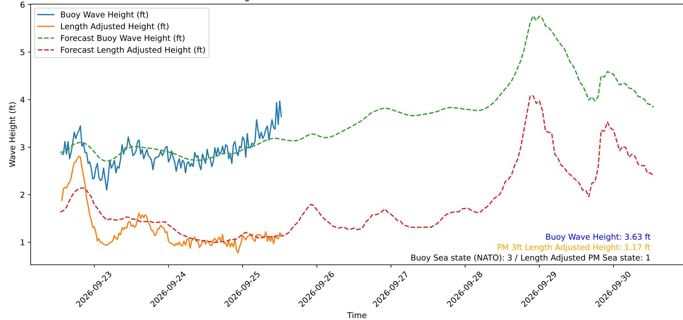
Wave Heights over Time for Green Beach at 2026-09-25 13:11:11
