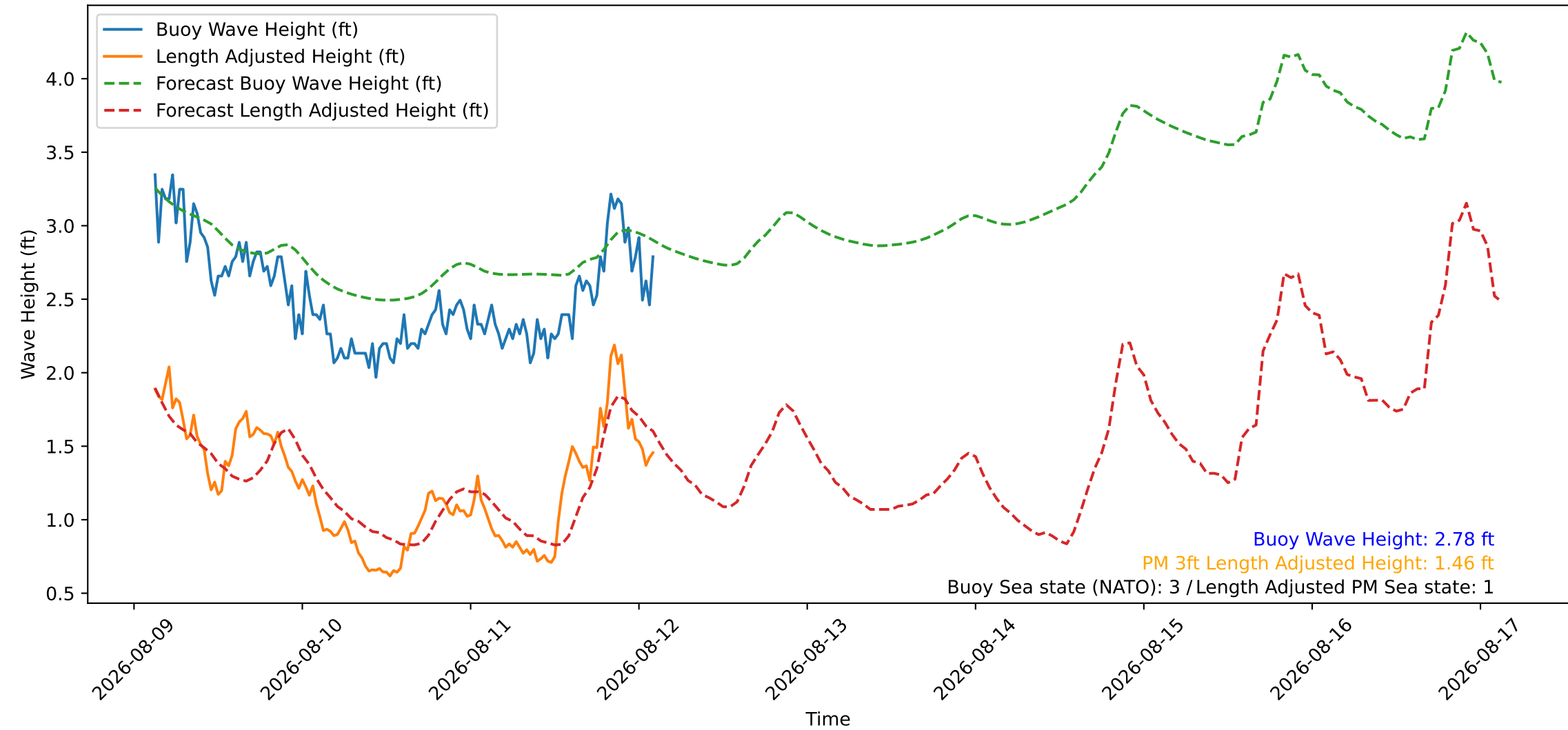
Wave Heights over Time for Green Beach at 2026-08-12 02:51:09
