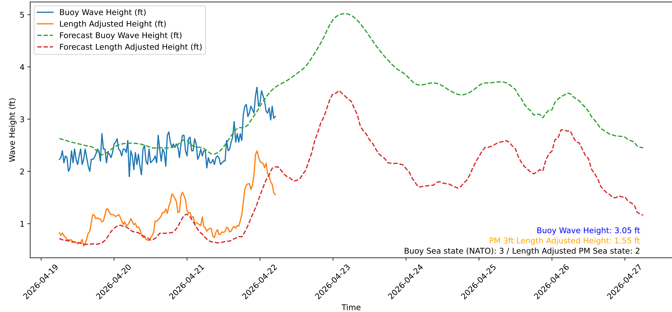
Wave Heights over Time for Oceanside Harbor at 2026-04-22 06:00:31
