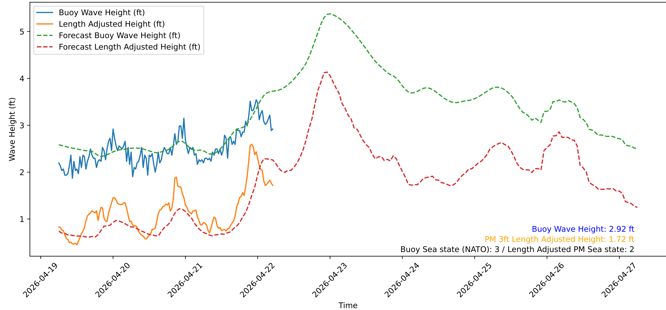
Wave Heights over Time for Green Beach at 2026-04-22 06:01:12
