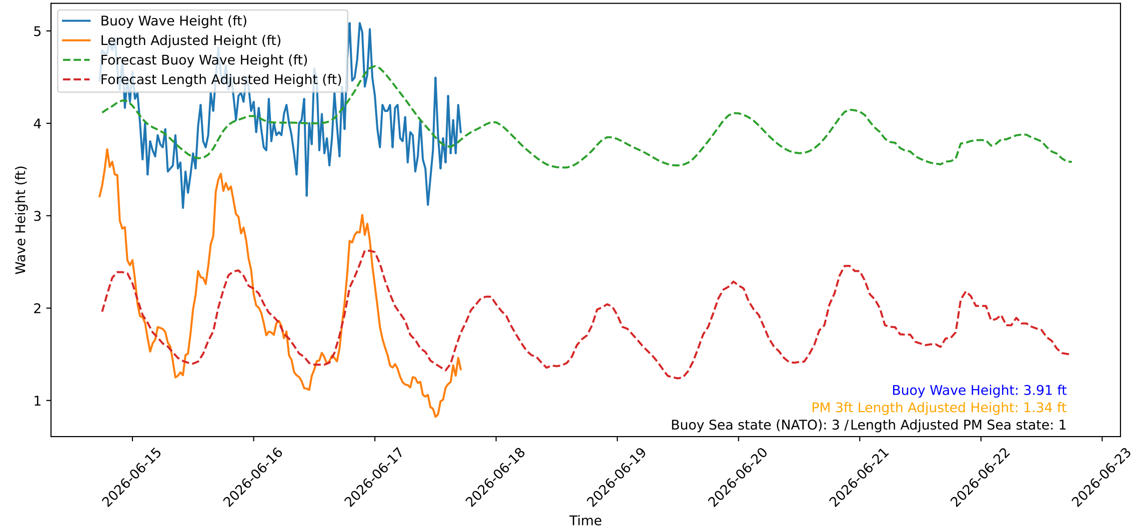
Wave Heights over Time for Green Beach at 2026-06-17 17:41:10
