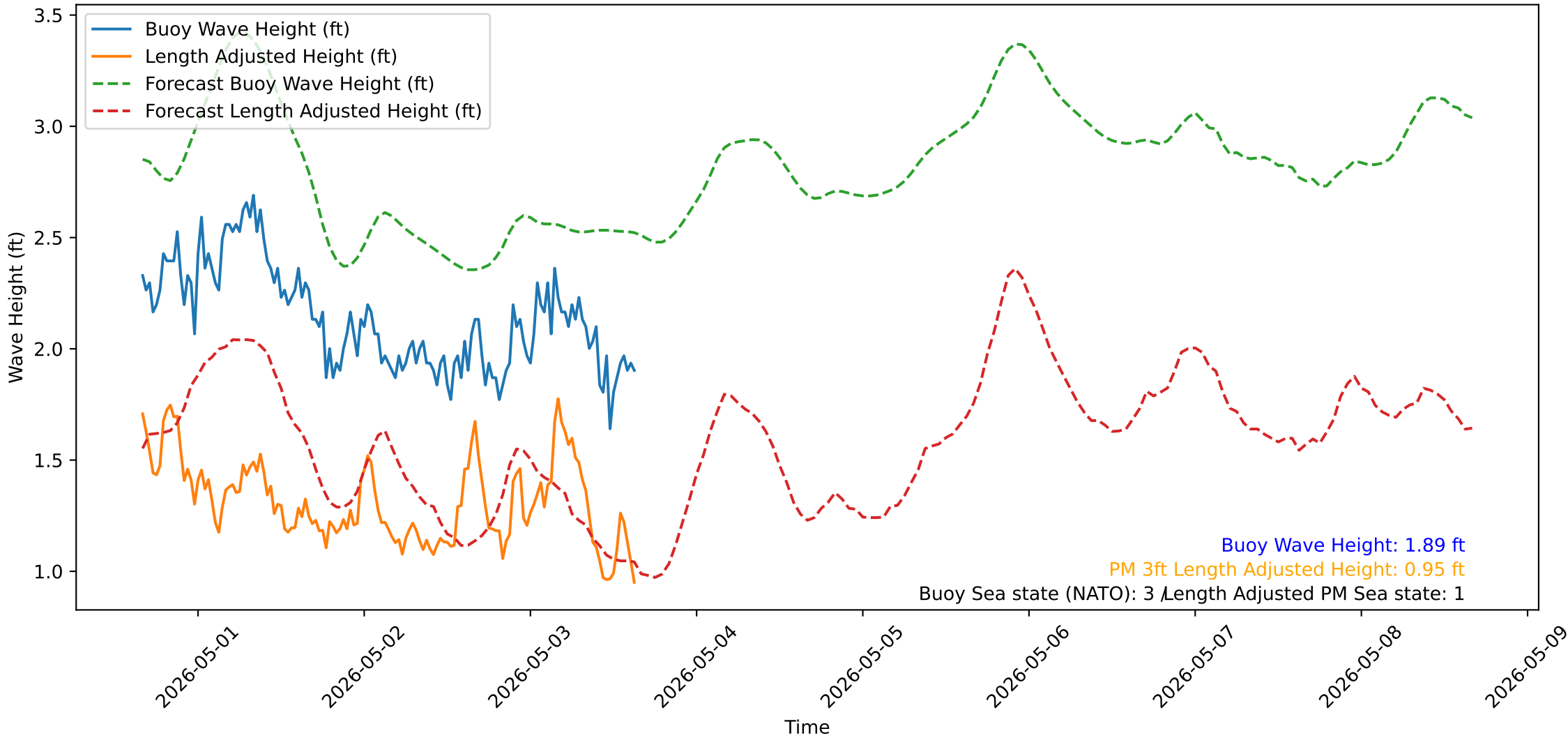
Wave Heights over Time for Oceanside Harbor at 2026-05-03 15:50:31
