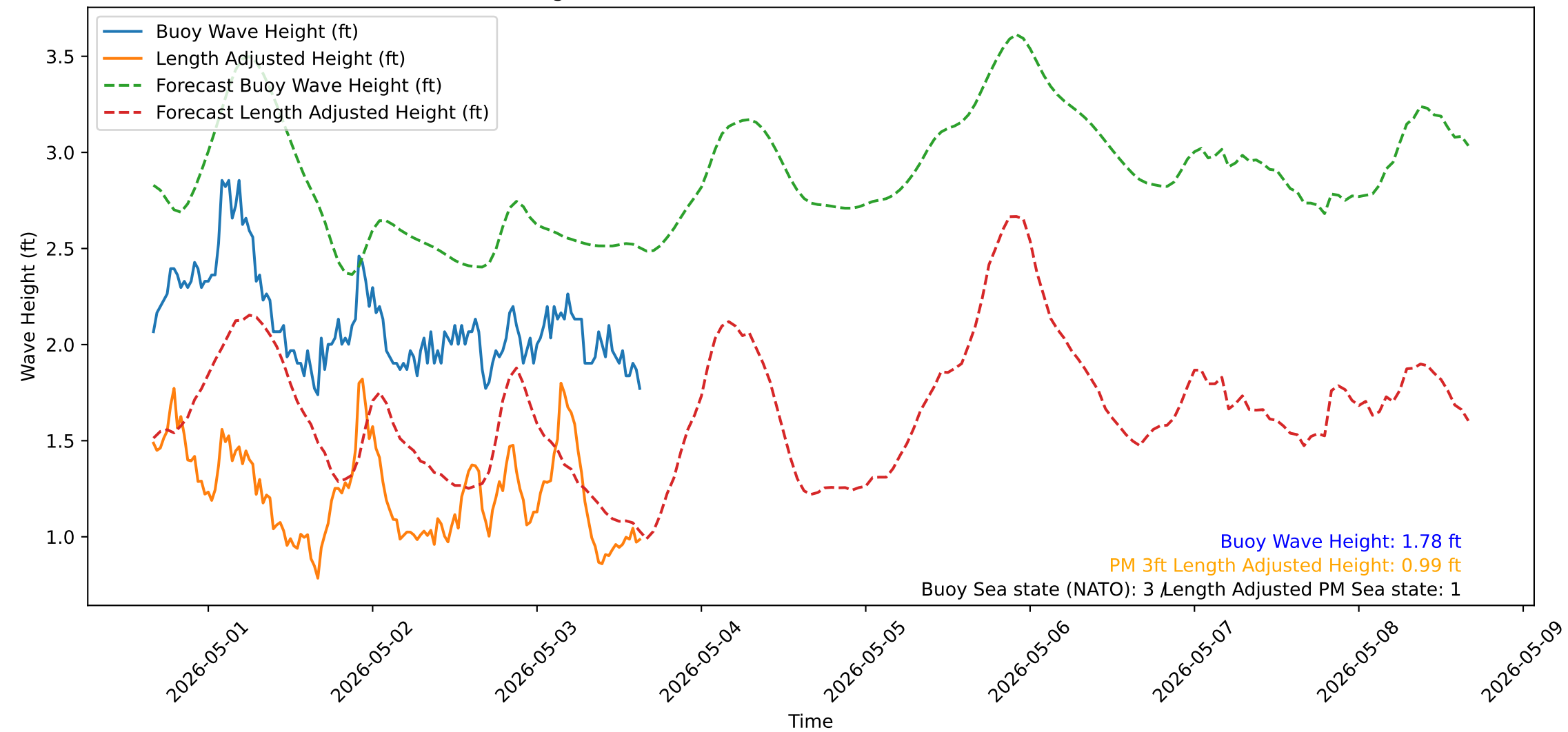
Wave Heights over Time for Green Beach at 2026-05-03 15:51:13
