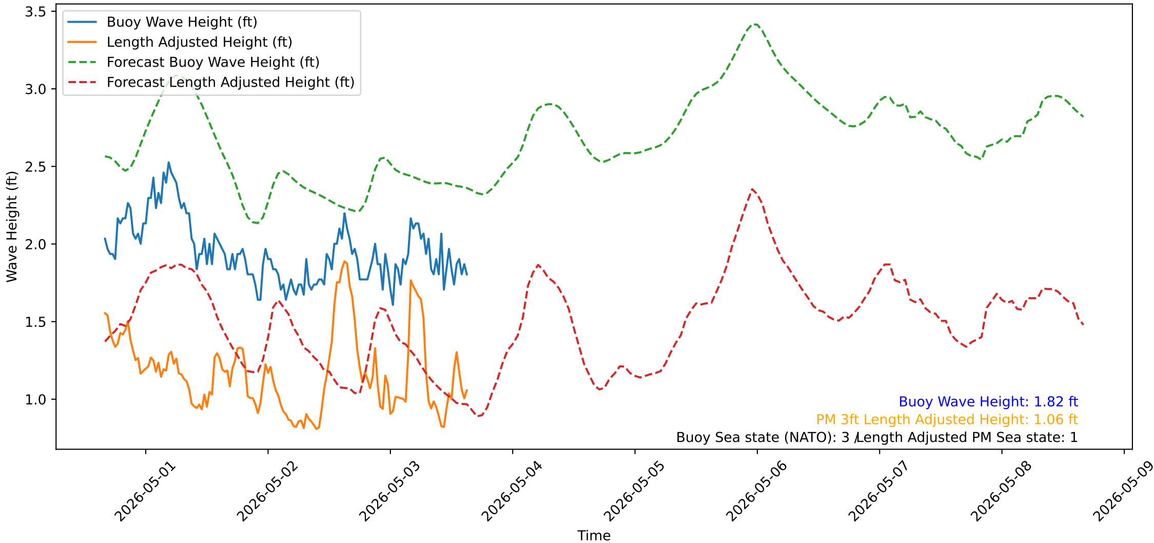
Wave Heights over Time for Red Beach at 2026-05-03 15:50:51
