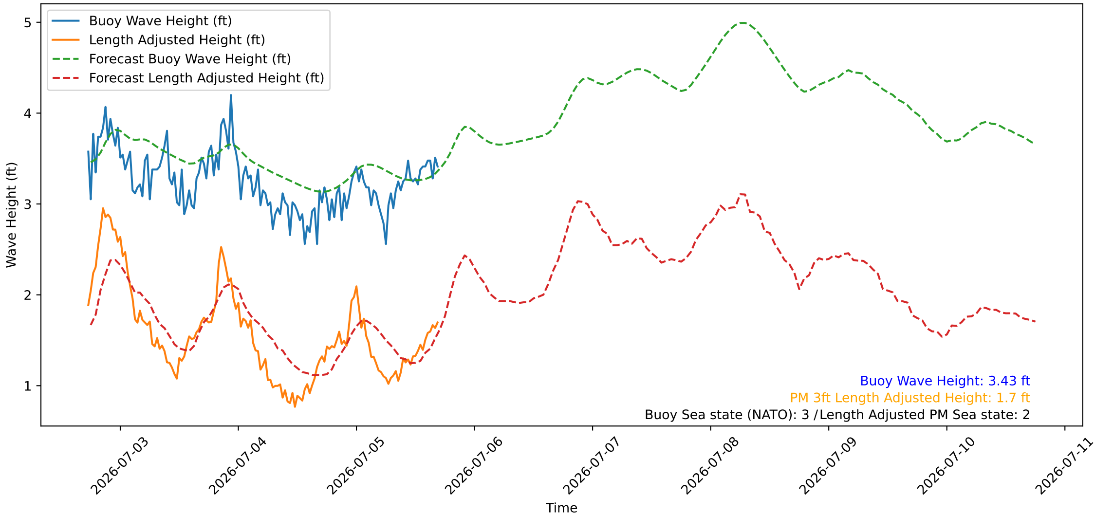
Wave Heights over Time for Green Beach at 2026-07-05 17:31:09
