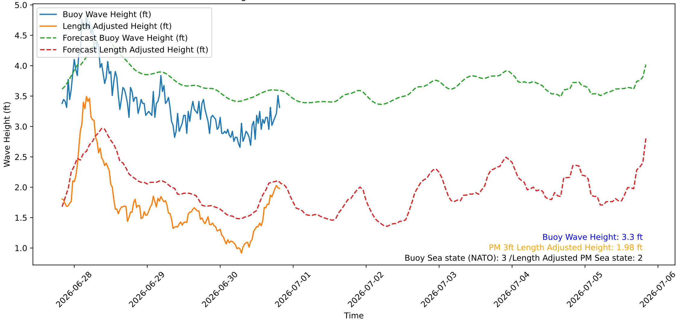
Wave Heights over Time for Green Beach at 2026-06-30 20:11:08
