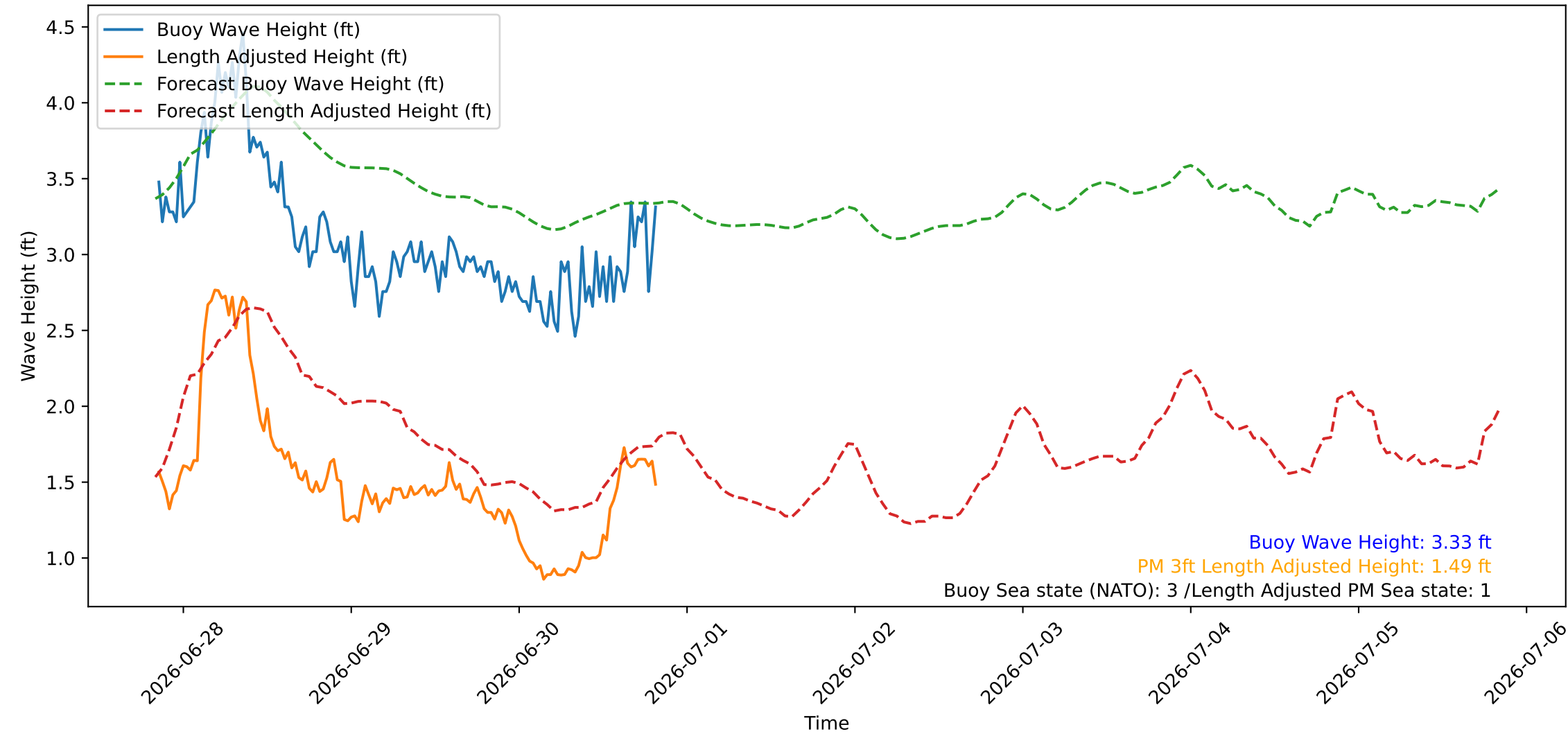
Wave Heights over Time for Red Beach at 2026-06-30 20:10:45
