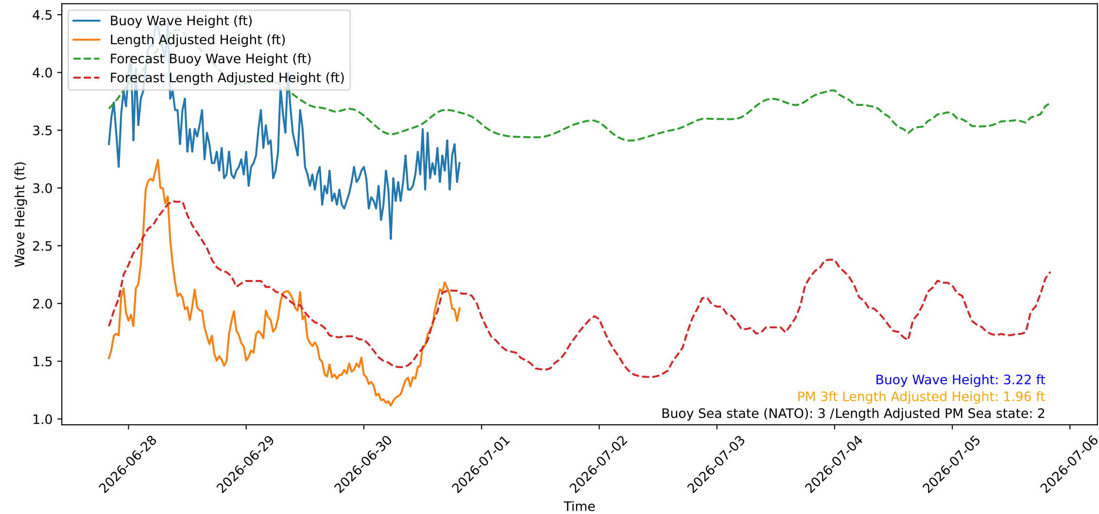
Wave Heights over Time for Oceanside Harbor at 2026-06-30 20:10:26
