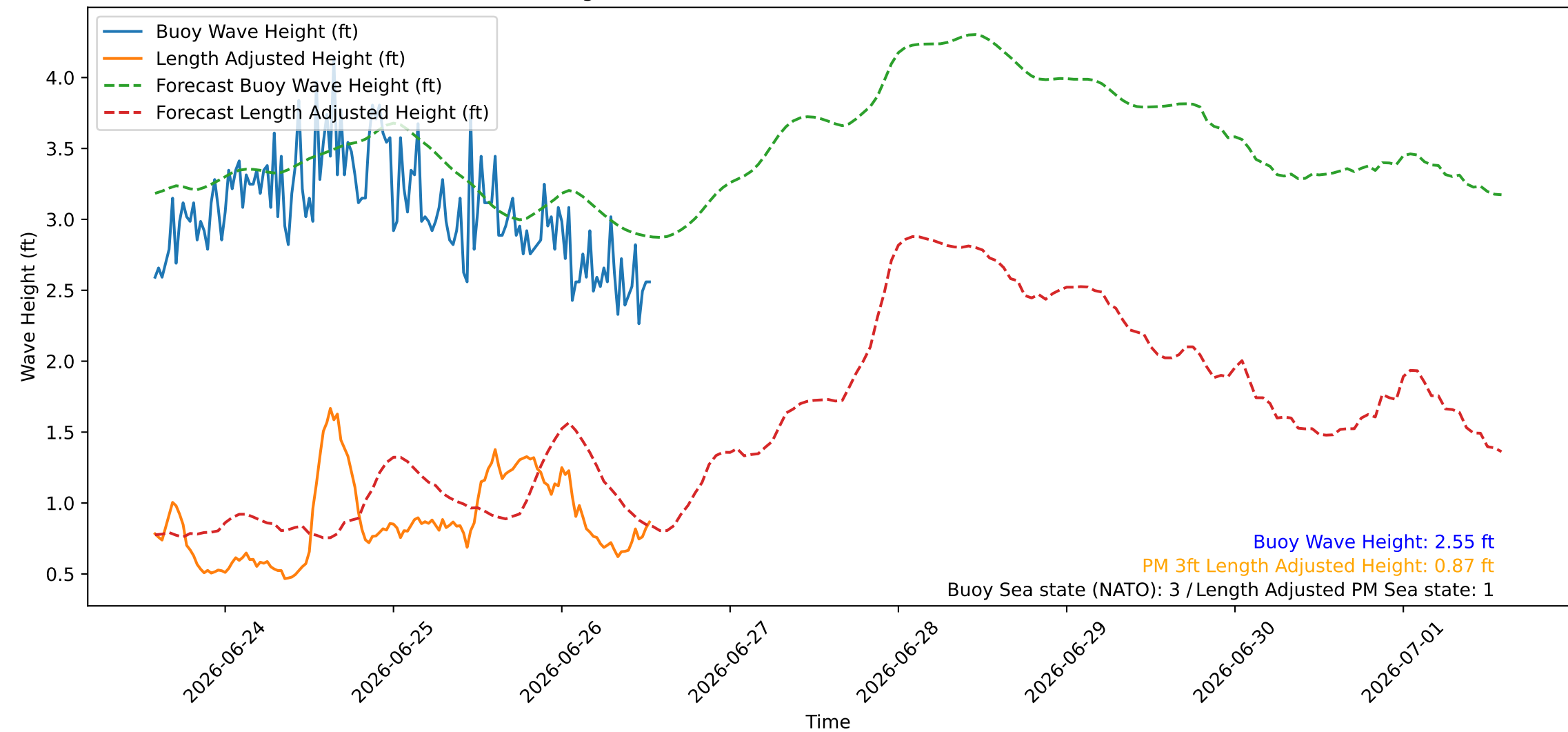
Wave Heights over Time for Red Beach at 2026-06-26 13:40:46
