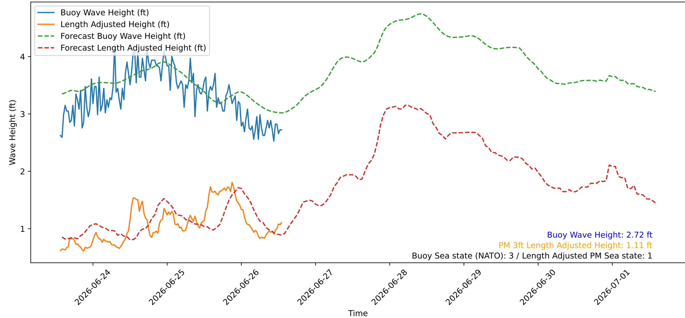
Wave Heights over Time for Green Beach at 2026-06-26 13:41:08
