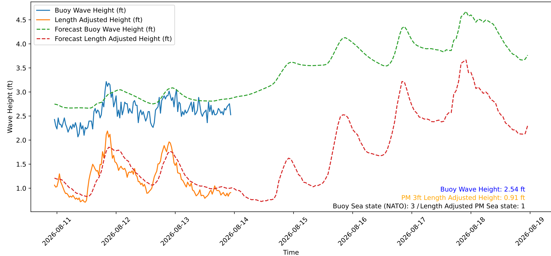
Wave Heights over Time for Green Beach at 2026-08-13 23:11:08
