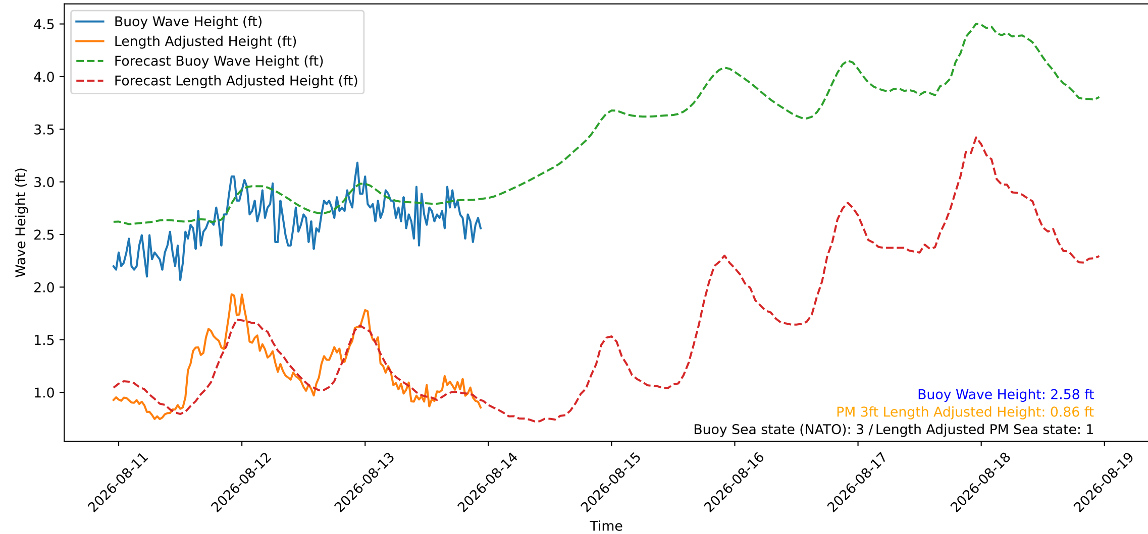
Wave Heights over Time for Oceanside Harbor at 2026-08-13 23:10:27
