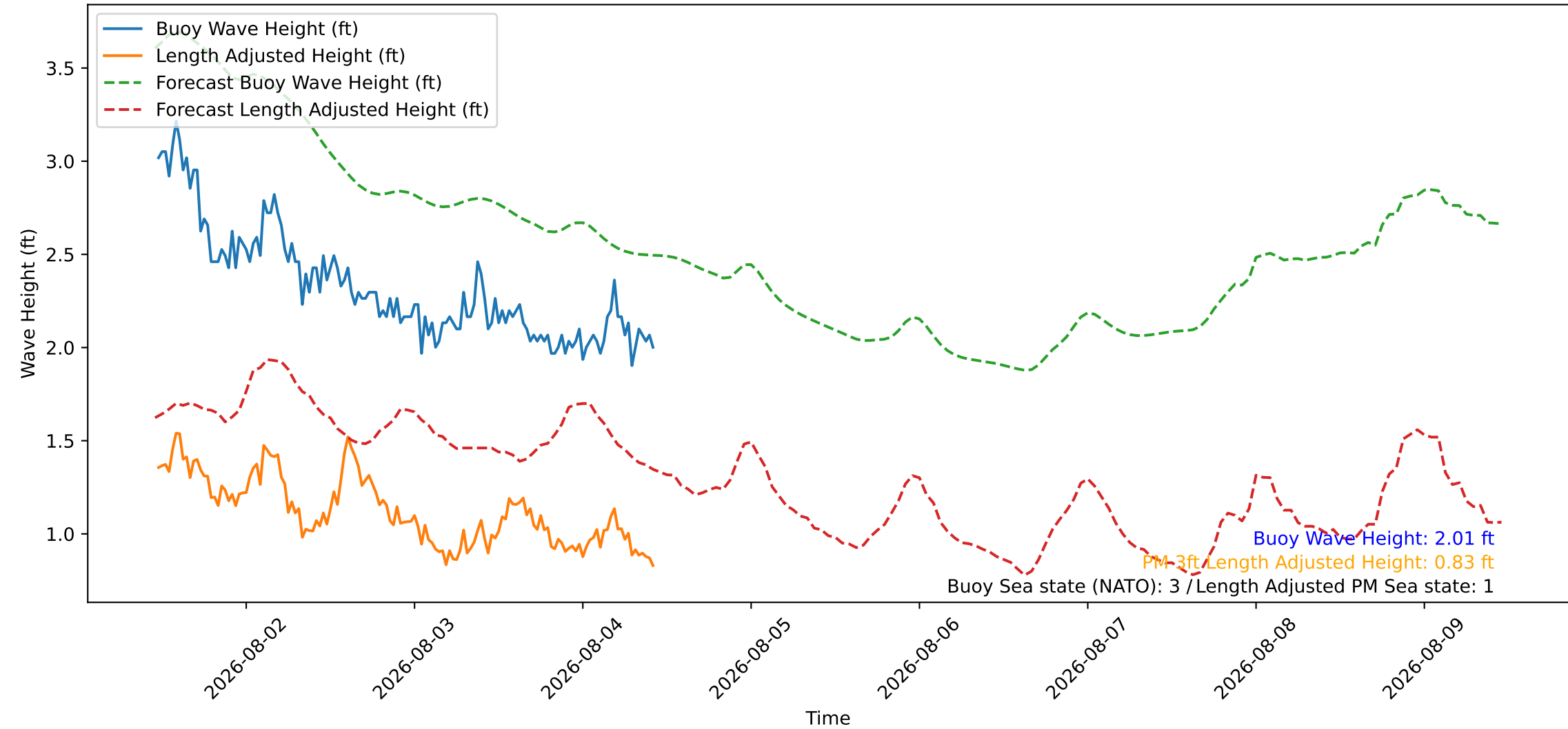
Wave Heights over Time for Red Beach at 2026-08-04 11:00:46
