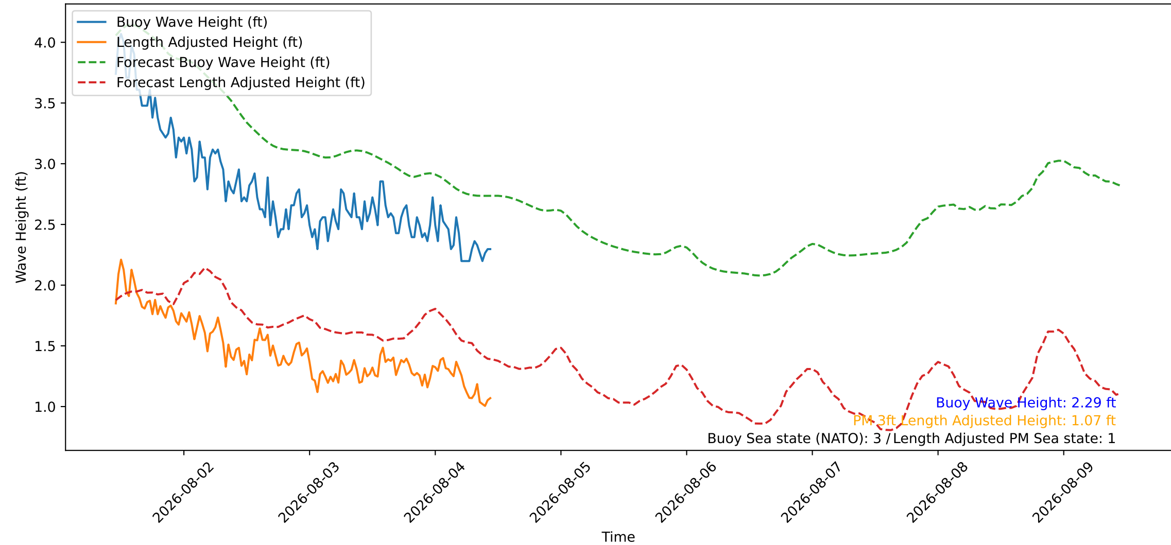
Wave Heights over Time for Oceanside Harbor at 2026-08-04 11:00:26
