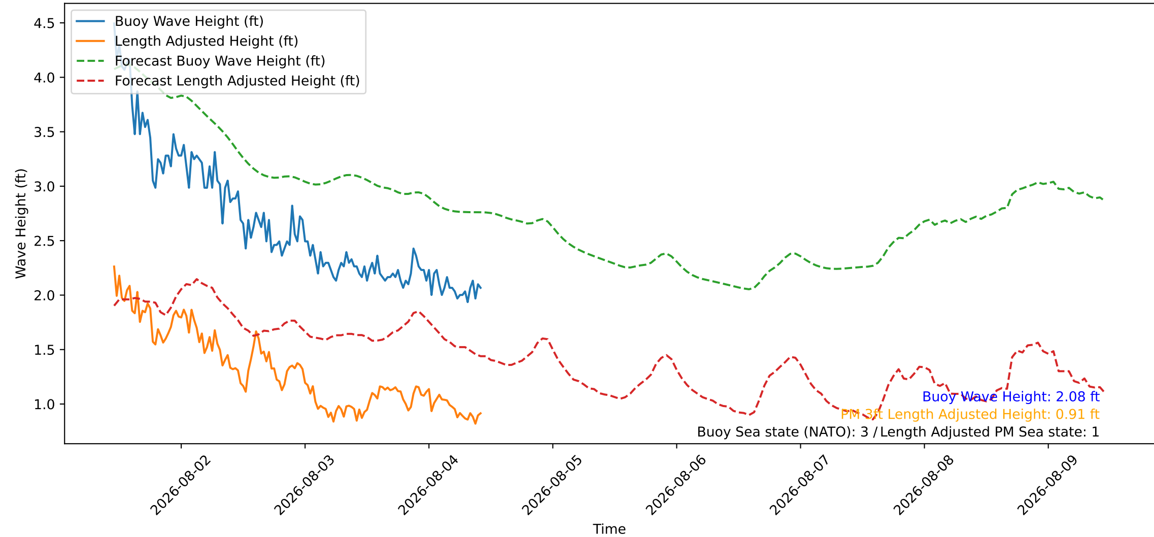
Wave Heights over Time for Green Beach at 2026-08-04 11:01:08
