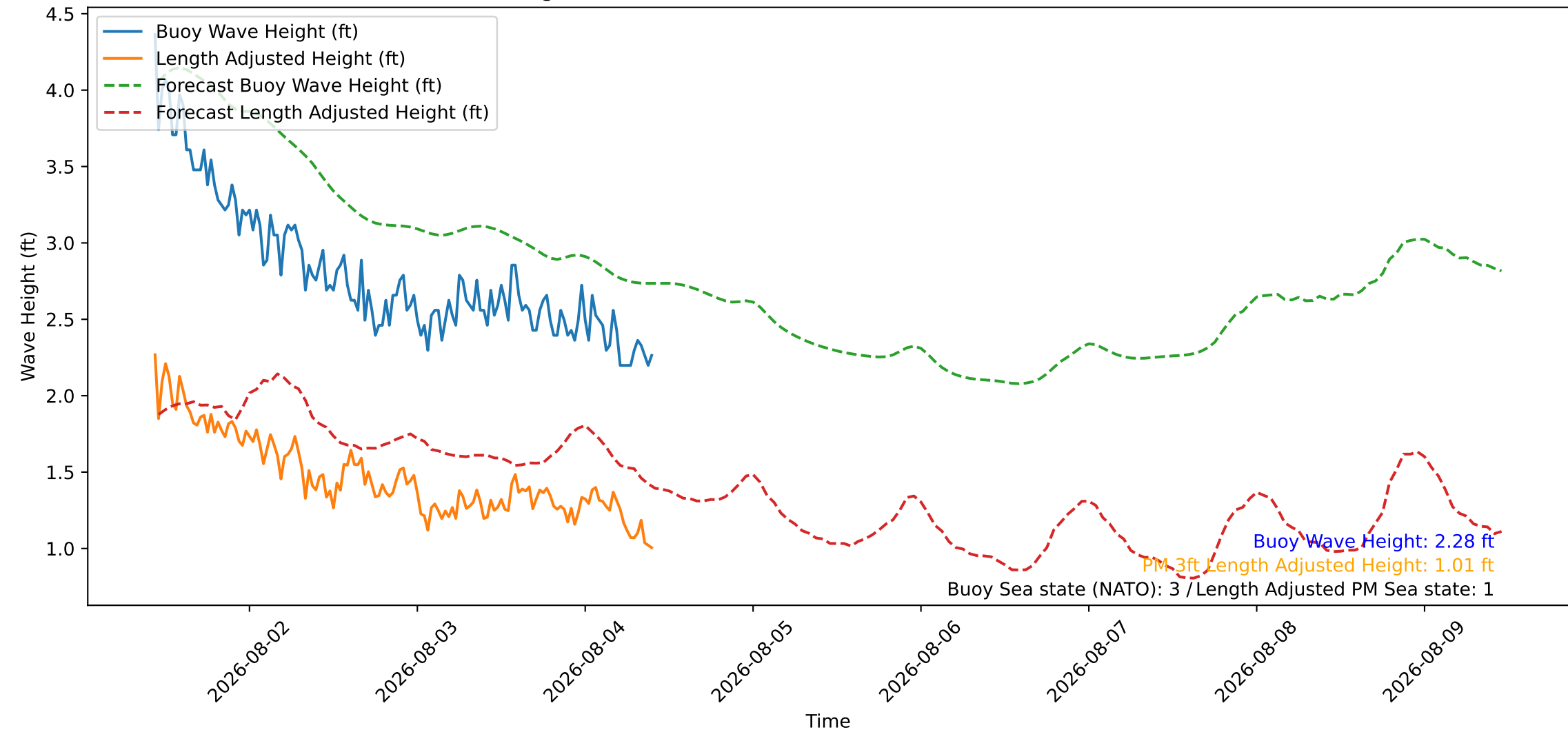
Wave Heights over Time for Oceanside Harbor at 2026-08-04 10:30:26
