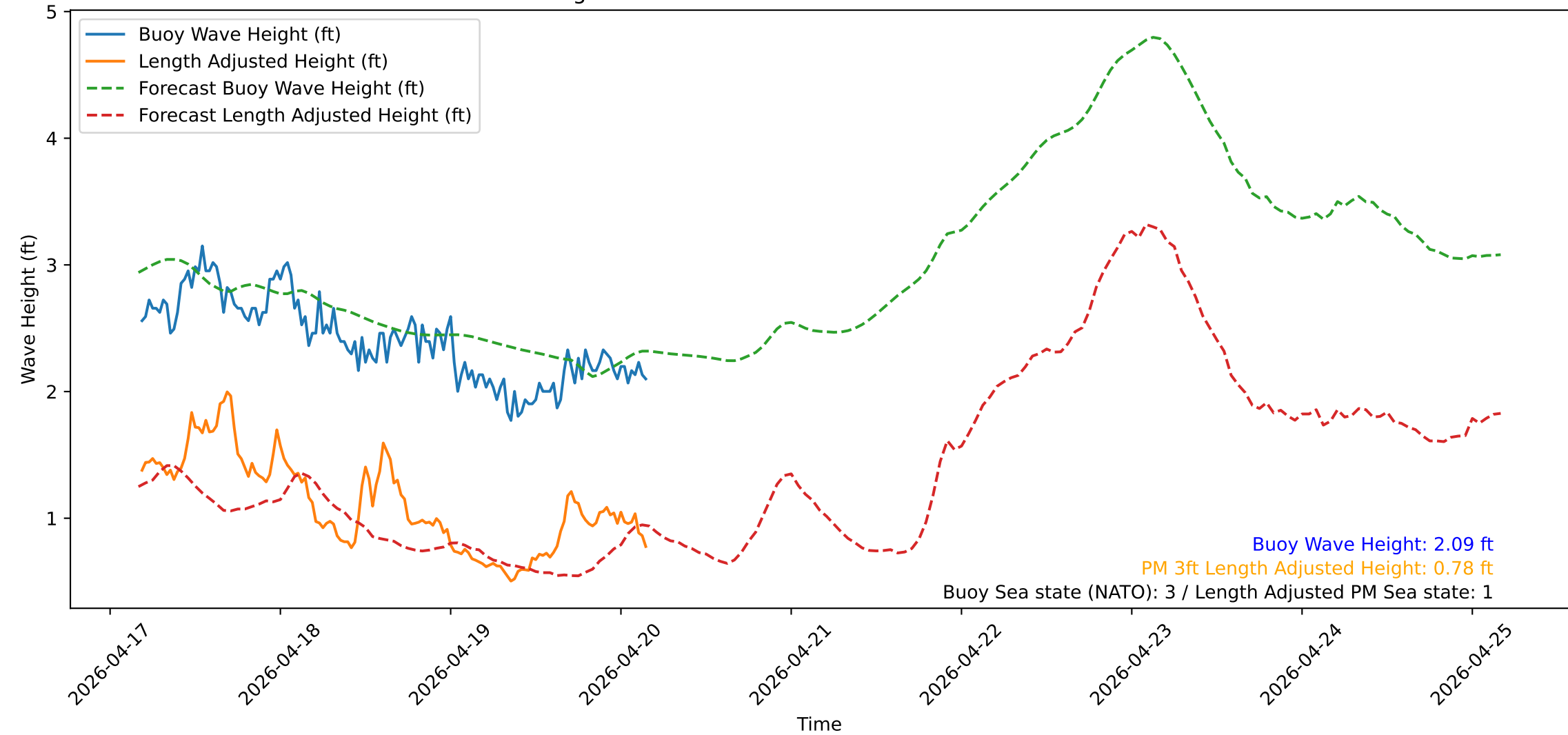
Wave Heights over Time for Red Beach at 2026-04-20 04:20:51
