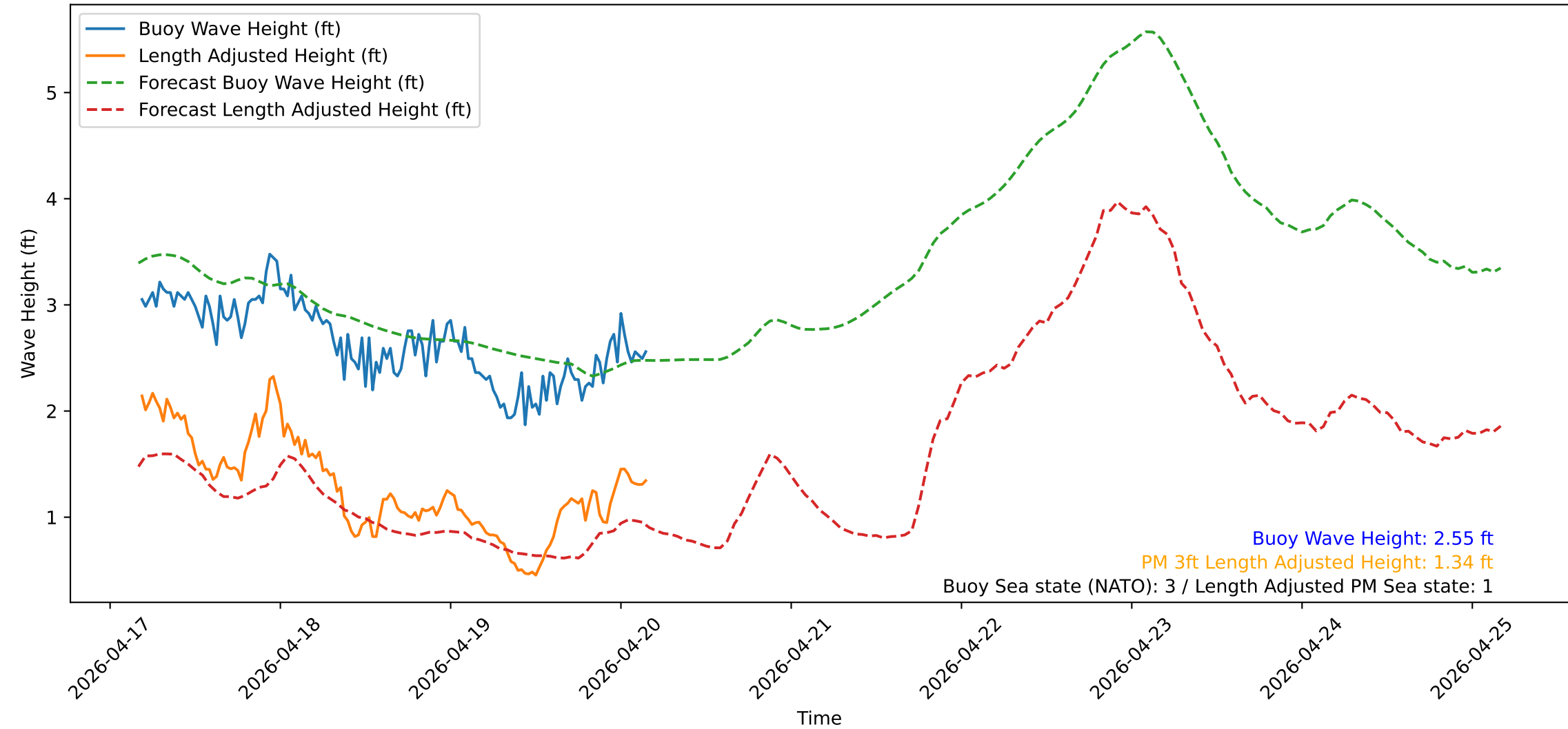
Wave Heights over Time for Green Beach at 2026-04-20 04:21:14
