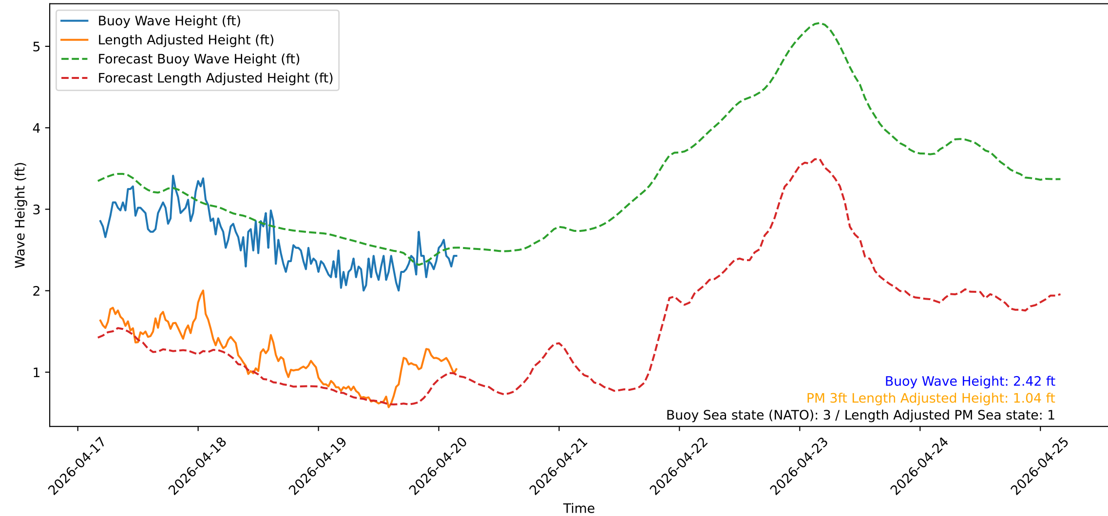
Wave Heights over Time for Oceanside Harbor at 2026-04-20 04:20:31
