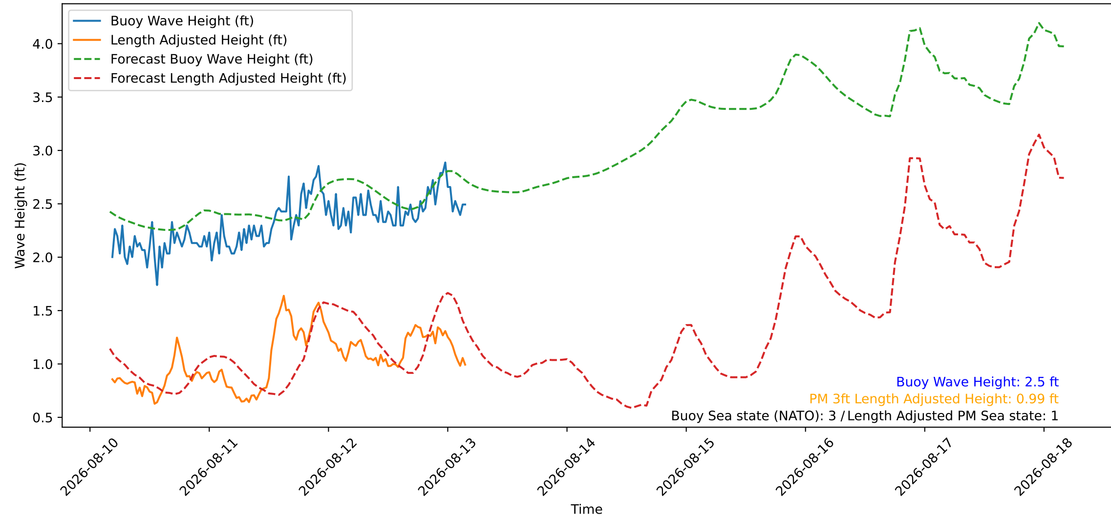
Wave Heights over Time for Red Beach at 2026-08-13 04:20:48
