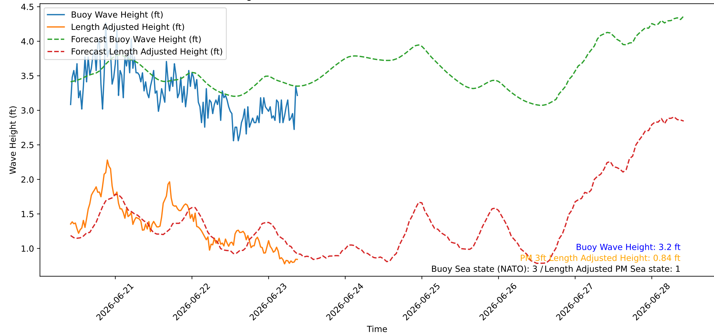
Wave Heights over Time for Oceanside Harbor at 2026-06-23 10:00:26
