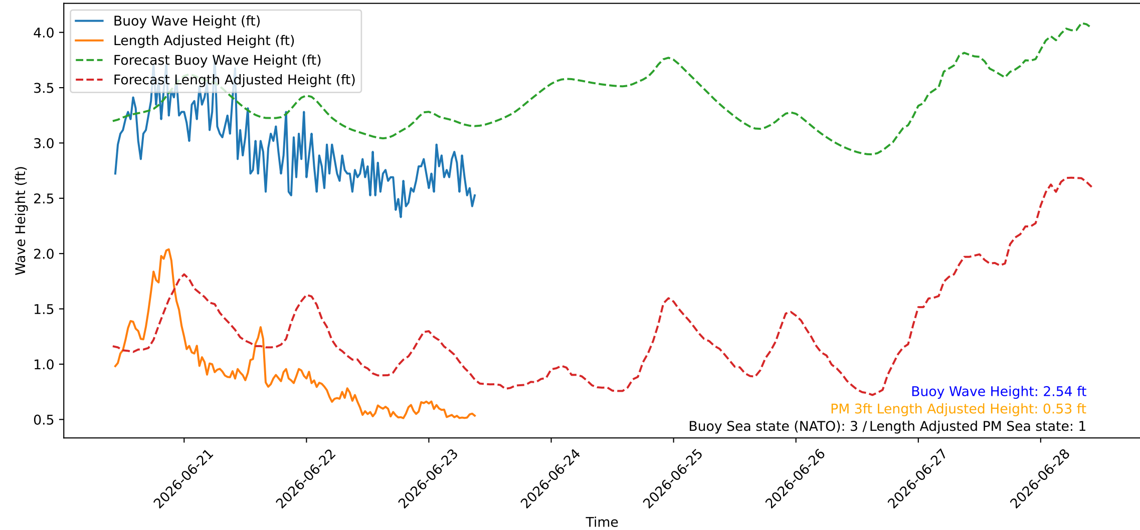
Wave Heights over Time for Red Beach at 2026-06-23 10:00:45
