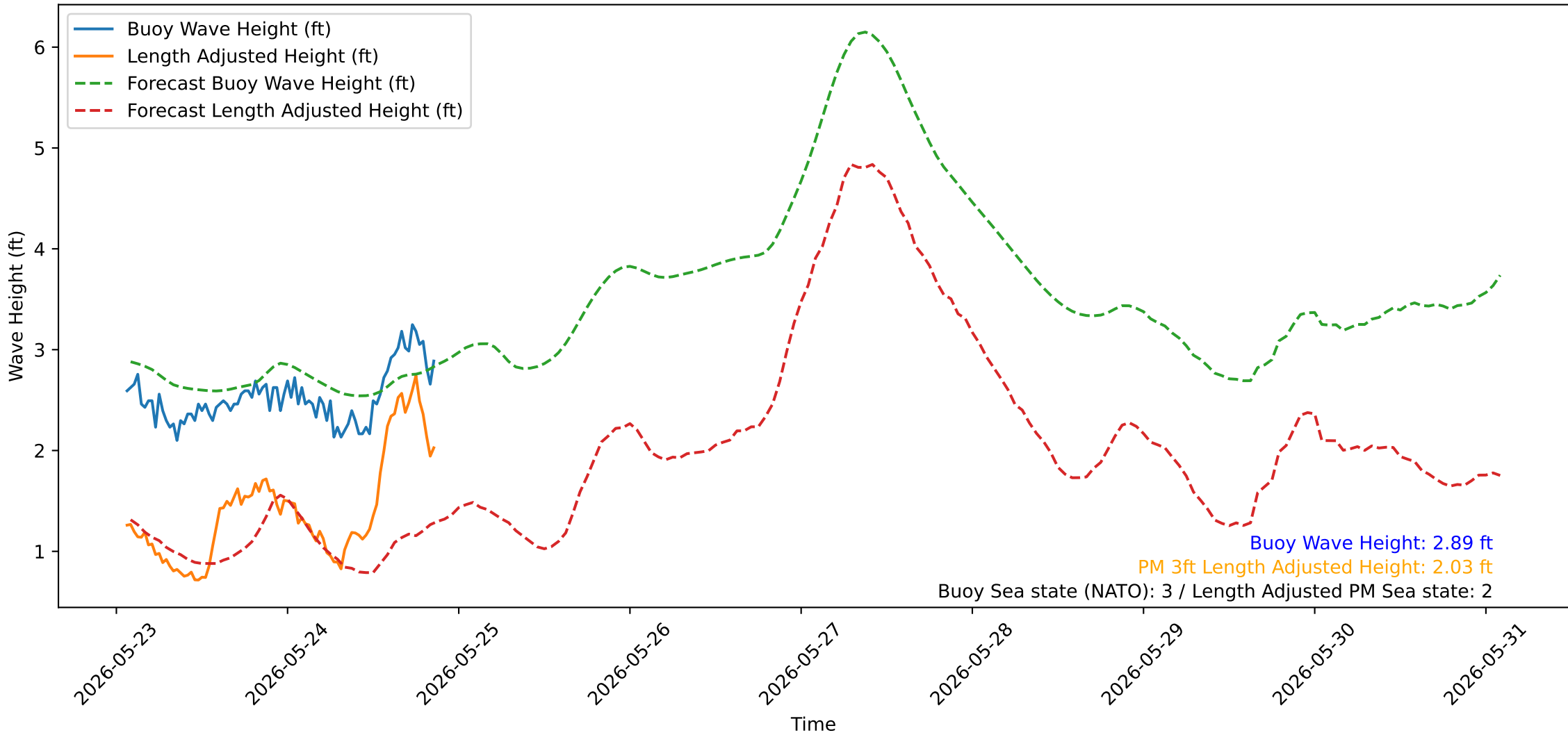
Wave Heights over Time for Oceanside Harbor at 2026-05-26 01:40:29
