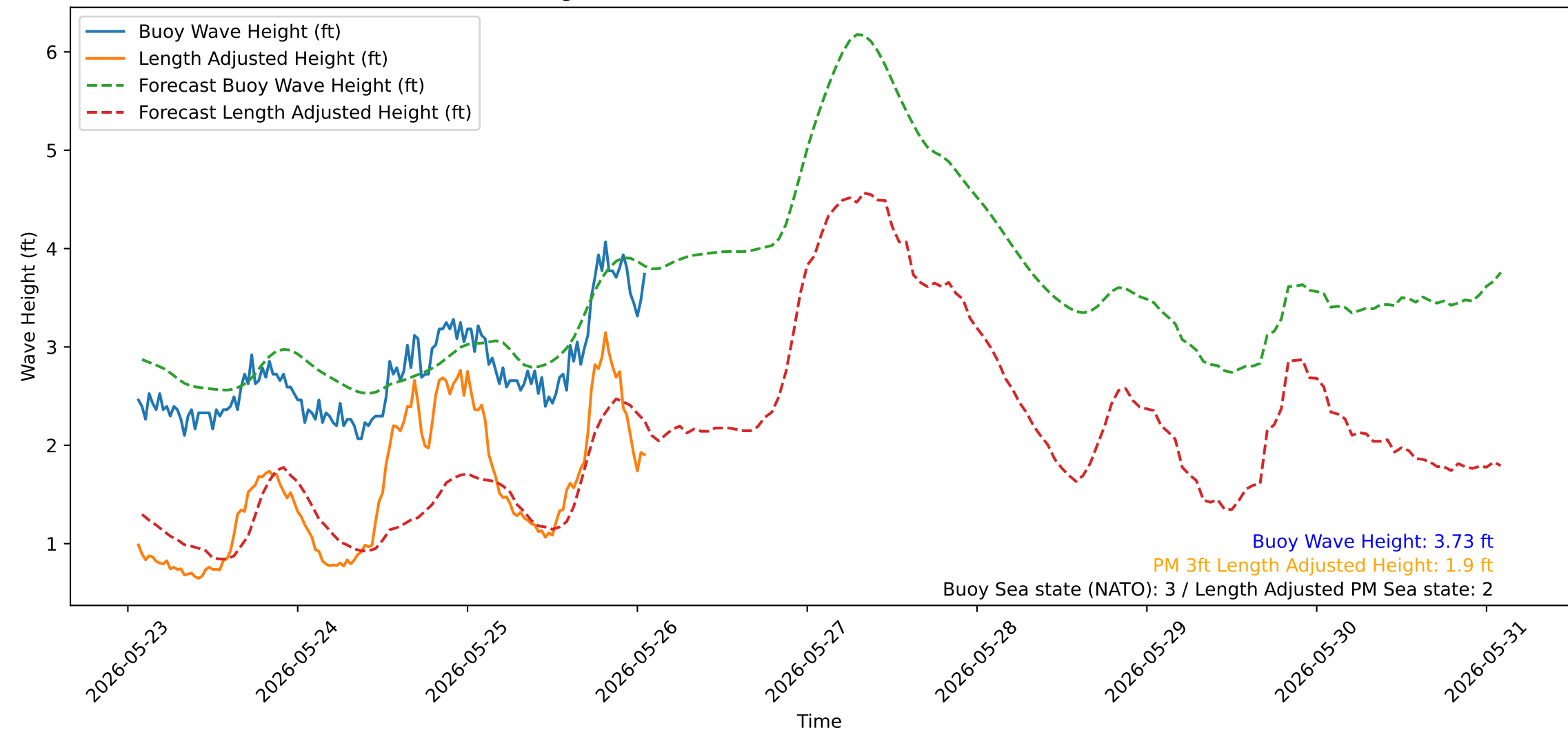
Wave Heights over Time for Green Beach at 2026-05-26 01:41:11
