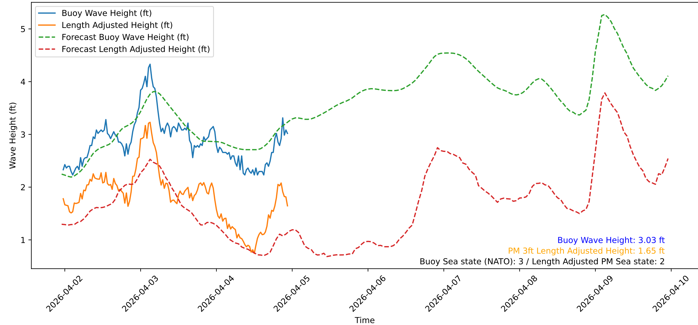
Wave Heights over Time for Green Beach at 2026-04-04 23:21:15
