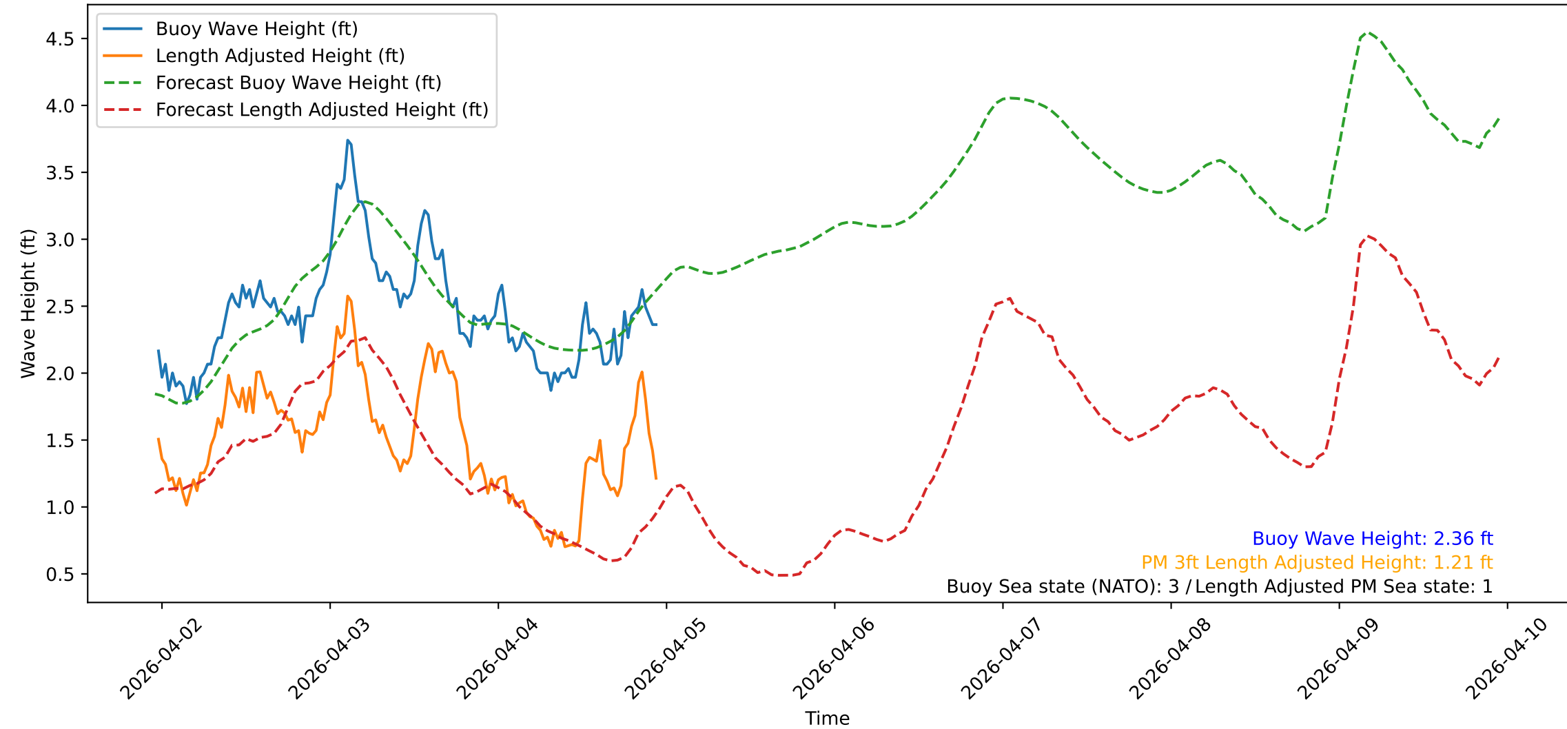
Wave Heights over Time for Red Beach at 2026-04-04 23:20:50
