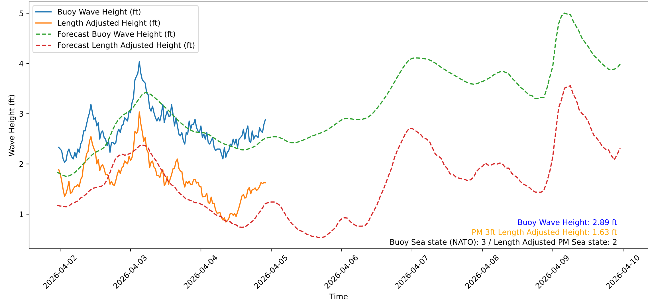
Wave Heights over Time for Oceanside Harbor at 2026-04-04 23:20:34
