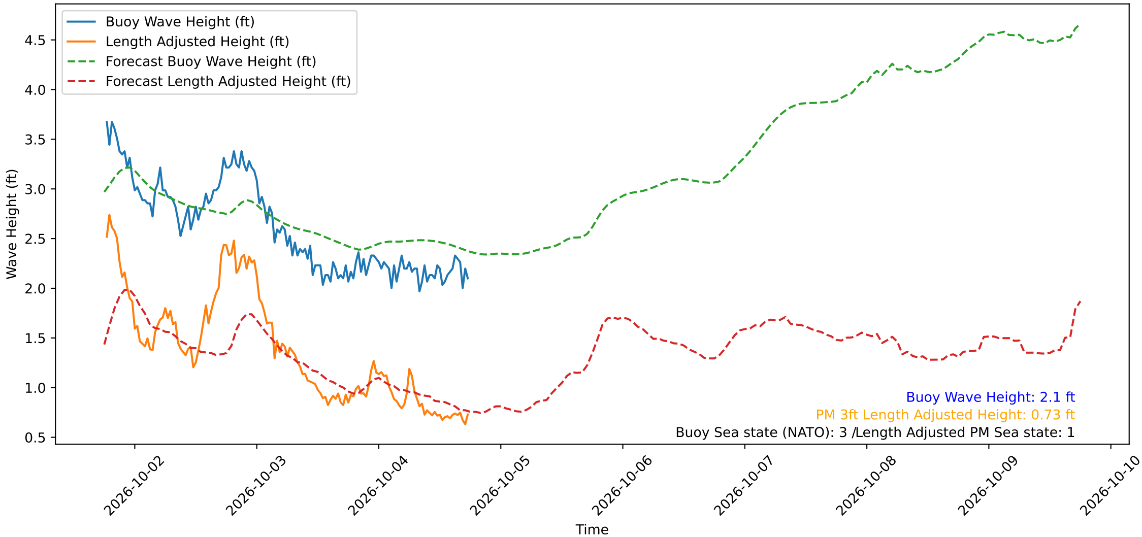
Wave Heights over Time for Green Beach at 2026-10-04 18:11:11
