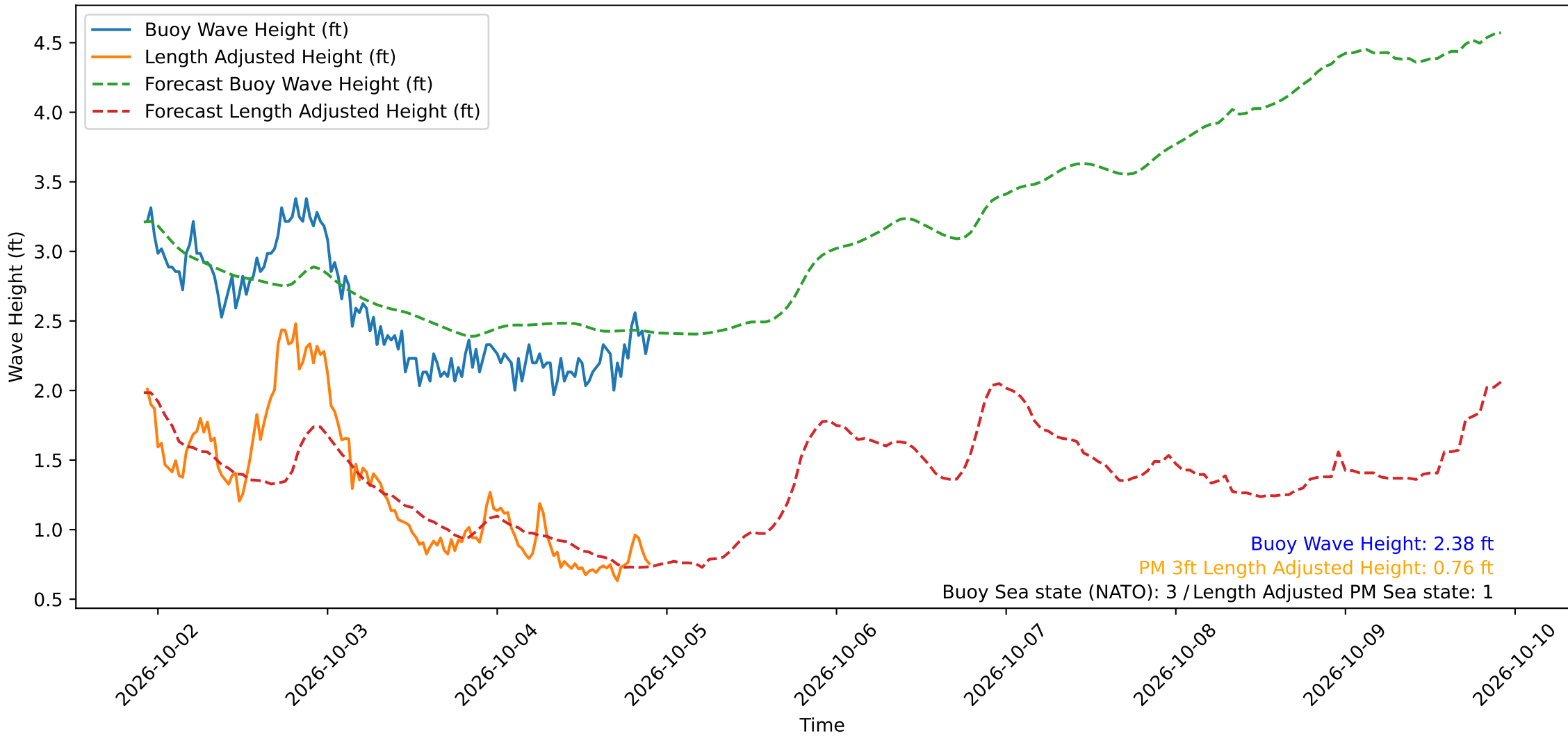
Wave Heights over Time for Green Beach at 2026-10-04 22:11:11
