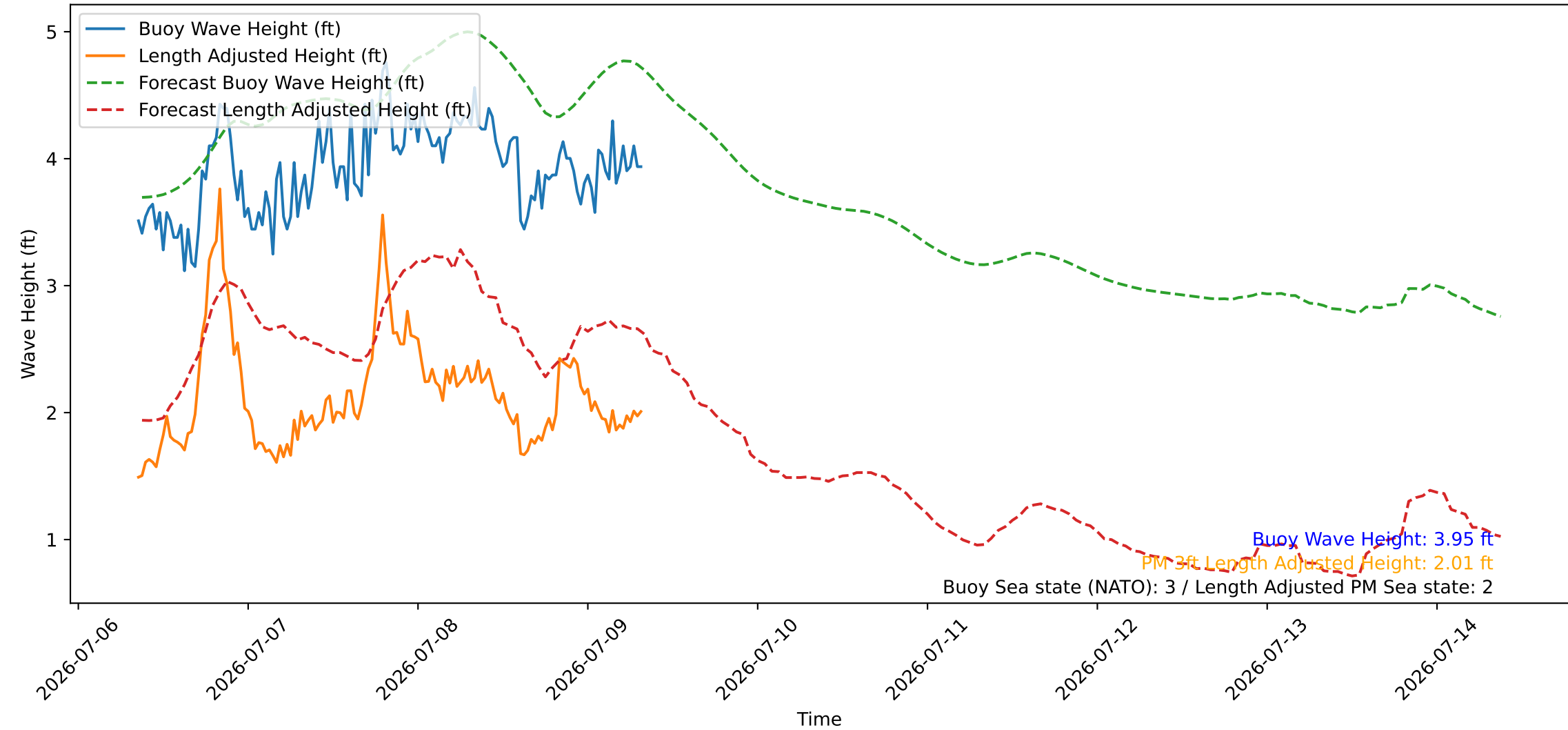
Wave Heights over Time for Green Beach at 2026-07-09 08:41:08
