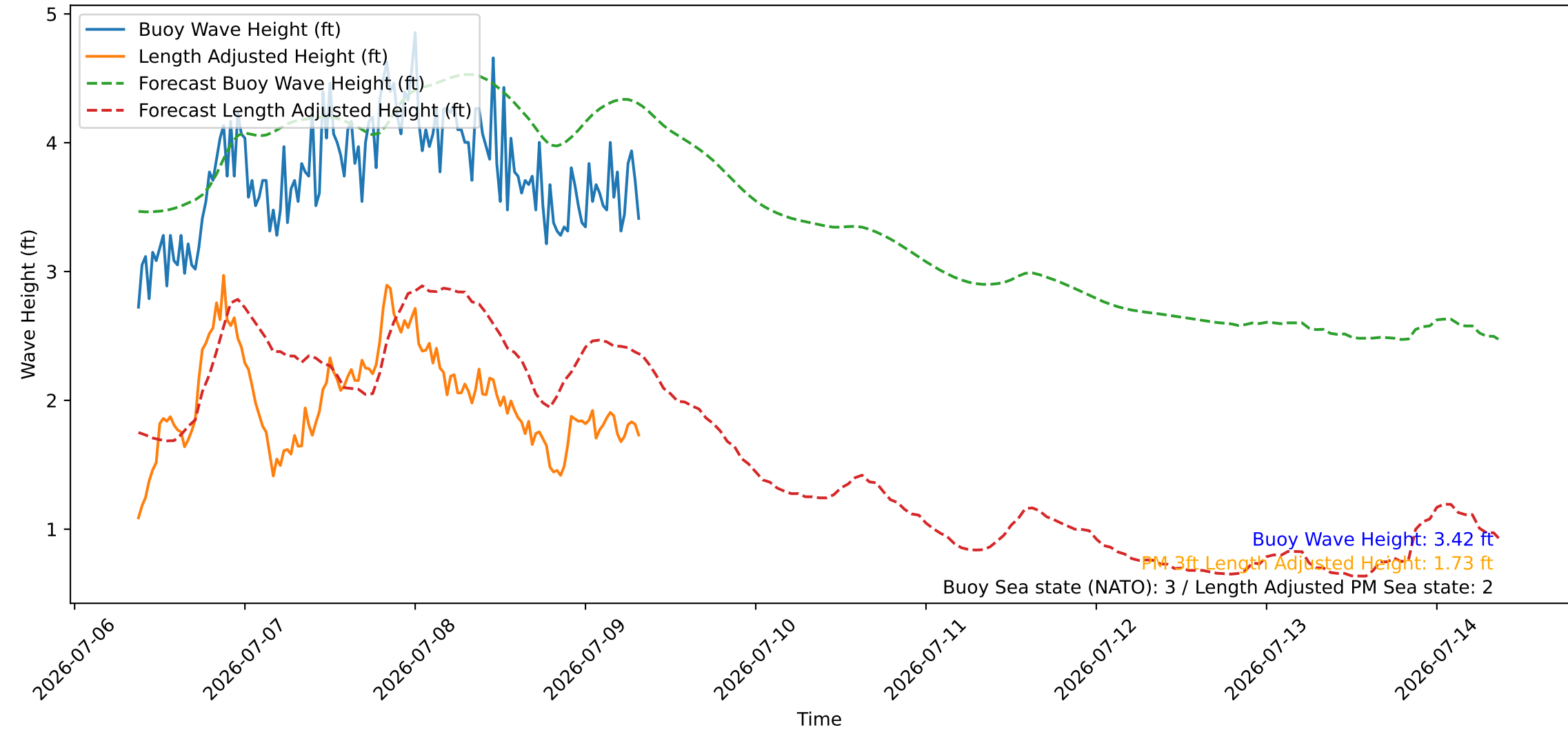
Wave Heights over Time for Red Beach at 2026-07-09 08:40:46
