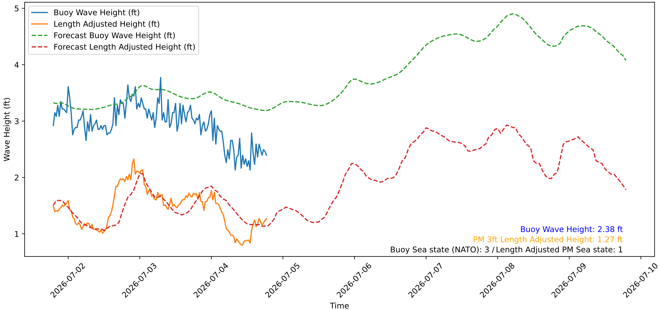
Wave Heights over Time for Oceanside Harbor at 2026-07-04 19:00:27
