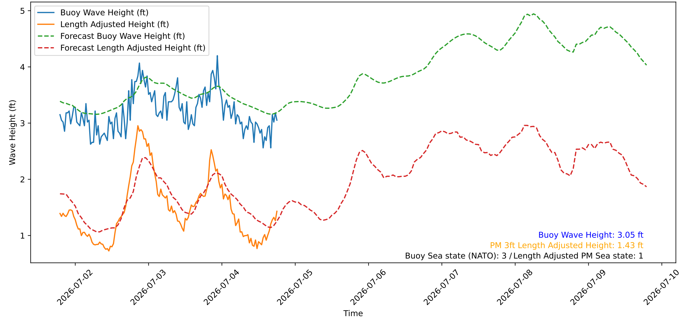
Wave Heights over Time for Green Beach at 2026-07-04 19:01:08
