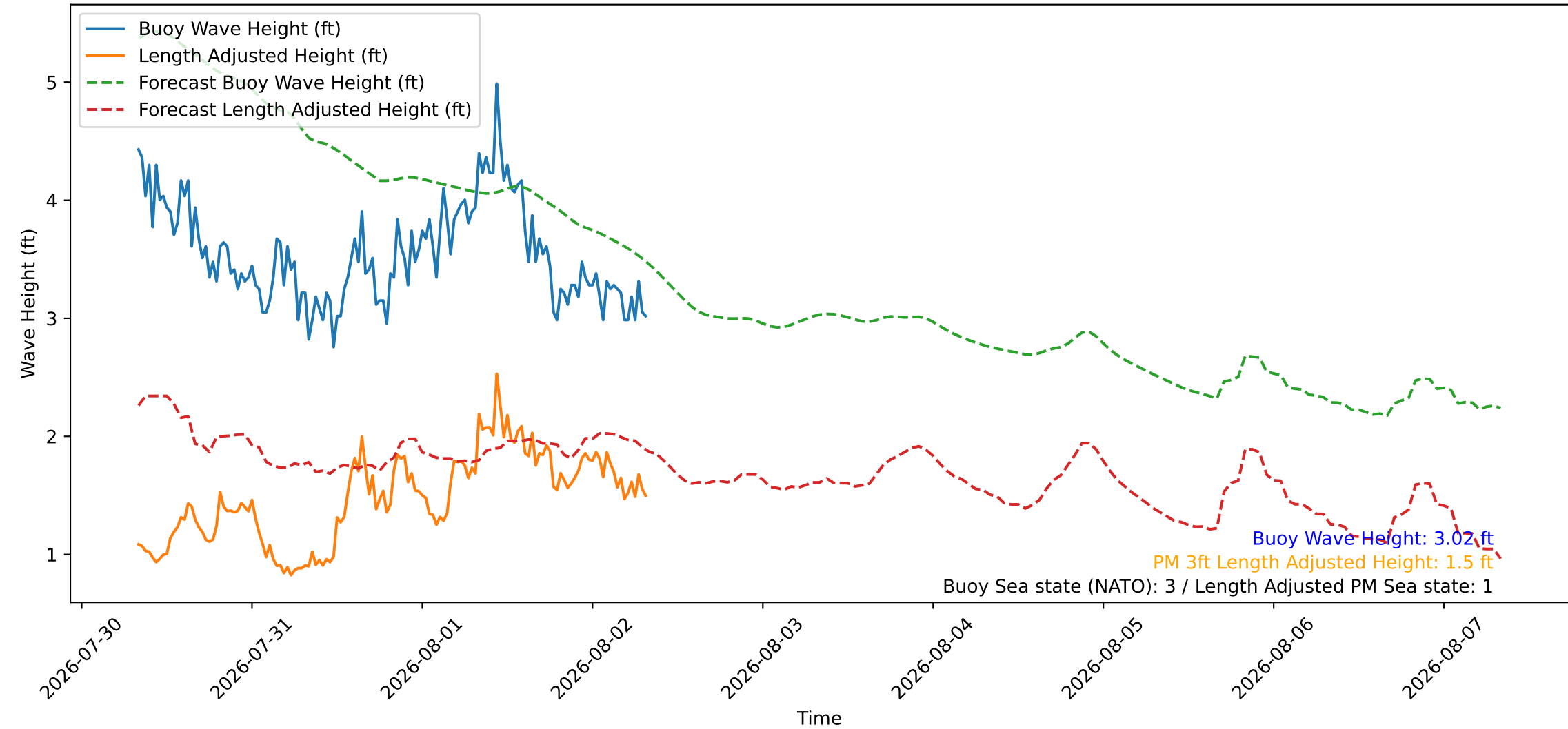
Wave Heights over Time for Green Beach at 2026-08-02 08:11:08
