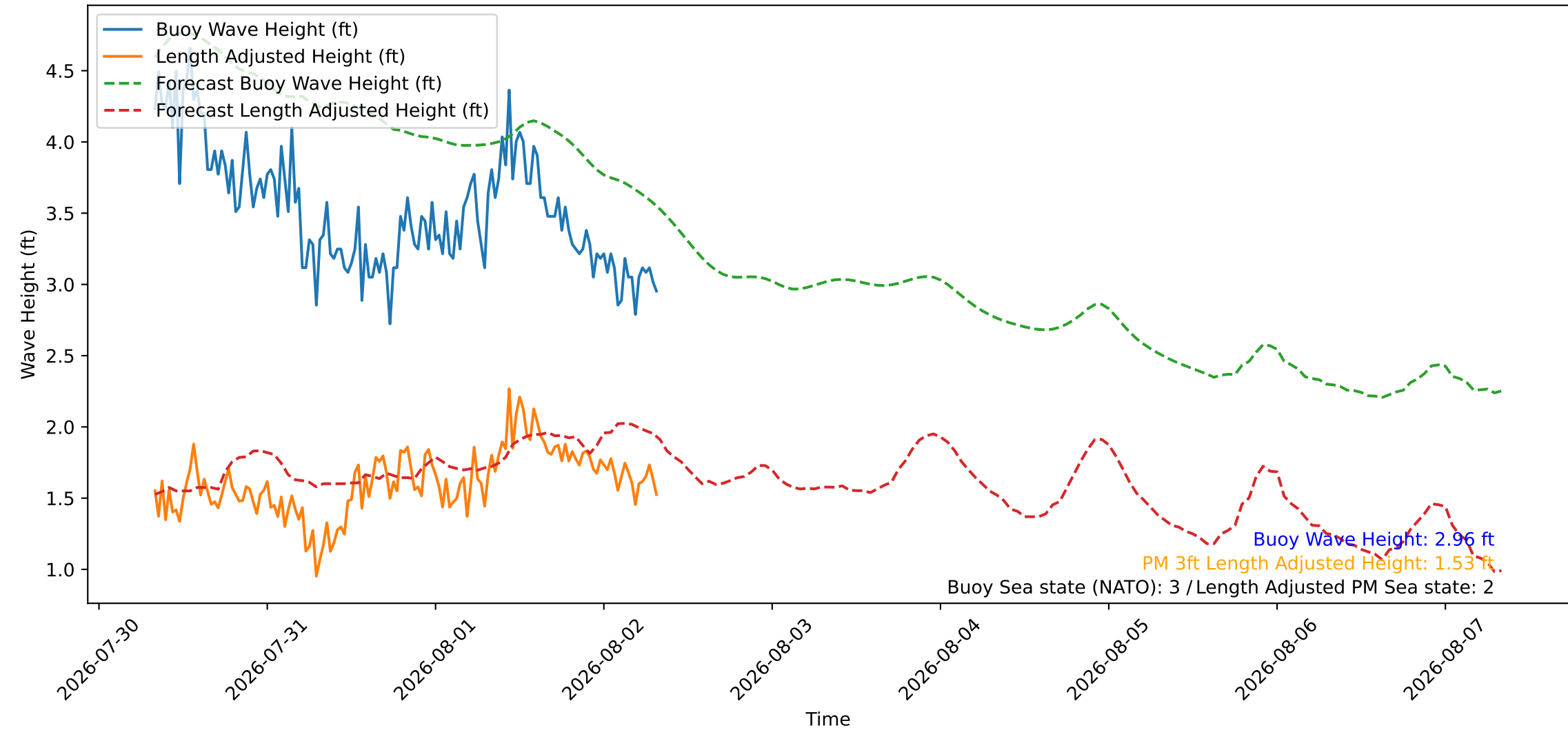
Wave Heights over Time for Oceanside Harbor at 2026-08-02 08:10:26
