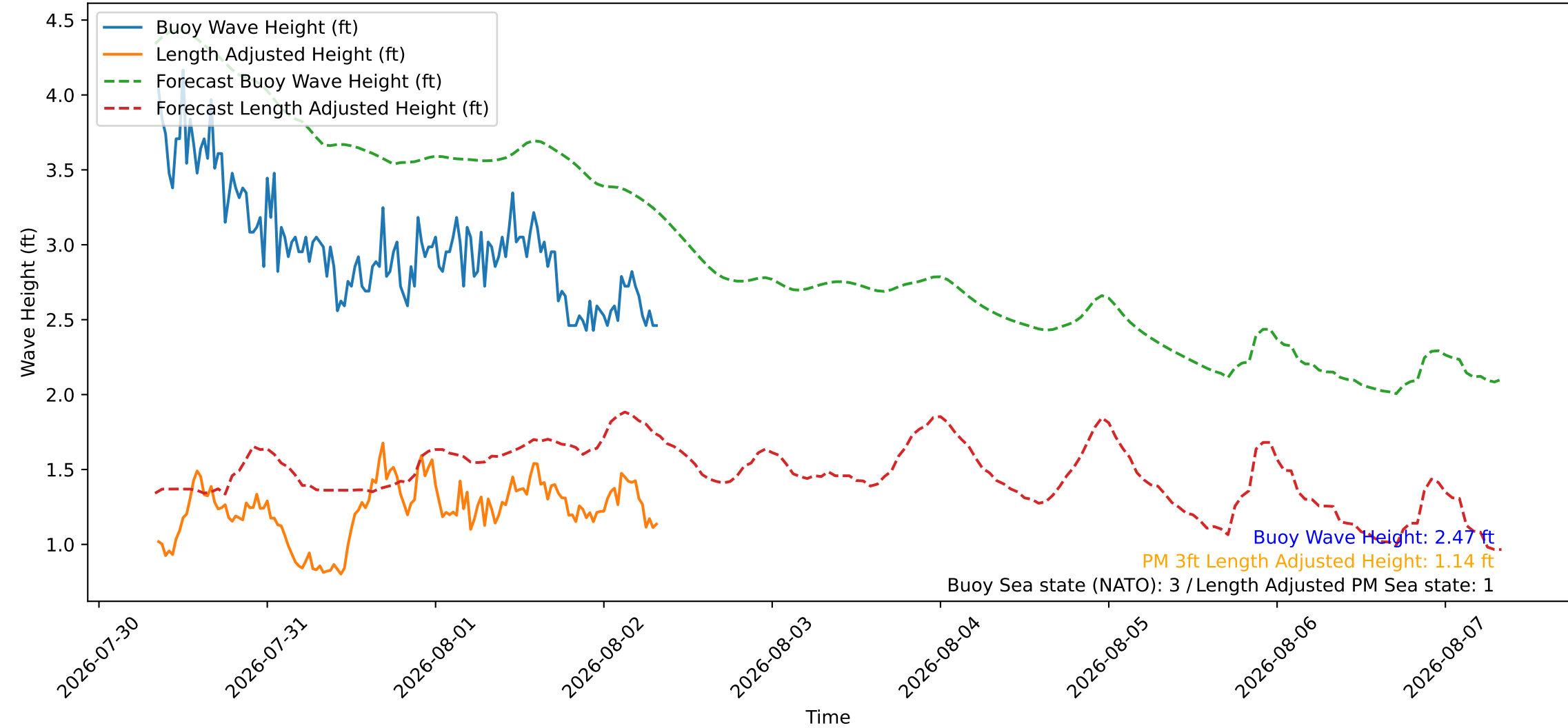
Wave Heights over Time for Red Beach at 2026-08-02 08:10:45
