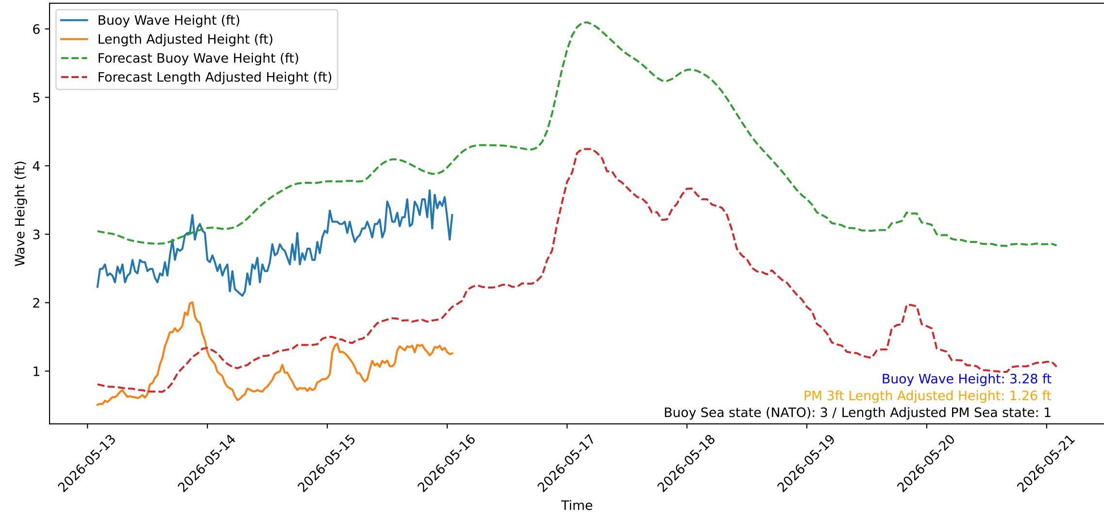
Wave Heights over Time for Green Beach at 2026-05-16 02:01:12
