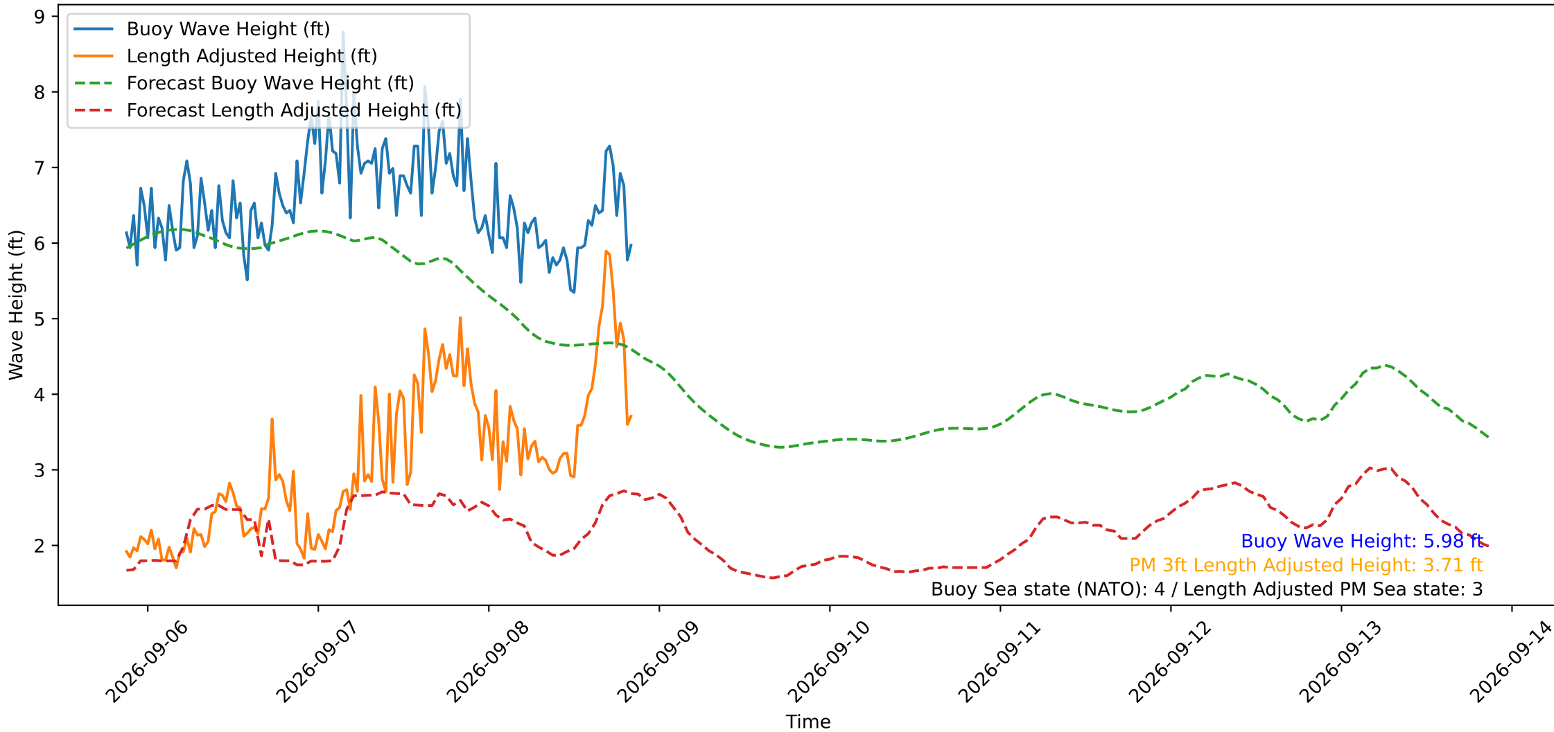
Wave Heights over Time for Green Beach at 2026-09-08 20:51:13
