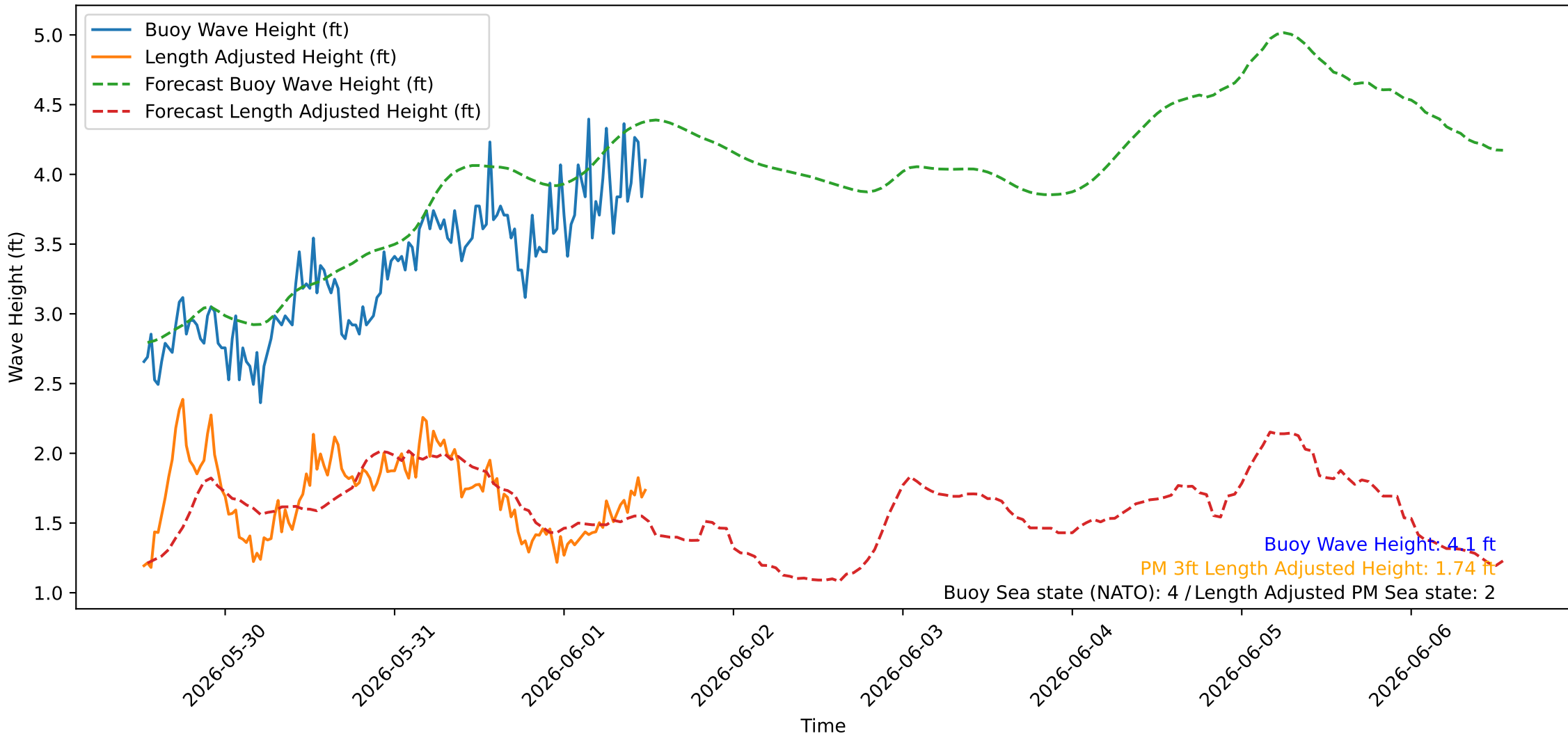
Wave Heights over Time for Oceanside Harbor at 2026-06-01 12:30:25
