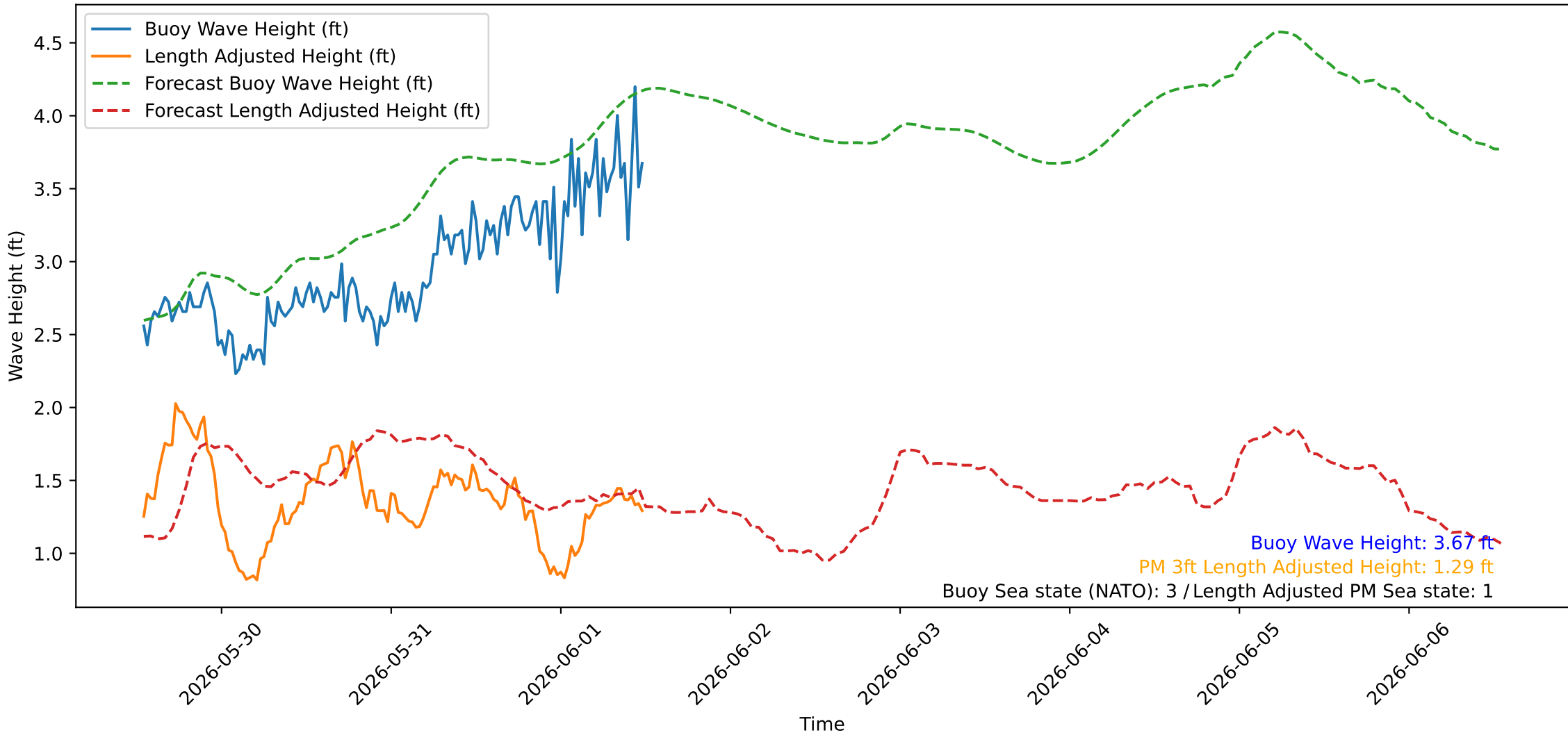
Wave Heights over Time for Red Beach at 2026-06-01 12:30:45
