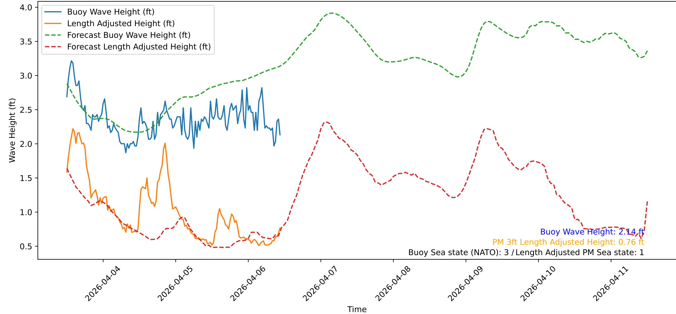
Wave Heights over Time for Red Beach at 2026-04-06 11:40:51
