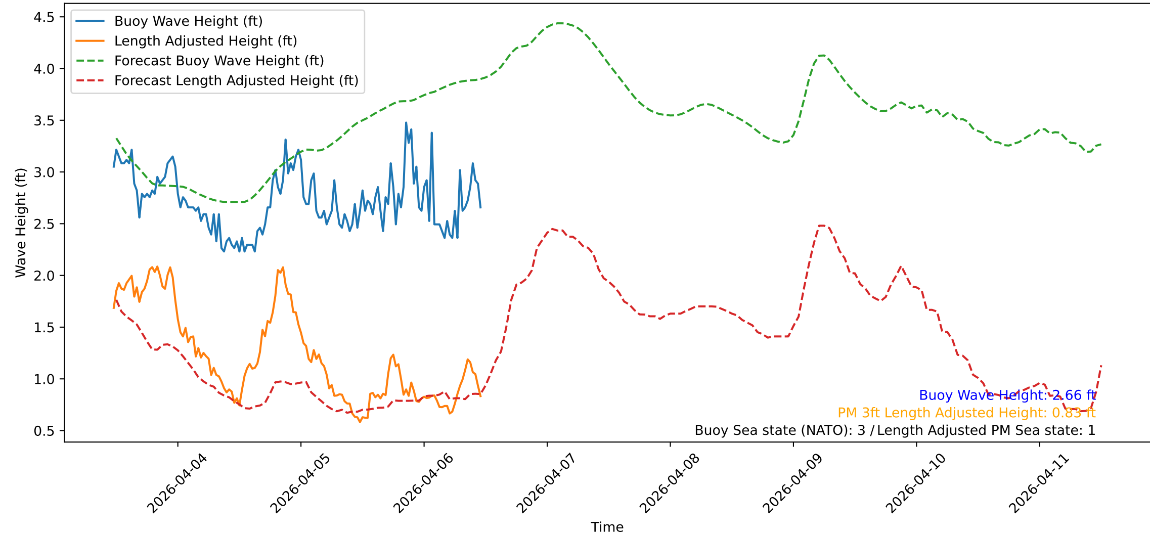
Wave Heights over Time for Green Beach at 2026-04-06 11:41:14
