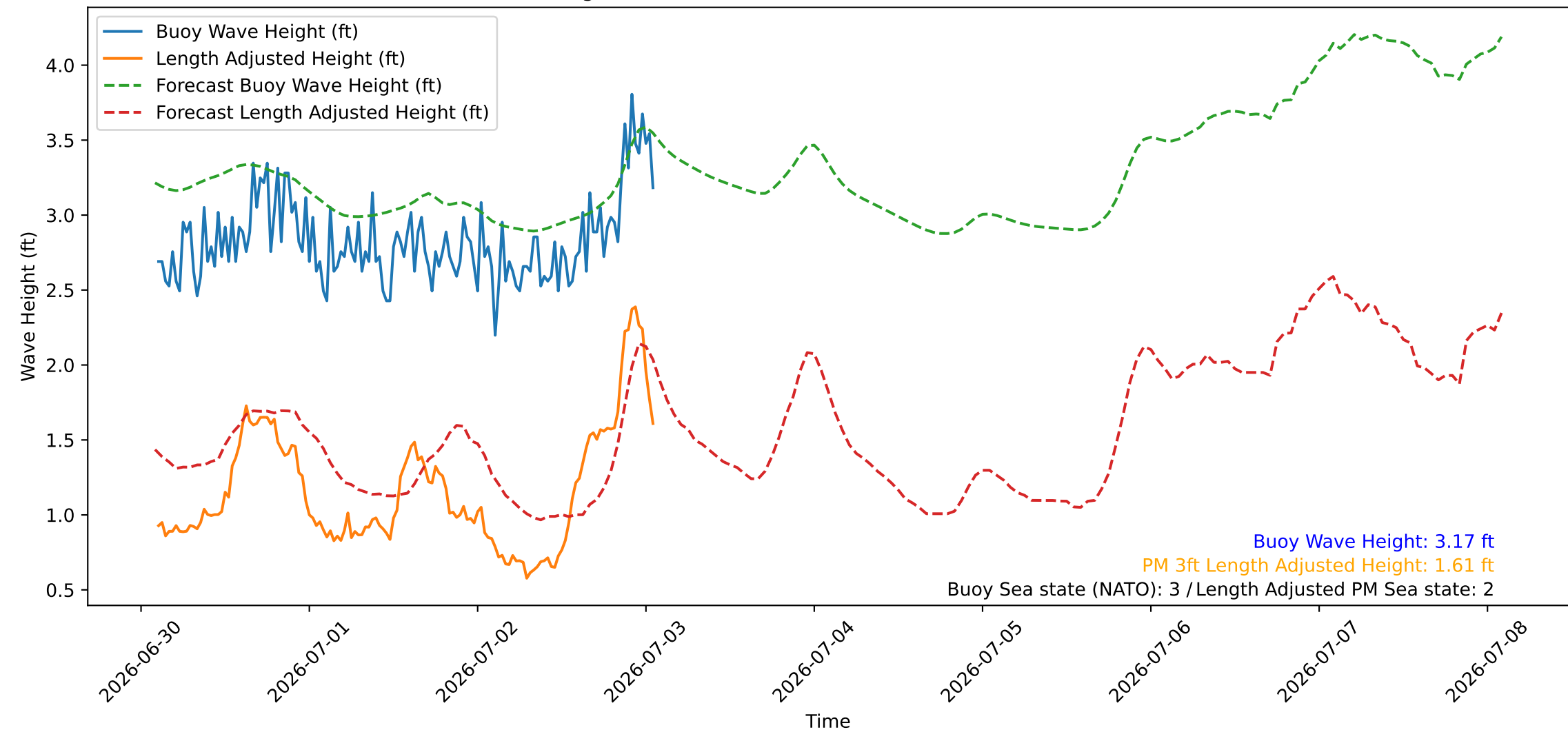
Wave Heights over Time for Red Beach at 2026-07-03 02:00:44
