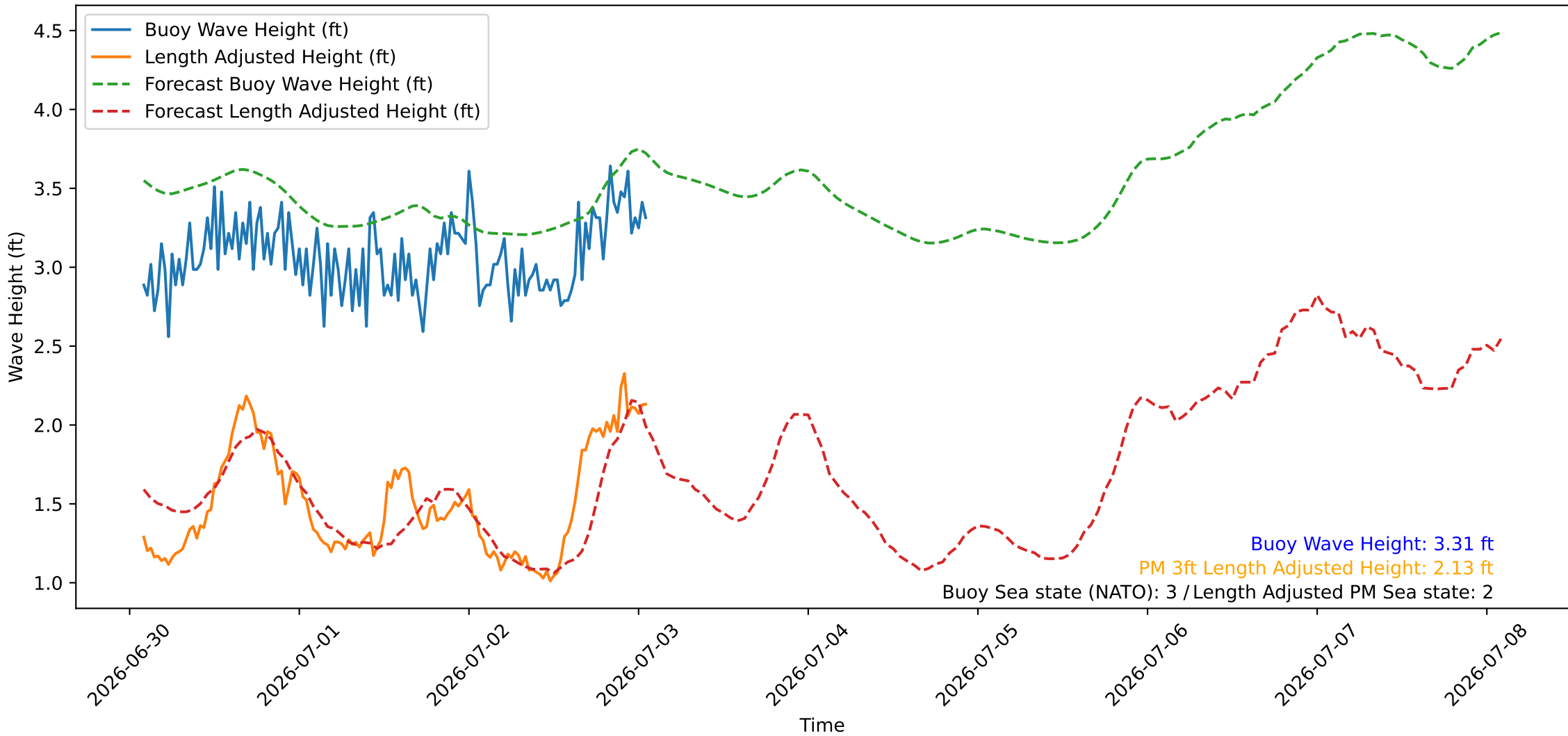
Wave Heights over Time for Oceanside Harbor at 2026-07-03 02:00:26
