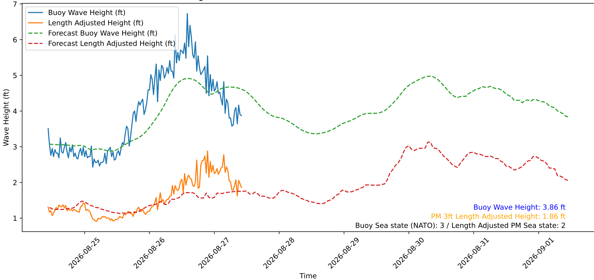
Wave Heights over Time for Oceanside Harbor at 2026-08-27 10:40:30
