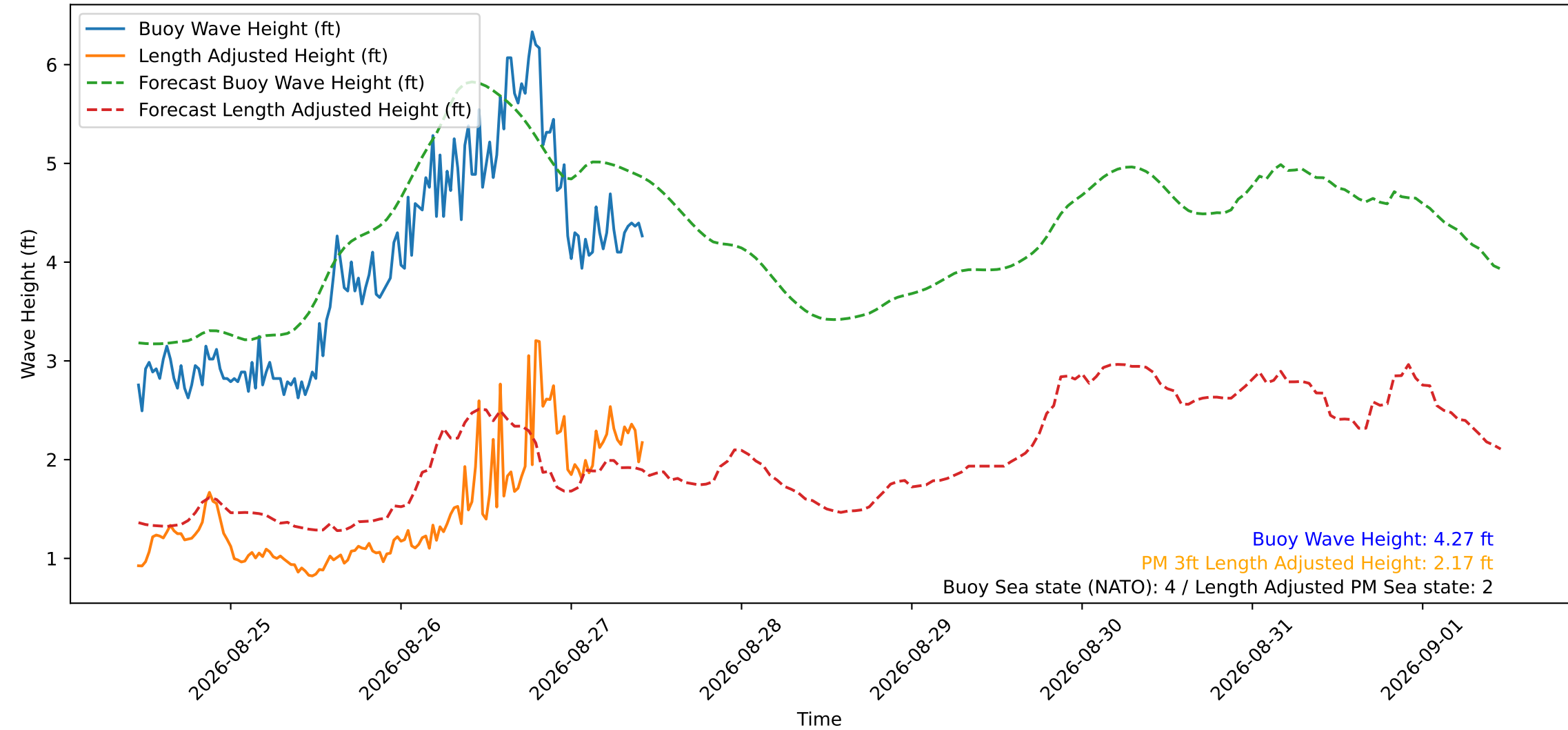
Wave Heights over Time for Green Beach at 2026-08-27 10:41:12
