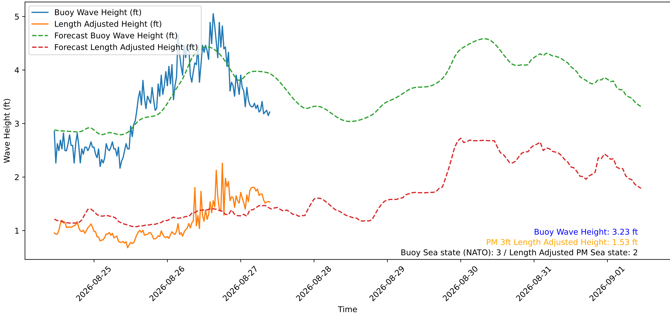
Wave Heights over Time for Red Beach at 2026-08-27 10:40:50
