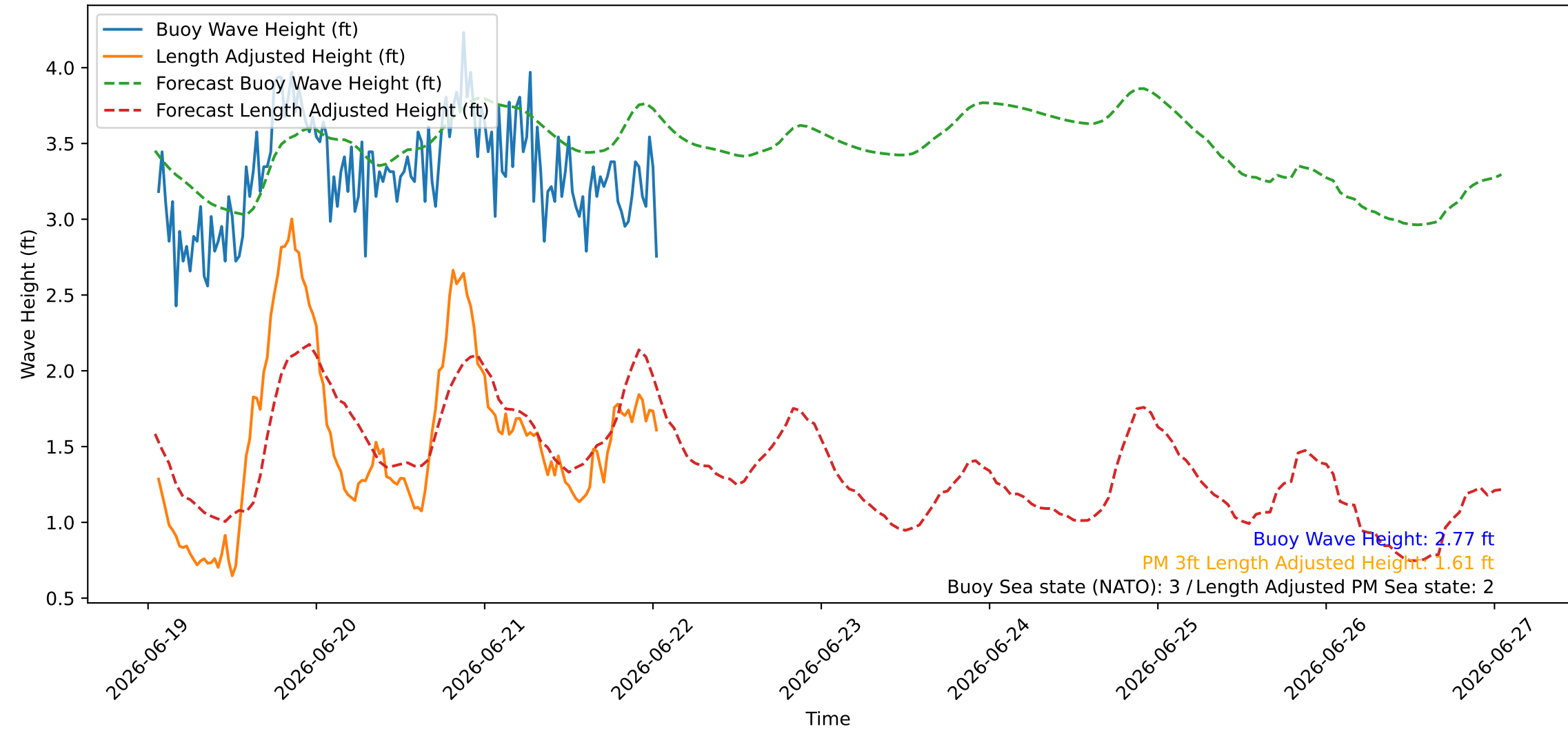
Wave Heights over Time for Green Beach at 2026-06-22 01:21:08
