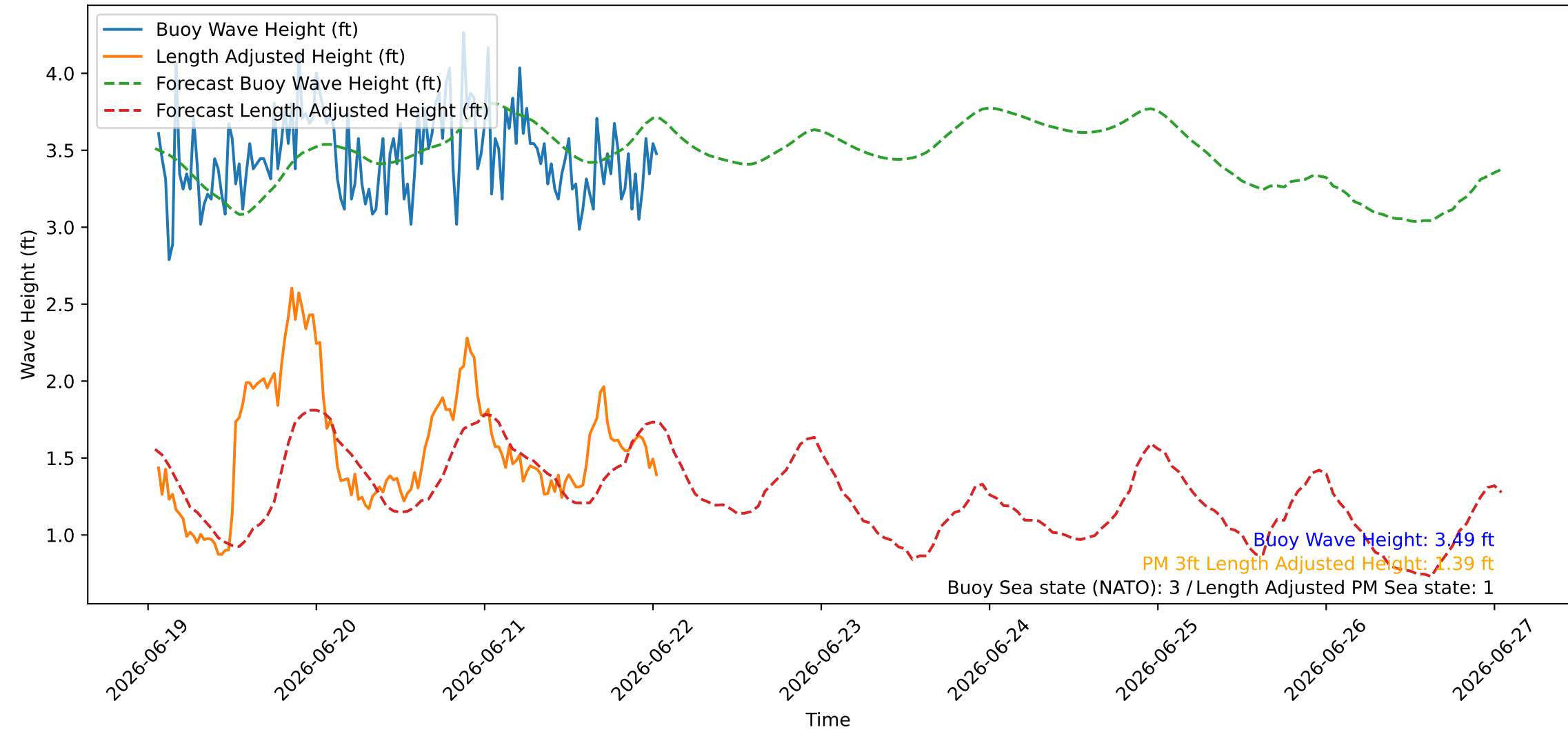
Wave Heights over Time for Oceanside Harbor at 2026-06-22 01:20:25
