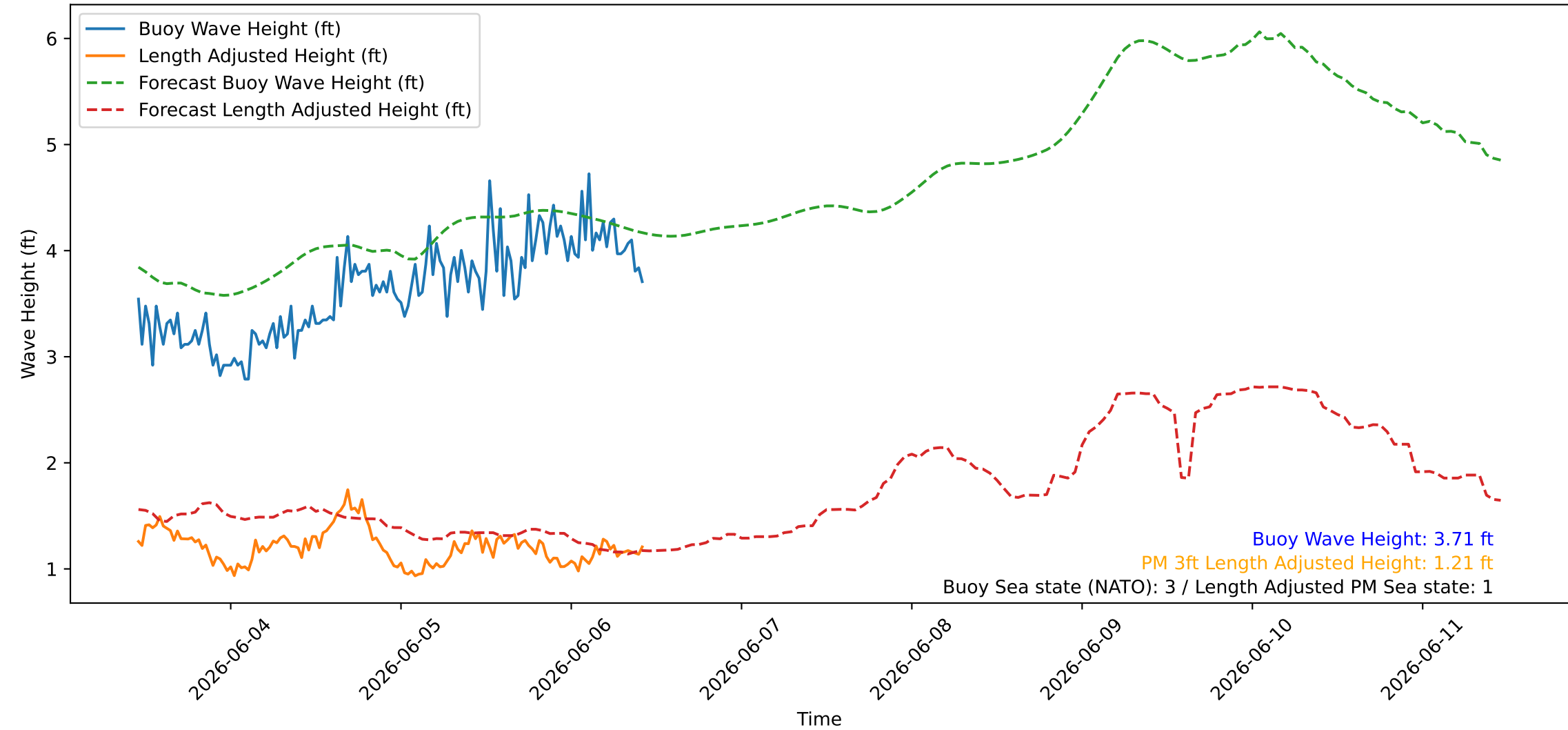
Wave Heights over Time for Green Beach at 2026-06-06 11:01:08
