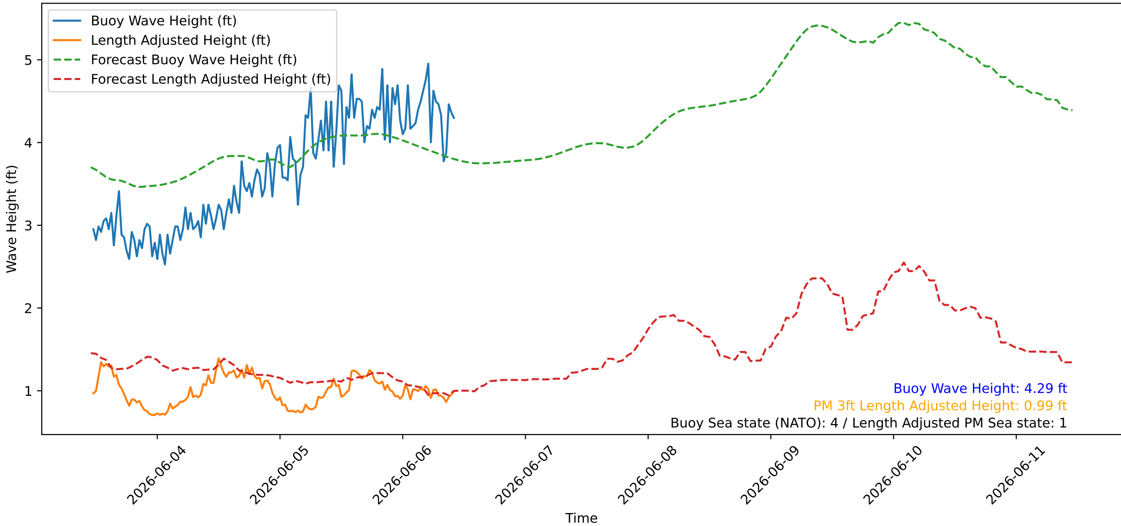
Wave Heights over Time for Red Beach at 2026-06-06 11:00:46
