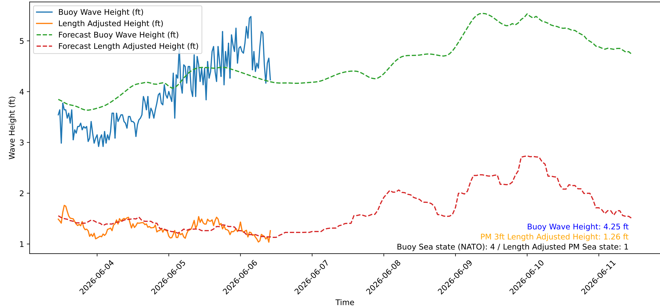
Wave Heights over Time for Oceanside Harbor at 2026-06-06 11:00:26
