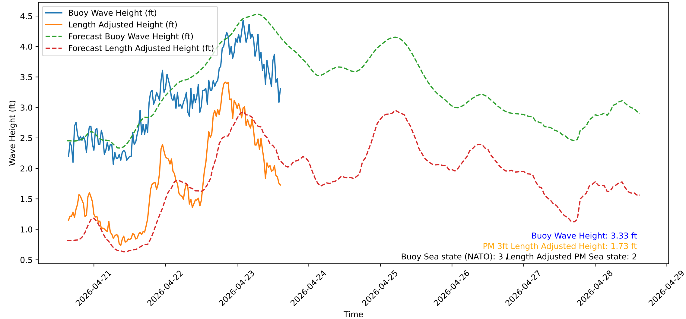
Wave Heights over Time for Oceanside Harbor at 2026-04-23 15:20:31
