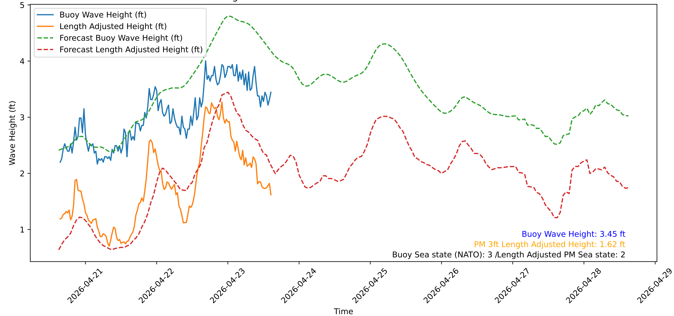
Wave Heights over Time for Green Beach at 2026-04-23 15:21:13
