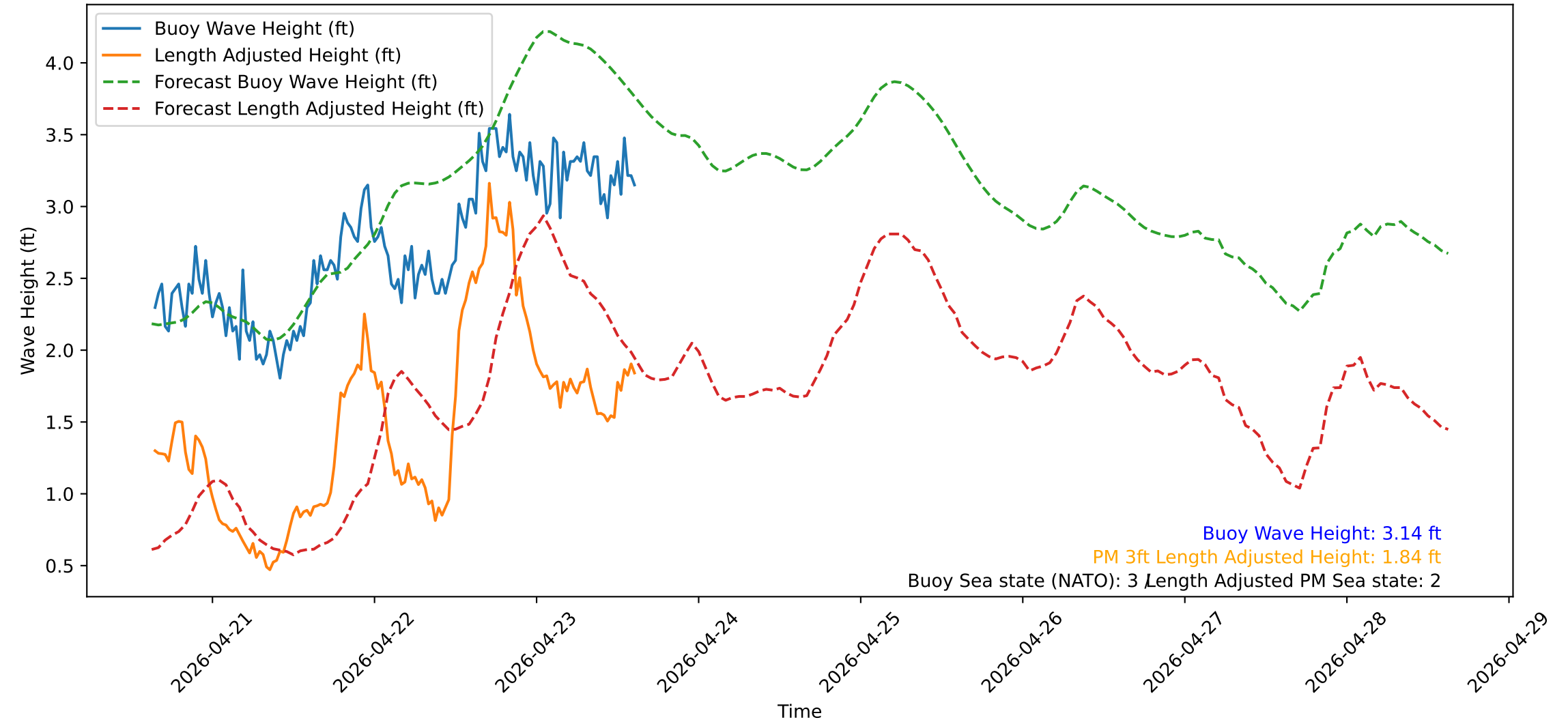
Wave Heights over Time for Red Beach at 2026-04-23 15:20:51
