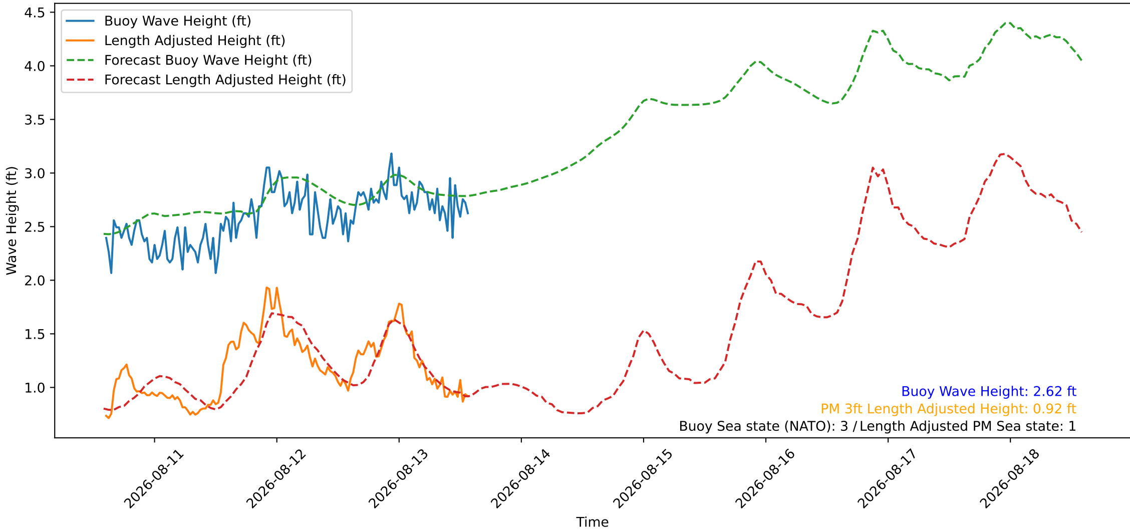
Wave Heights over Time for Oceanside Harbor at 2026-08-13 14:20:26
