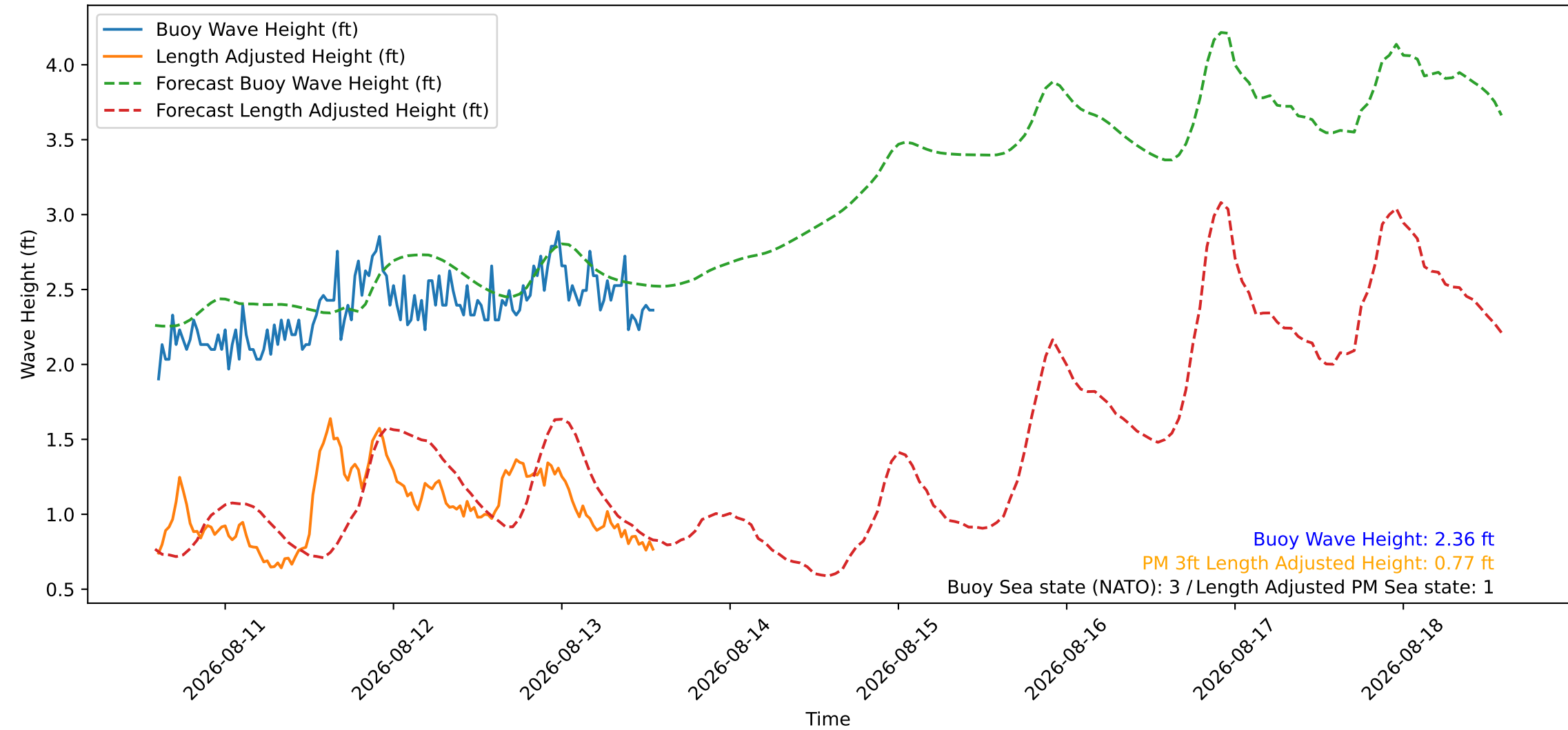
Wave Heights over Time for Red Beach at 2026-08-13 14:20:47
