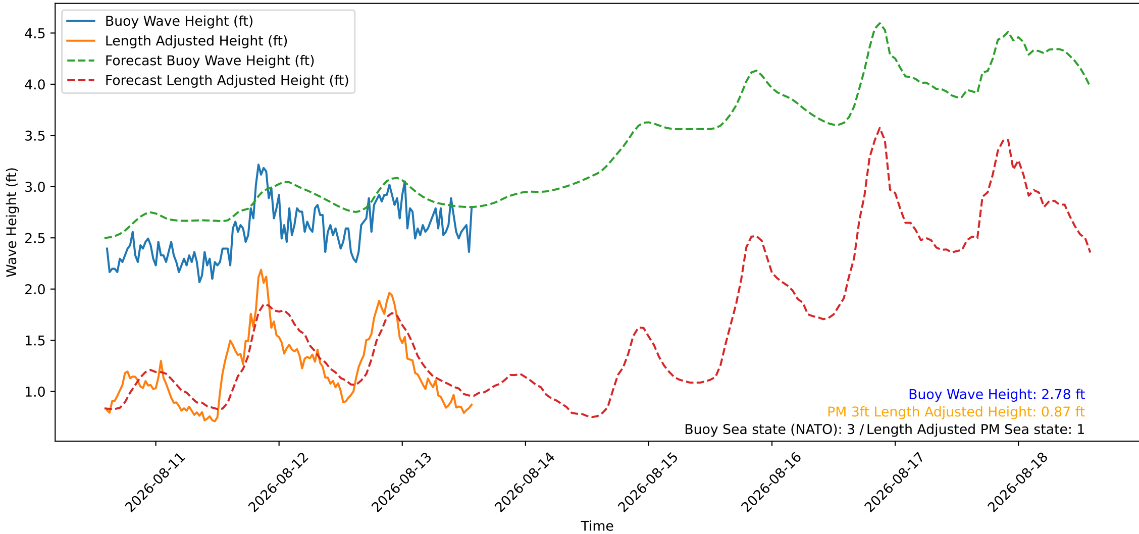
Wave Heights over Time for Green Beach at 2026-08-13 14:21:09
