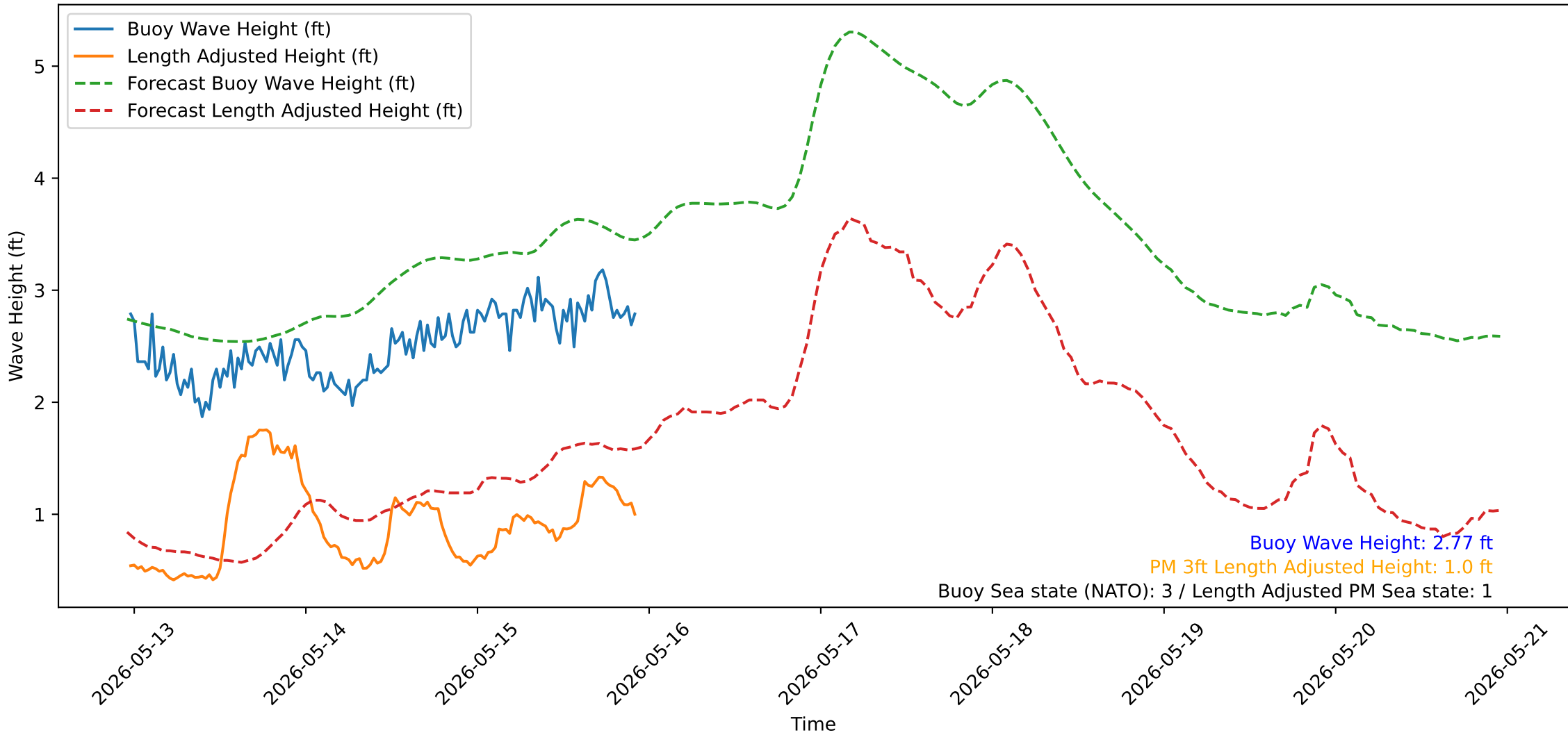
Wave Heights over Time for Red Beach at 2026-05-15 23:00:50
