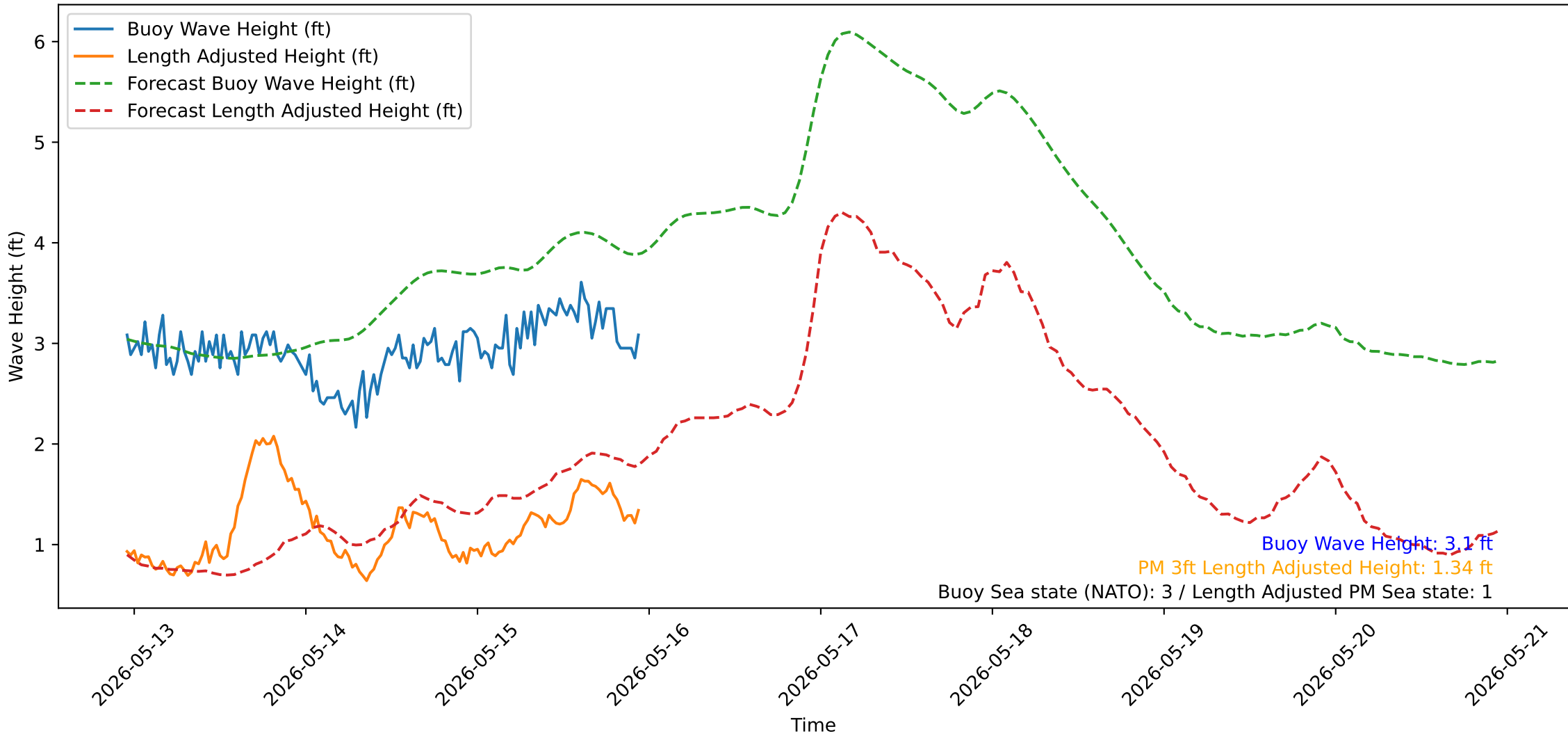
Wave Heights over Time for Oceanside Harbor at 2026-05-15 23:00:31
