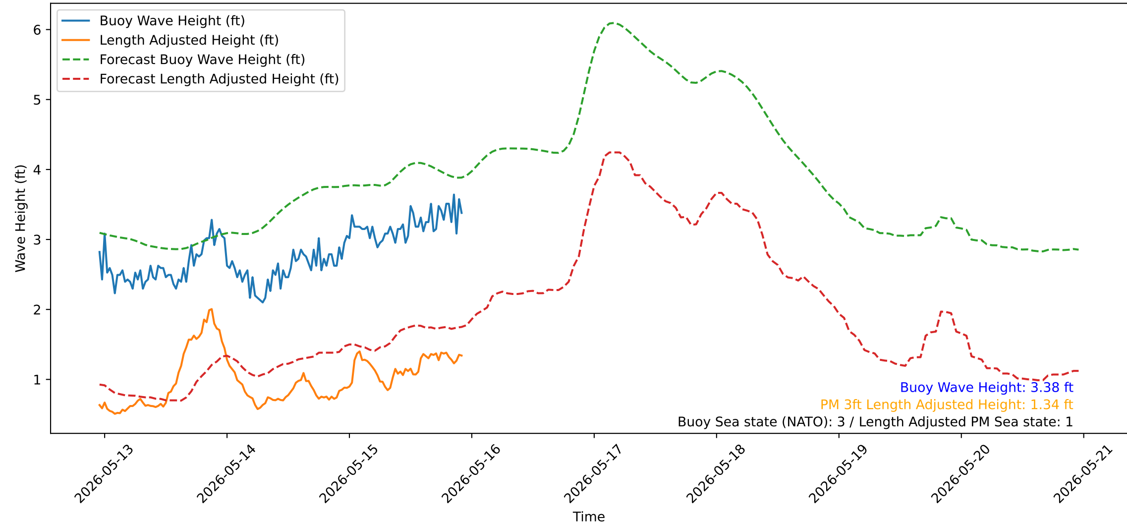
Wave Heights over Time for Green Beach at 2026-05-15 23:01:13
