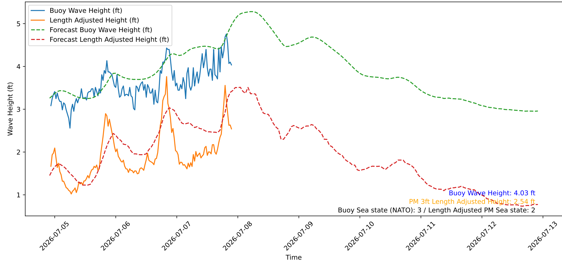
Wave Heights over Time for Green Beach at 2026-07-07 22:21:09
