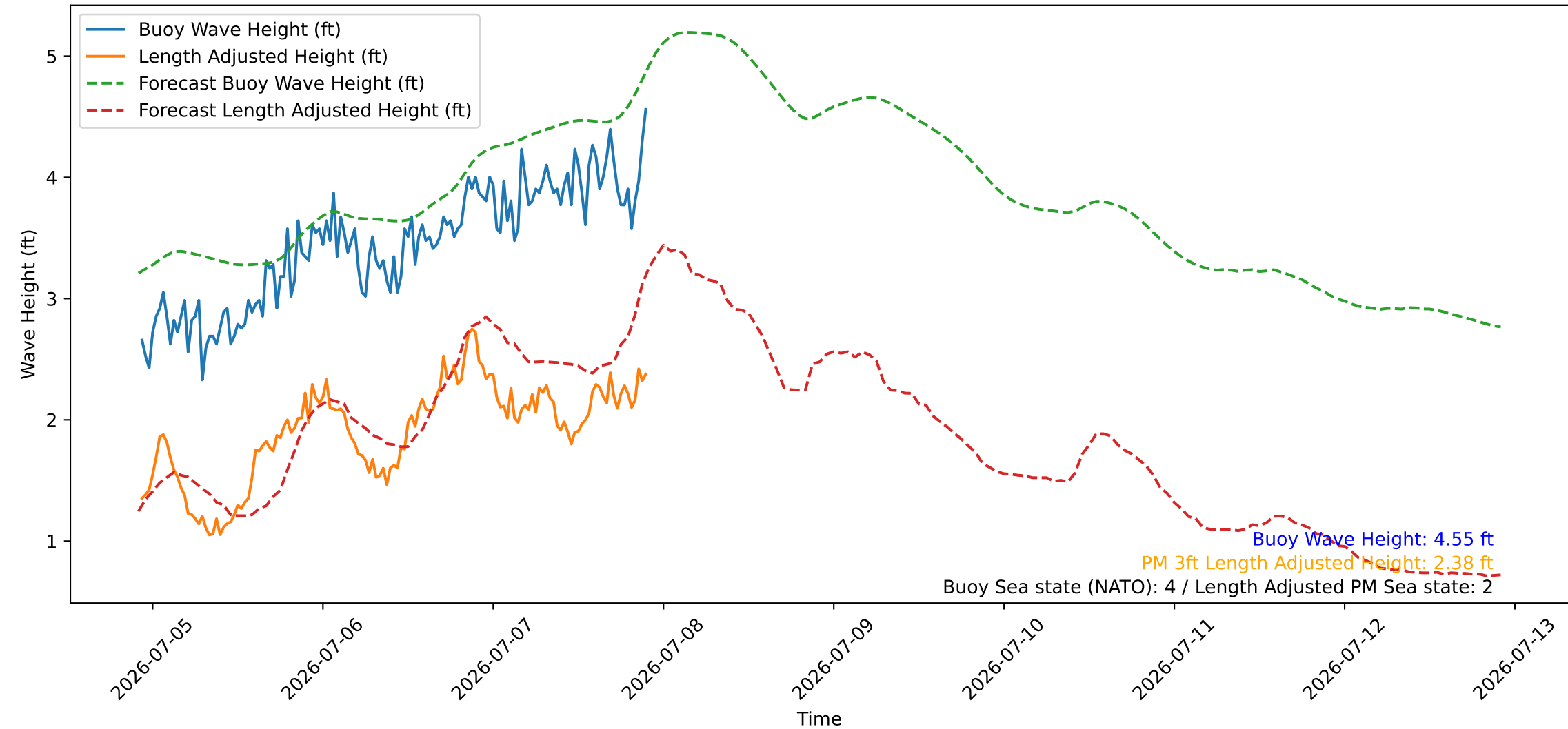
Wave Heights over Time for Oceanside Harbor at 2026-07-07 22:20:26
