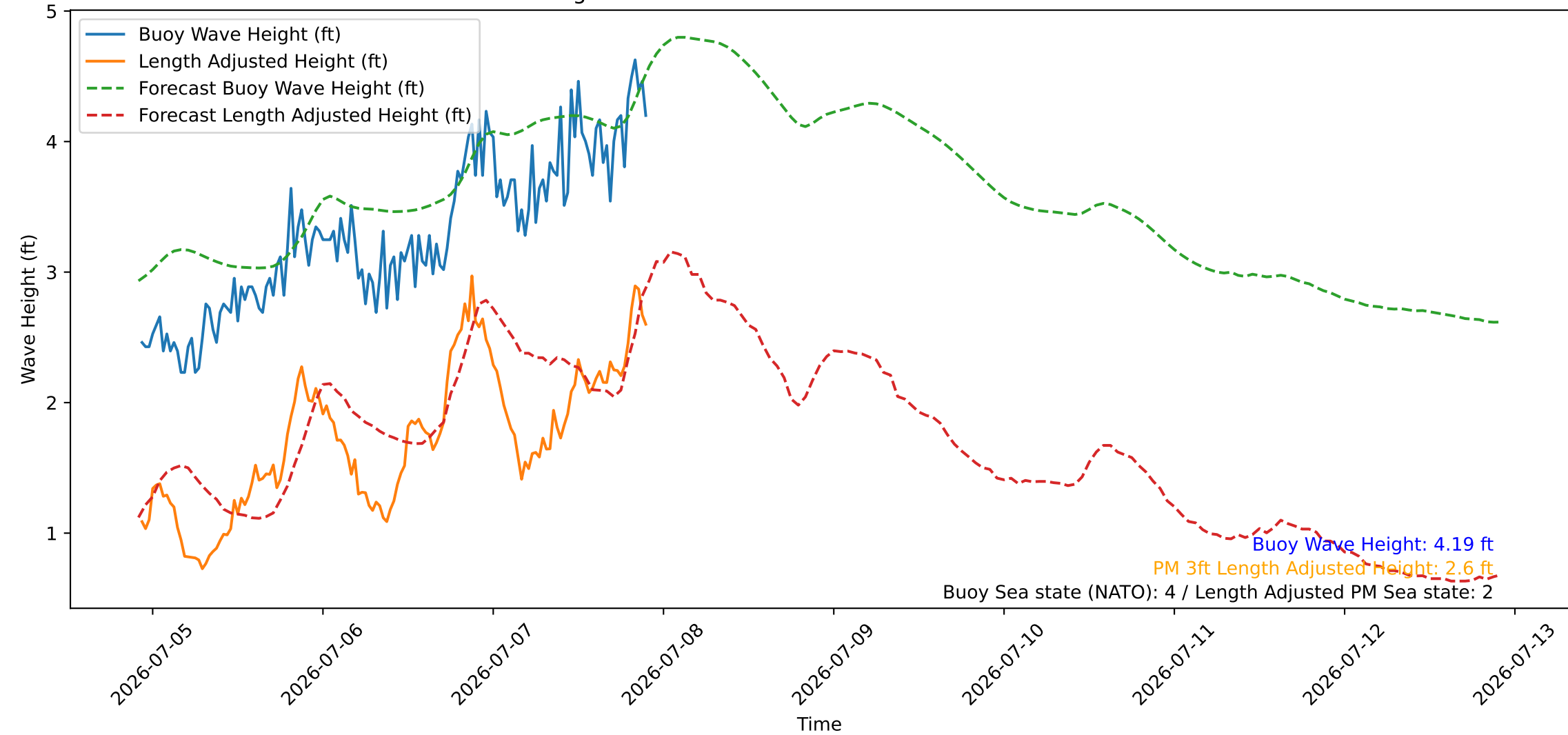
Wave Heights over Time for Red Beach at 2026-07-07 22:20:47
