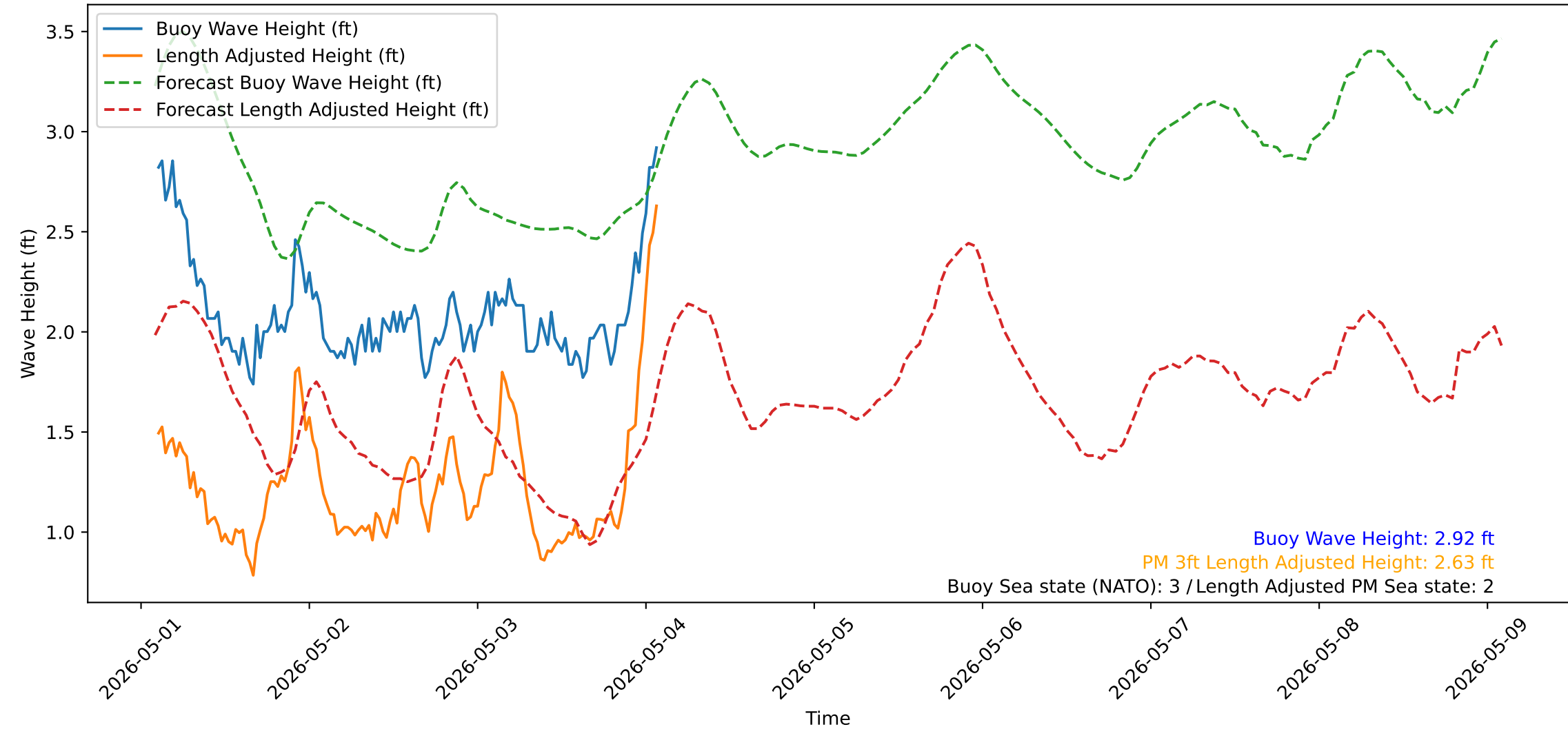
Wave Heights over Time for Green Beach at 2026-05-04 02:21:13
