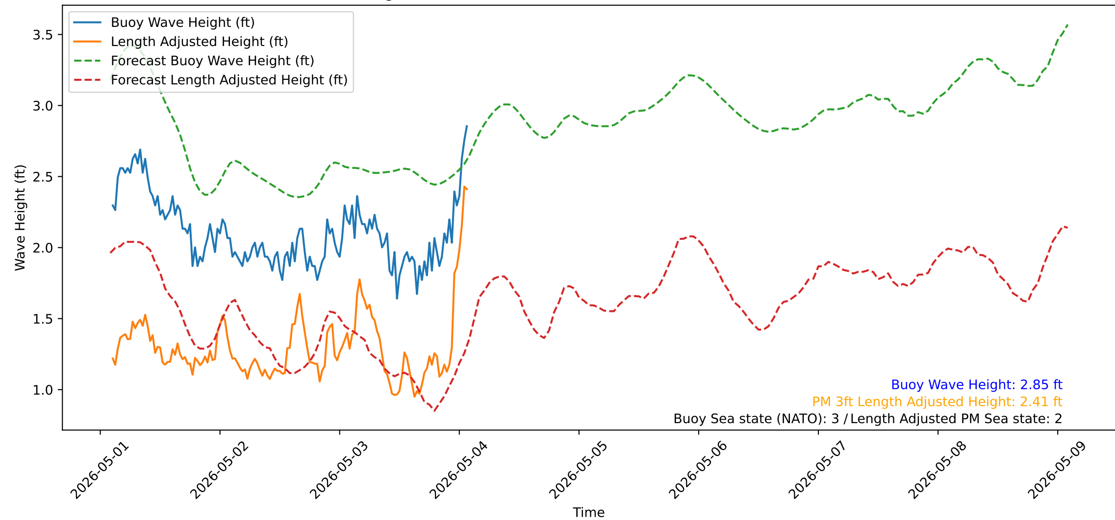
Wave Heights over Time for Oceanside Harbor at 2026-05-04 02:20:31
