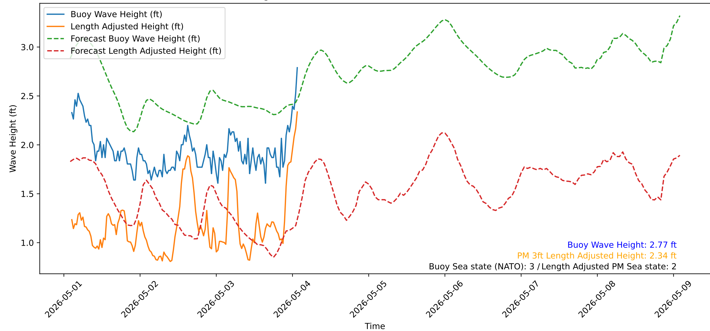
Wave Heights over Time for Red Beach at 2026-05-04 02:20:51
