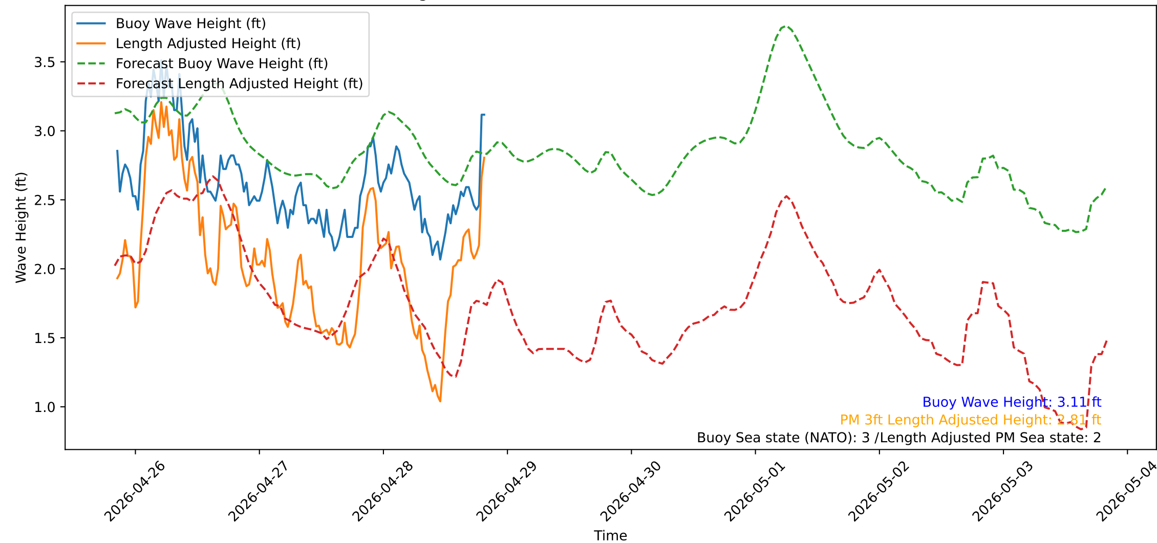
Wave Heights over Time for Green Beach at 2026-04-28 20:21:14
