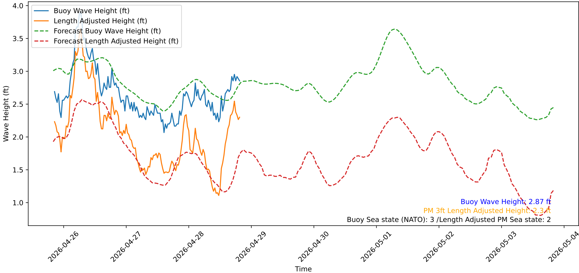
Wave Heights over Time for Oceanside Harbor at 2026-04-28 20:20:31
