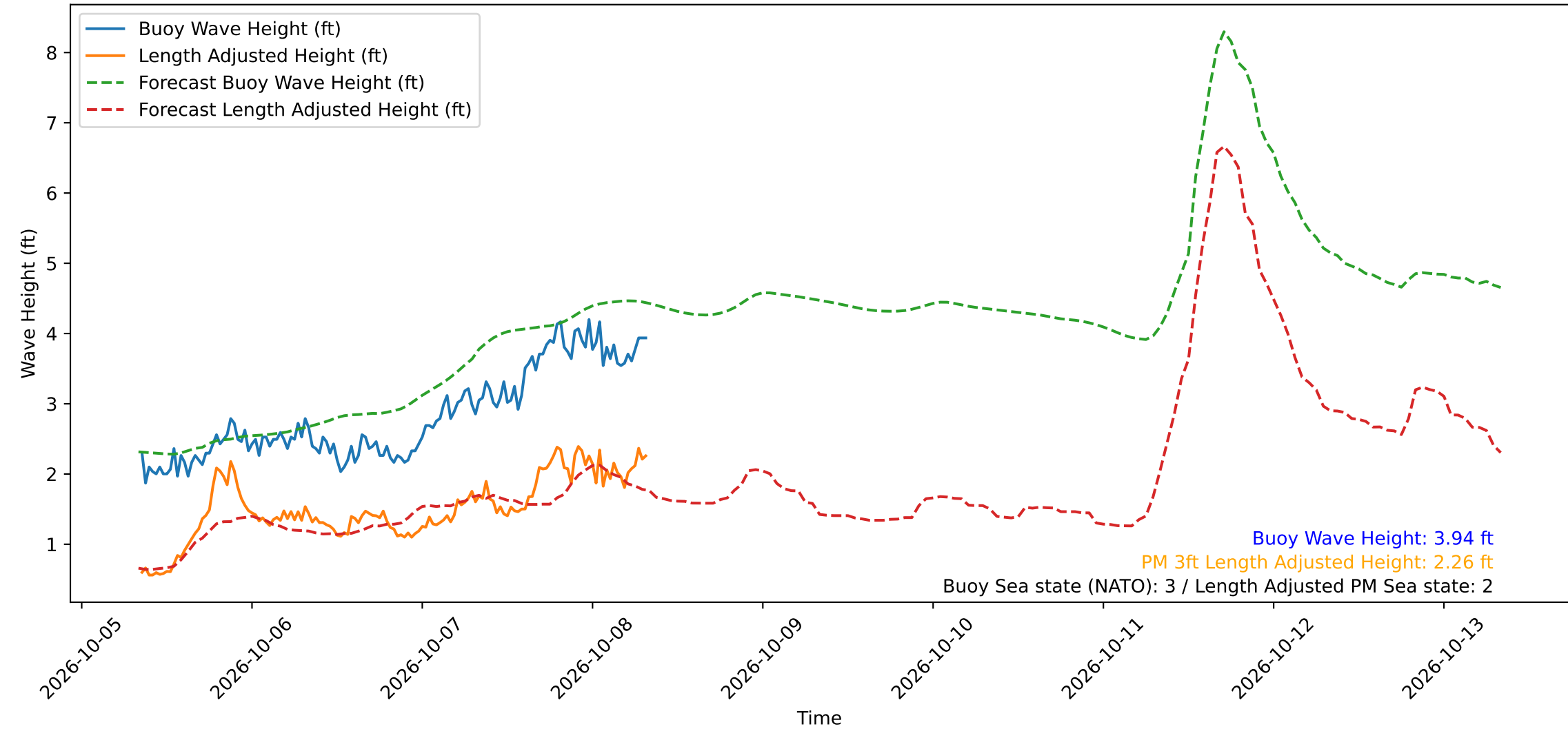
Wave Heights over Time for Oceanside Harbor at 2026-10-08 08:20:29
