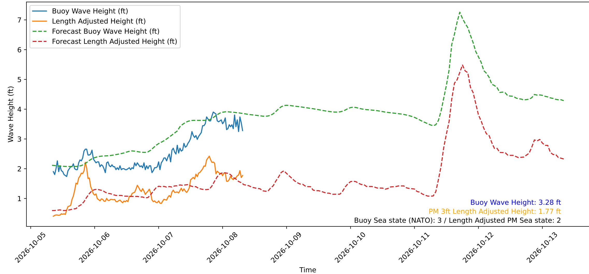
Wave Heights over Time for Red Beach at 2026-10-08 08:20:50
