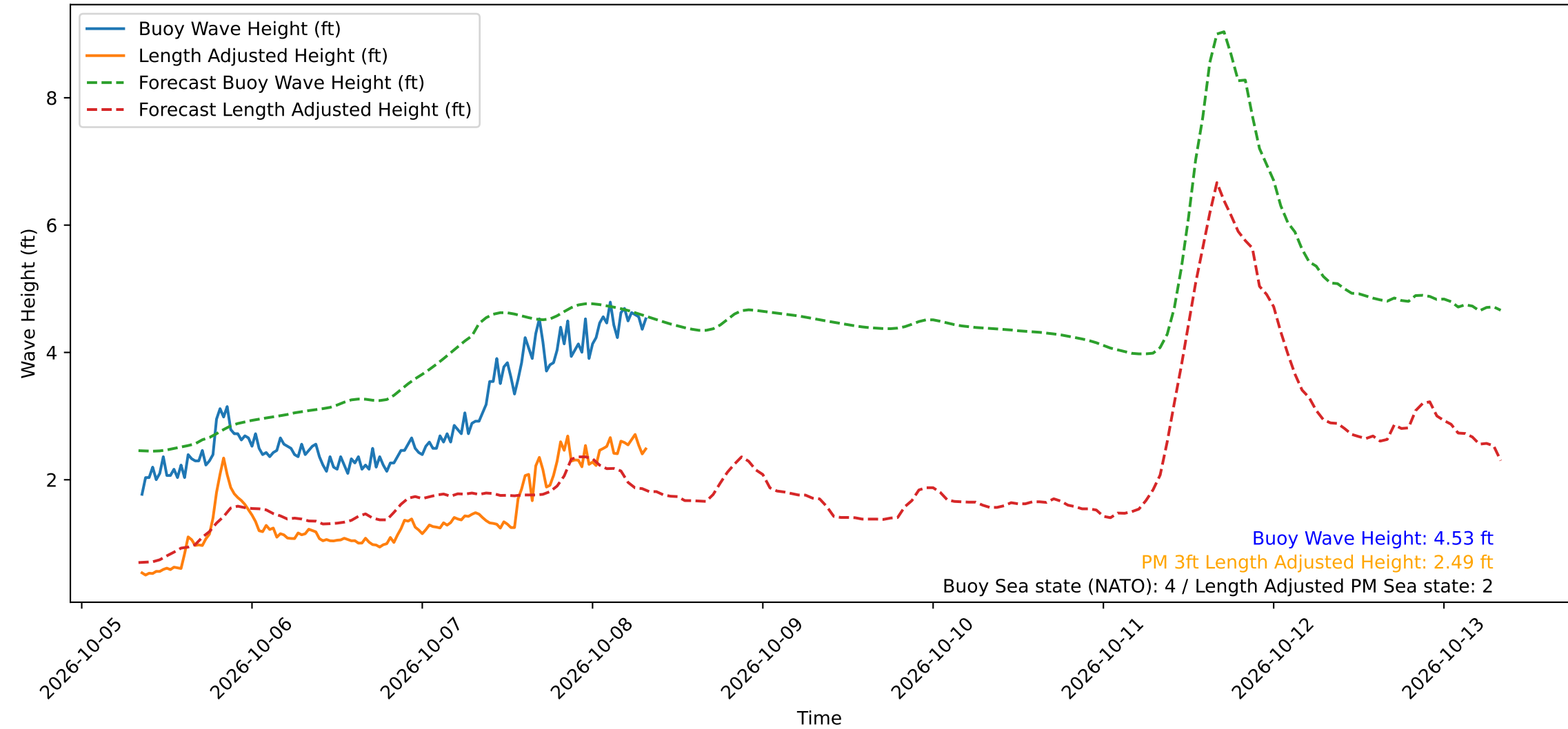
Wave Heights over Time for Green Beach at 2026-10-08 08:21:14
