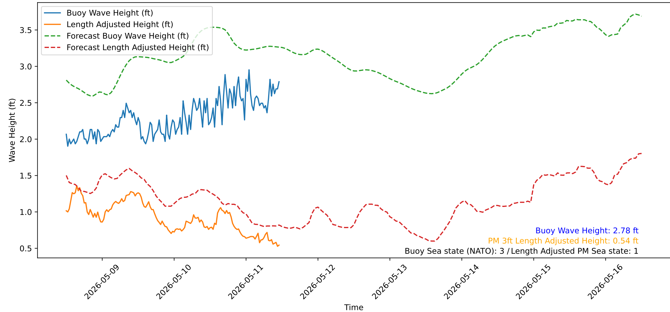
Wave Heights over Time for Red Beach at 2026-05-11 11:50:51
