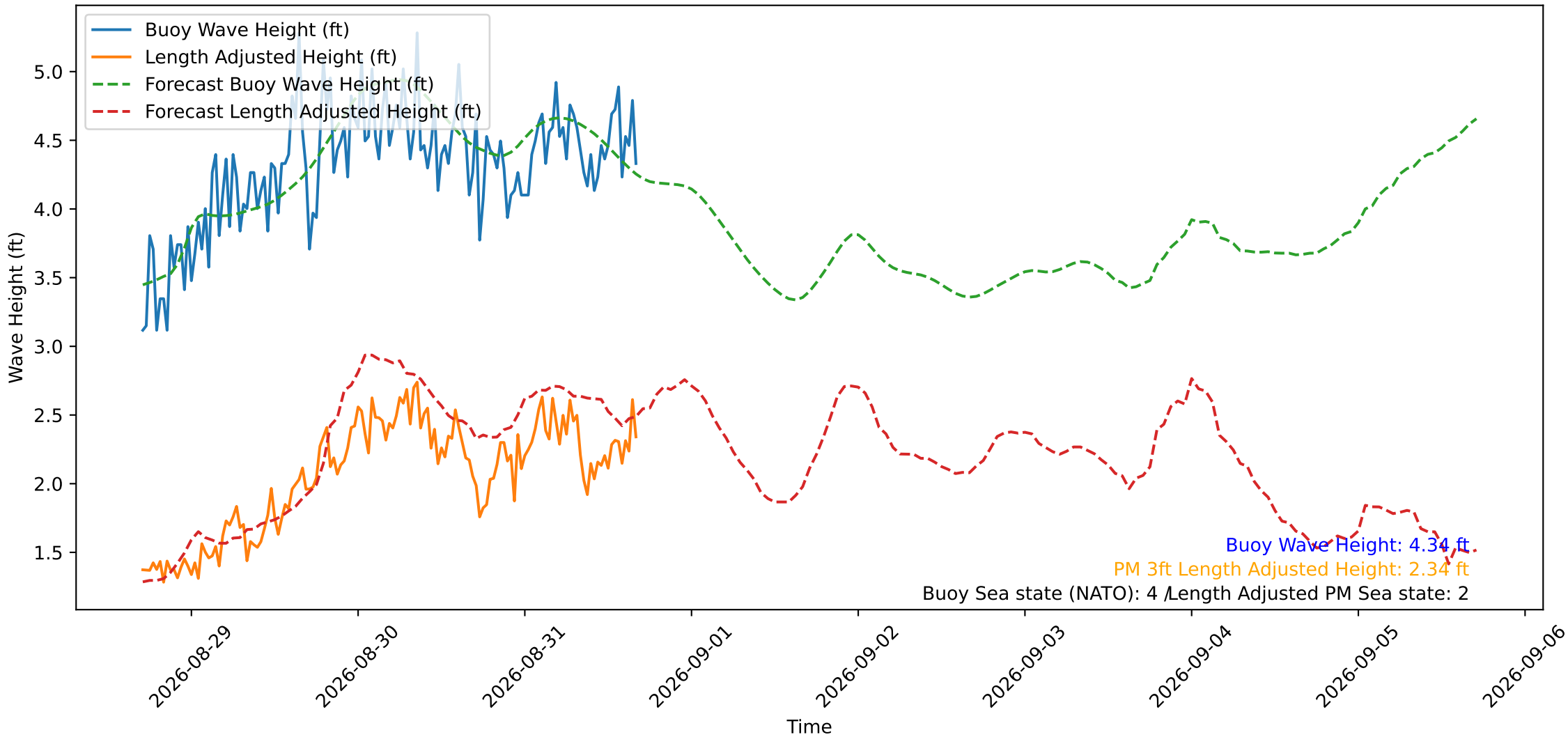
Wave Heights over Time for Oceanside Harbor at 2026-08-31 16:50:29
