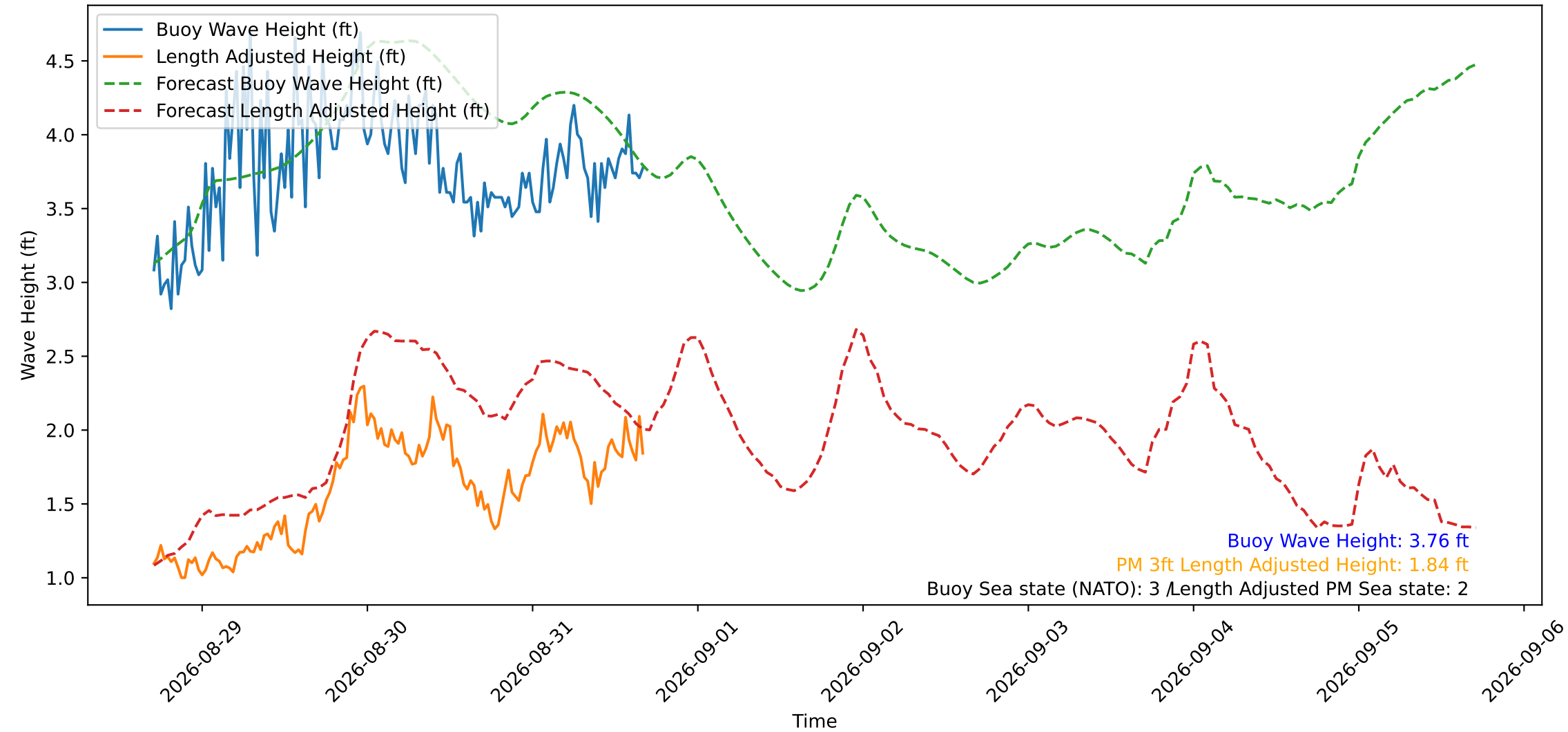
Wave Heights over Time for Red Beach at 2026-08-31 16:50:50
