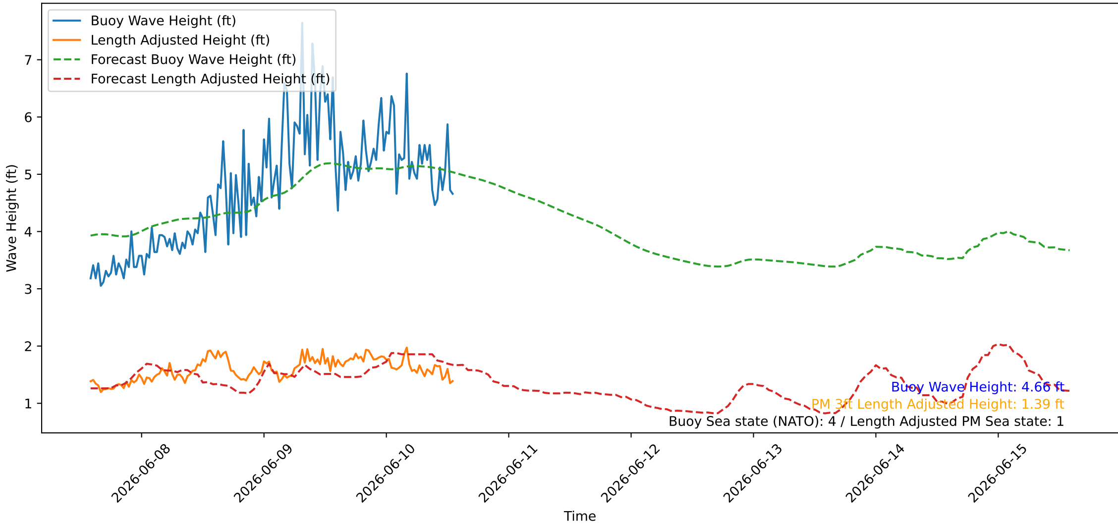
Wave Heights over Time for Red Beach at 2026-06-10 13:50:46
