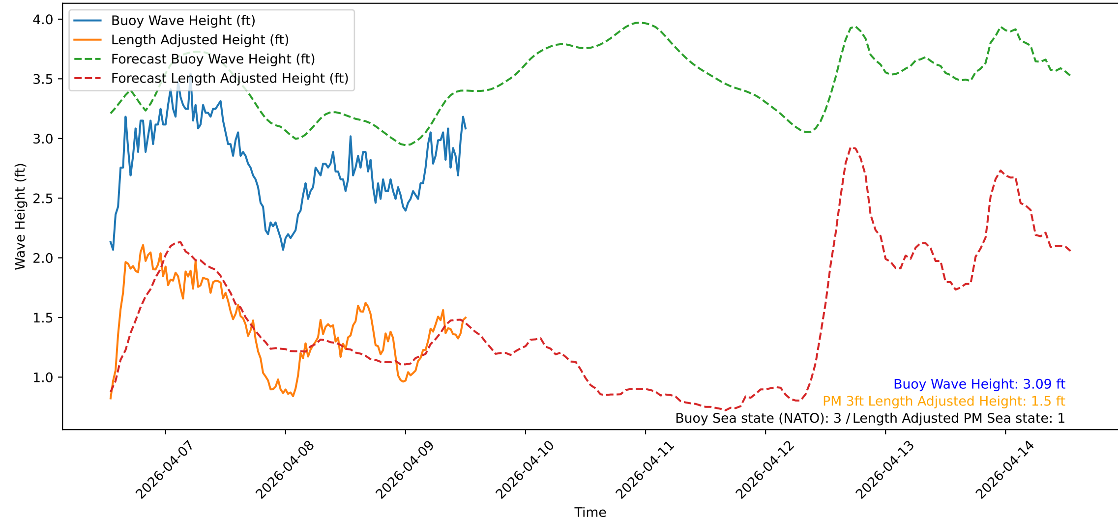
Wave Heights over Time for Red Beach at 2026-04-09 12:40:47
