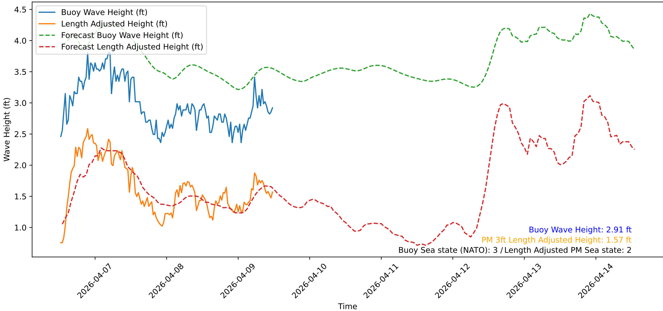
Wave Heights over Time for Green Beach at 2026-04-09 12:41:10
