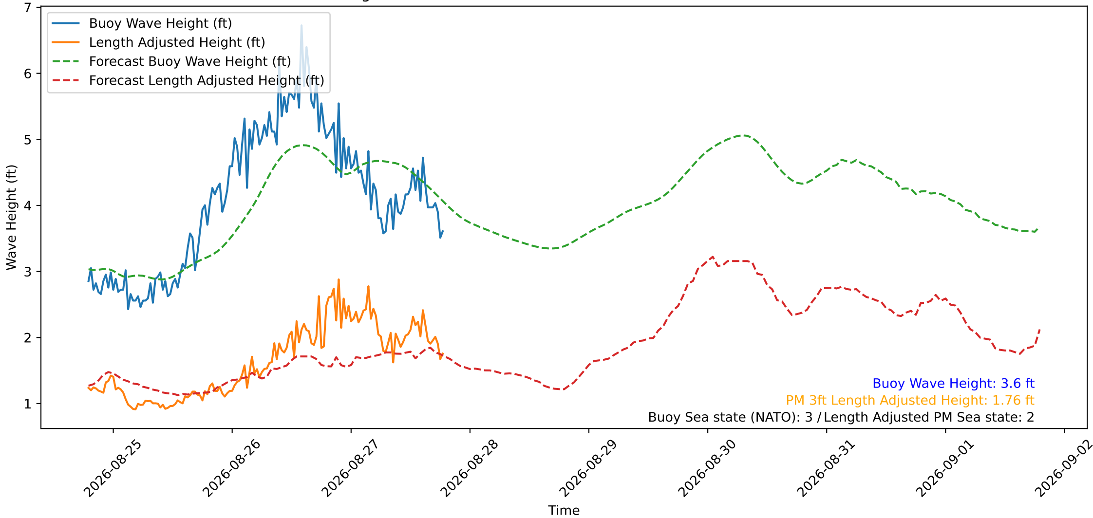
Wave Heights over Time for Oceanside Harbor at 2026-08-27 19:00:30
