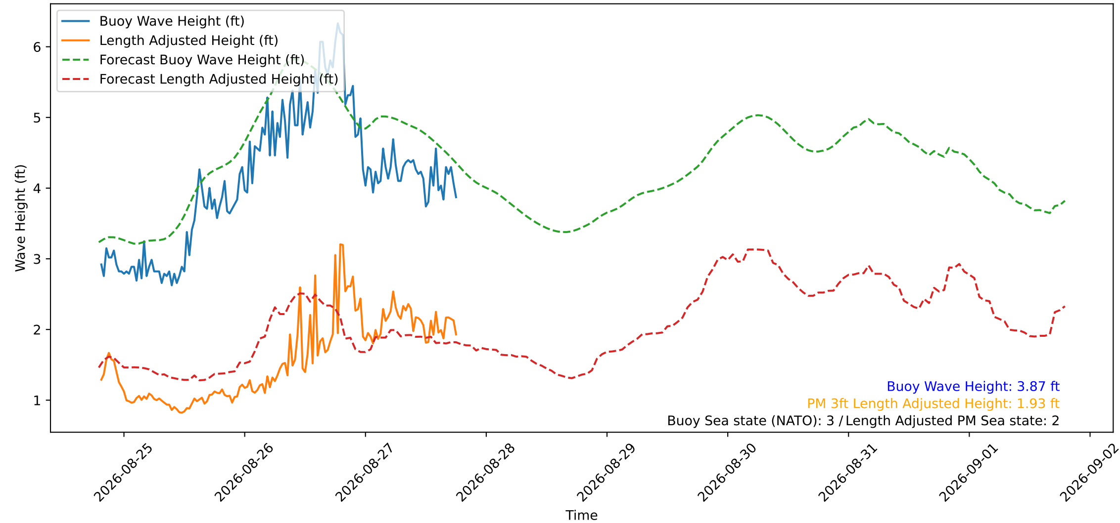
Wave Heights over Time for Green Beach at 2026-08-27 19:01:11
