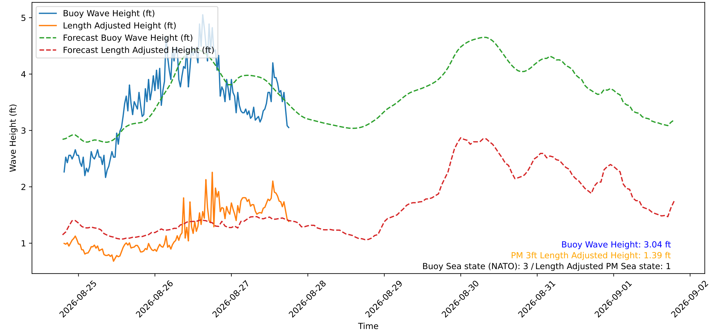
Wave Heights over Time for Red Beach at 2026-08-27 19:00:49
