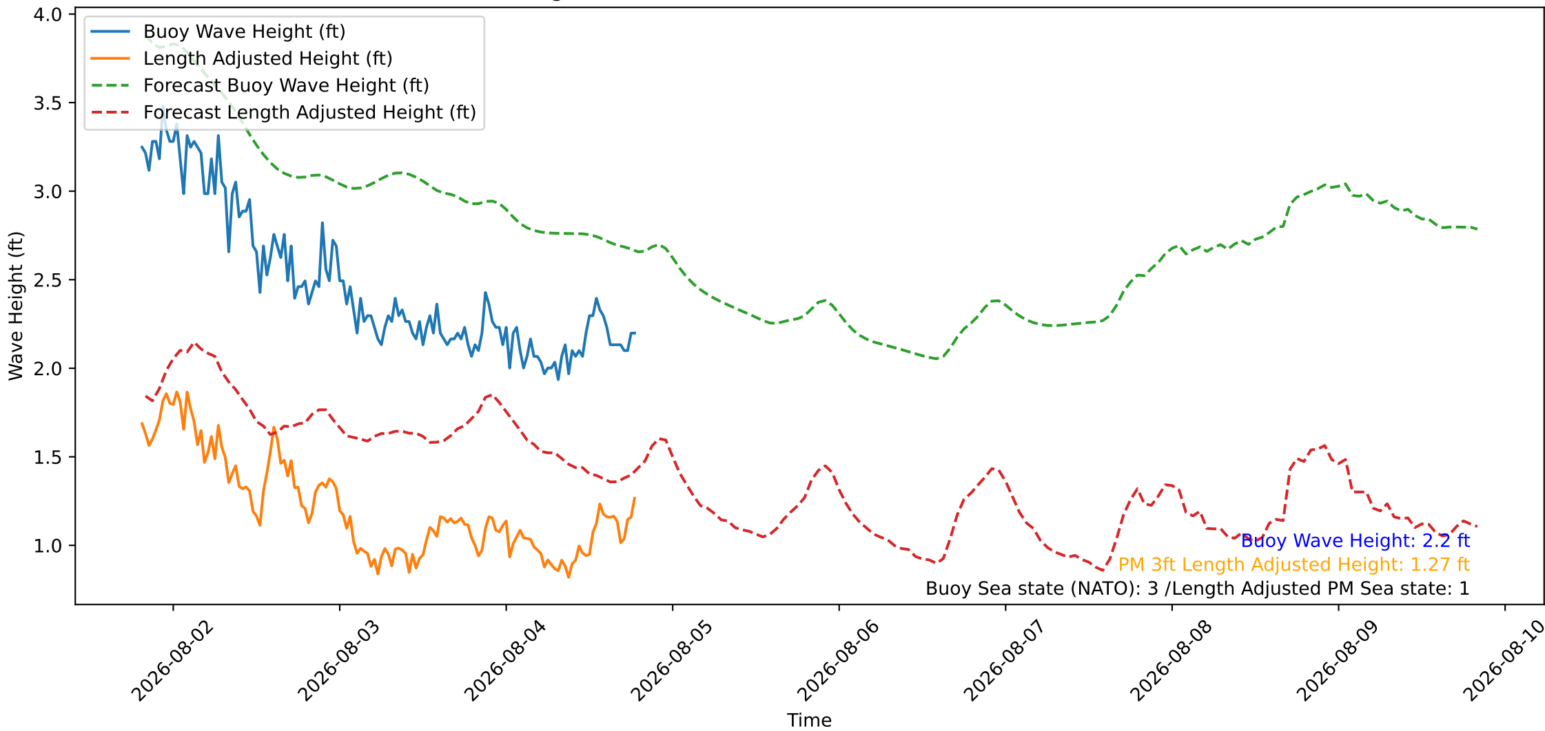
Wave Heights over Time for Green Beach at 2026-08-04 19:31:09
