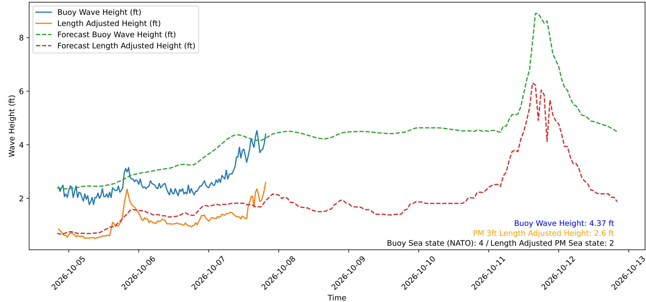
Wave Heights over Time for Green Beach at 2026-10-07 20:21:14
