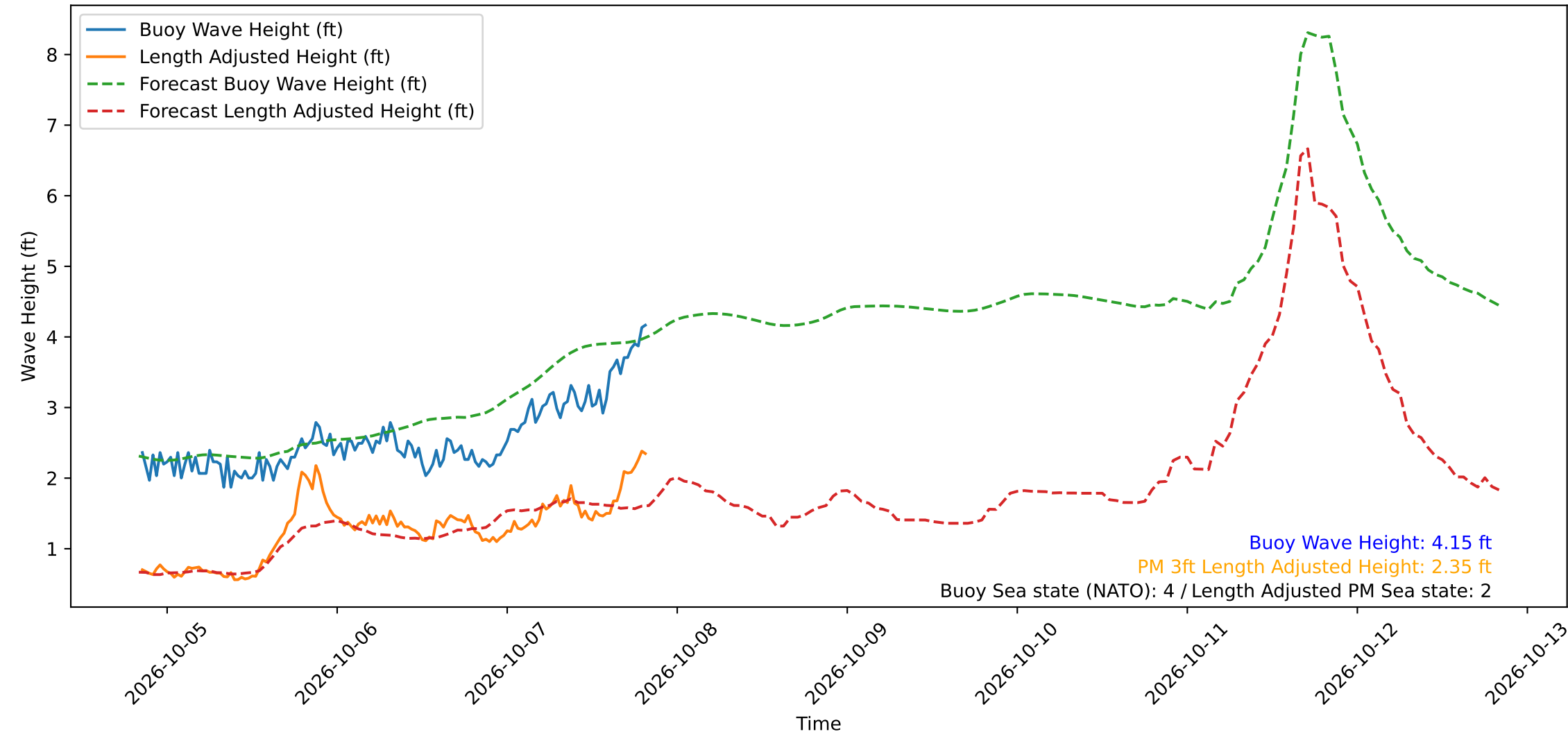
Wave Heights over Time for Oceanside Harbor at 2026-10-07 20:20:29
