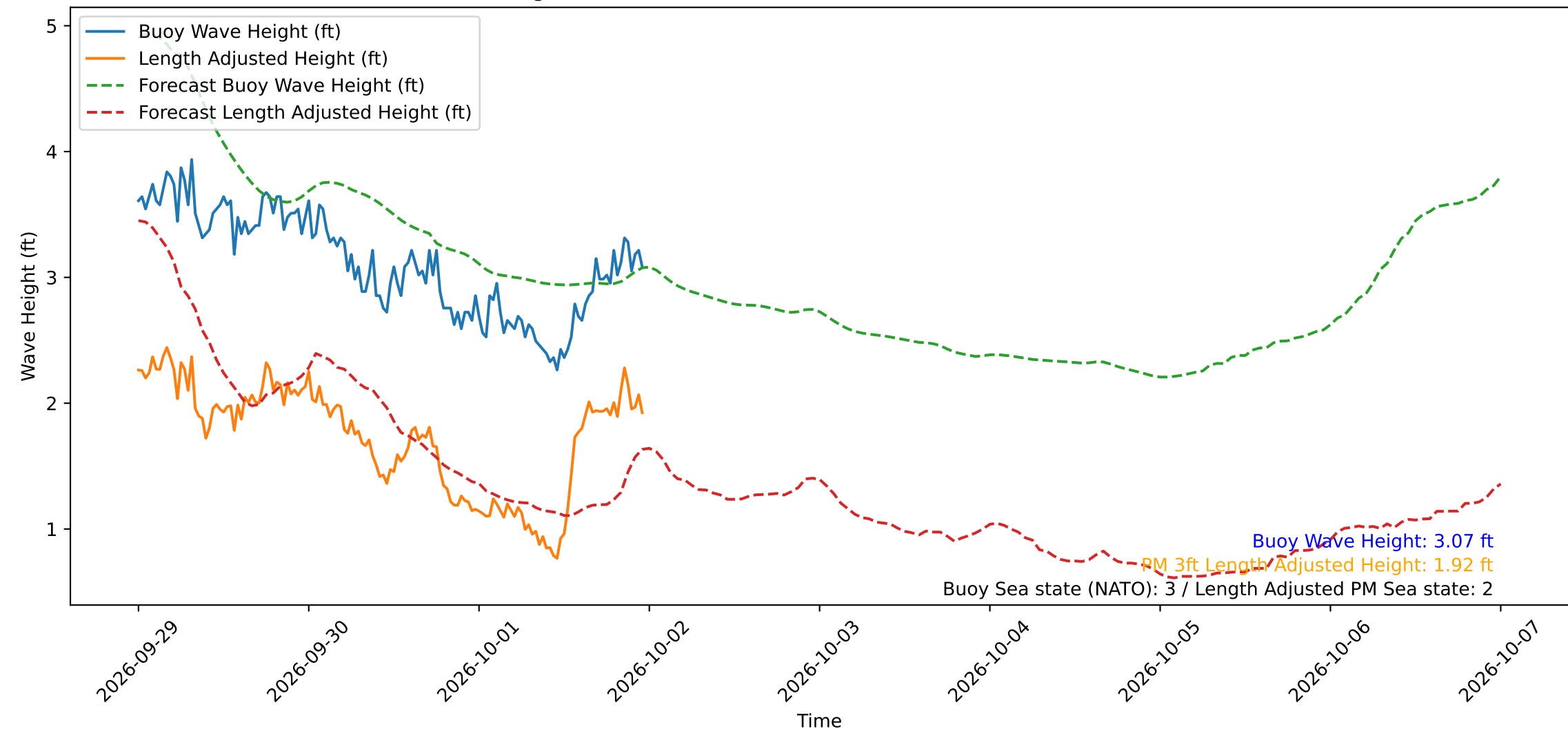
Wave Heights over Time for Oceanside Harbor at 2026-10-01 23:50:30
