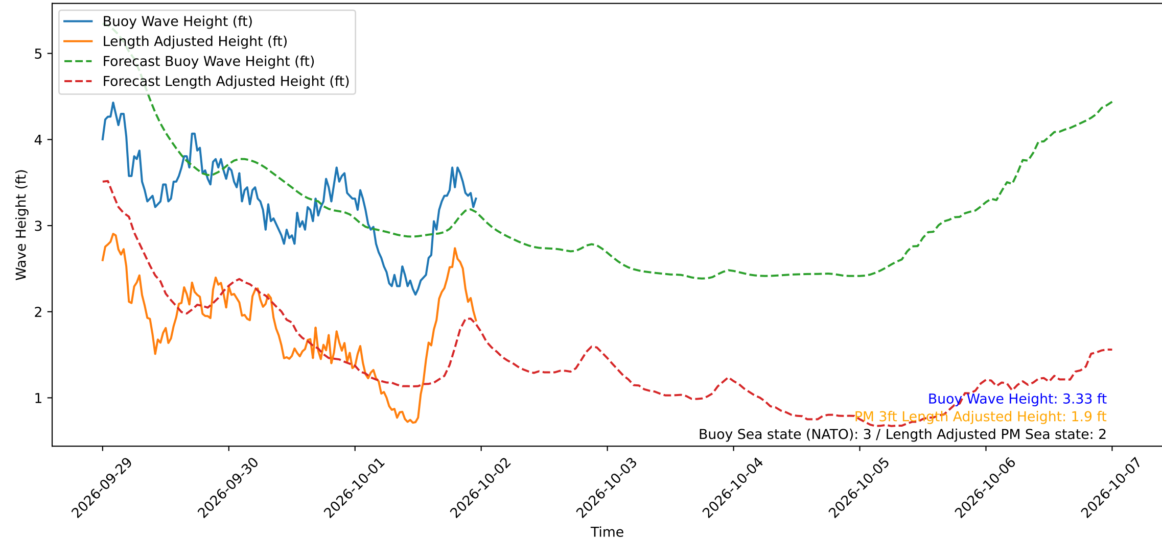
Wave Heights over Time for Green Beach at 2026-10-01 23:51:14
