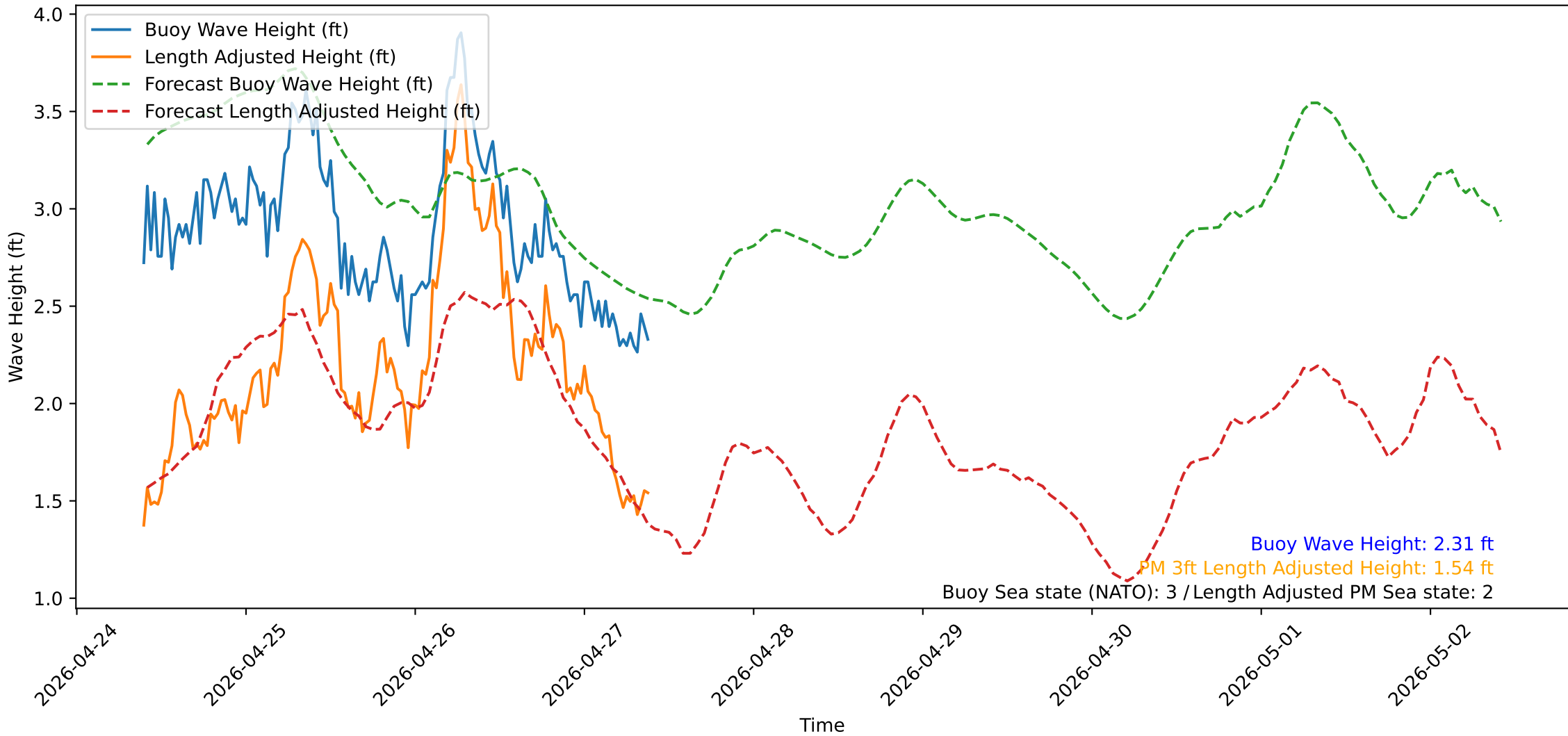
Wave Heights over Time for Oceanside Harbor at 2026-04-27 09:40:31
