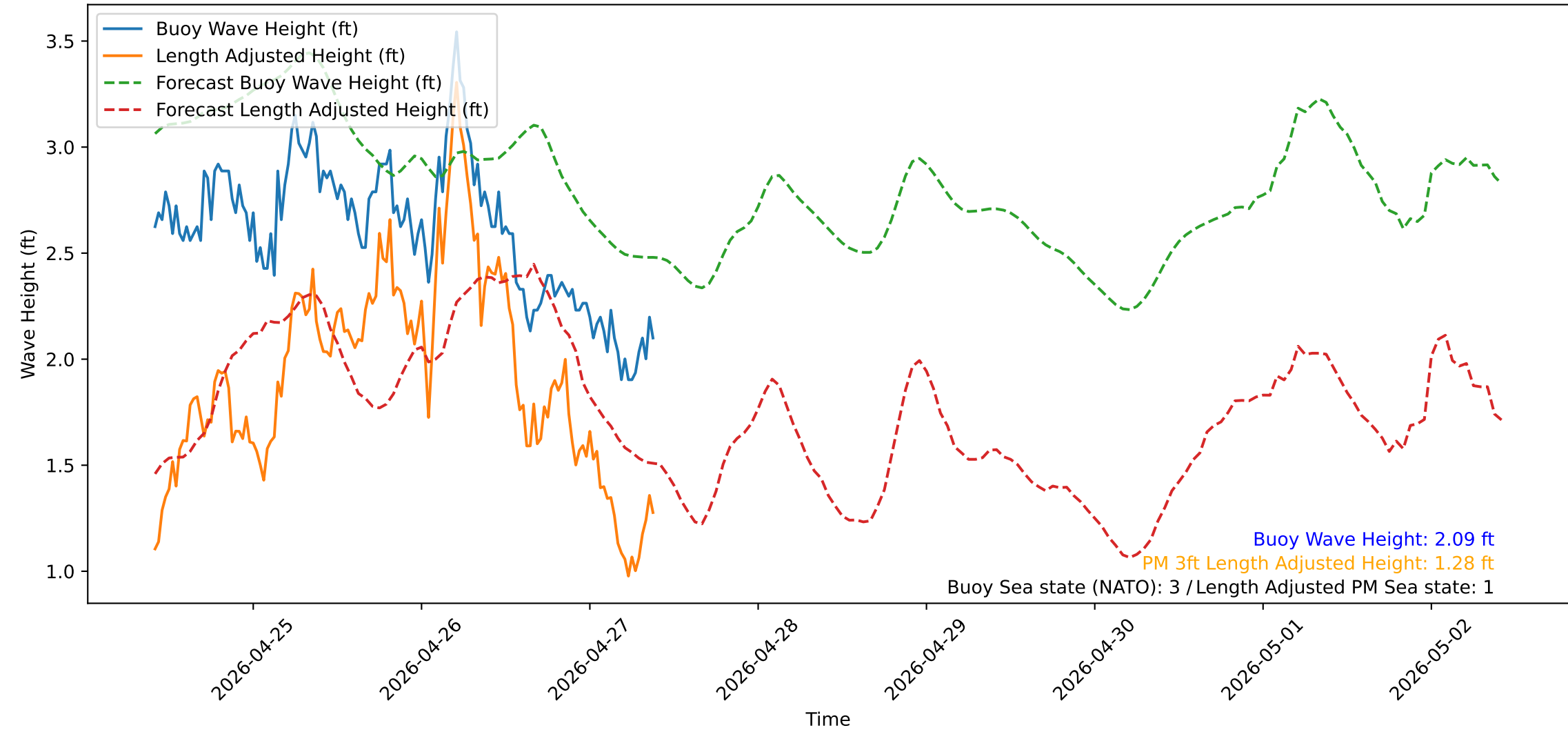
Wave Heights over Time for Red Beach at 2026-04-27 09:40:50
