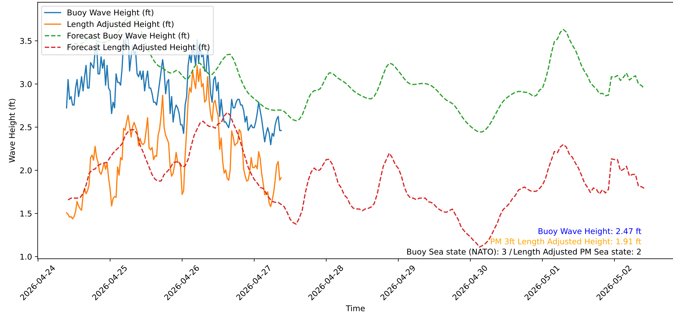
Wave Heights over Time for Green Beach at 2026-04-27 09:41:13
